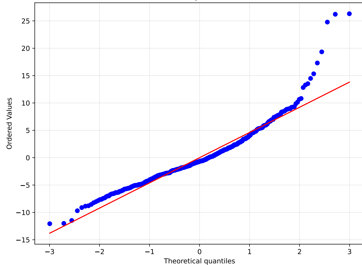
Q-Q Plot: Normality Check of Residuals
