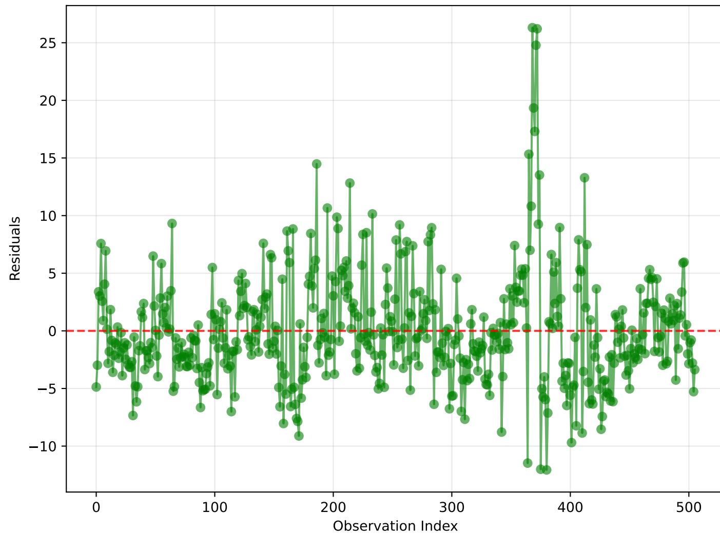
Residuals Order Plot
