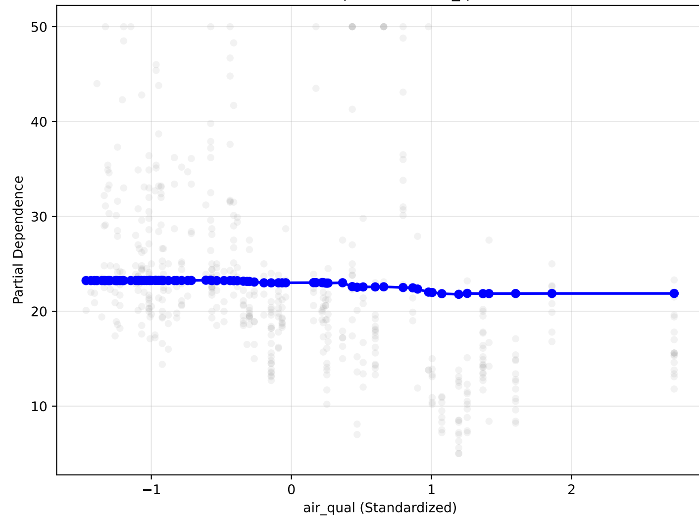
Partial Dependence: air_qual
