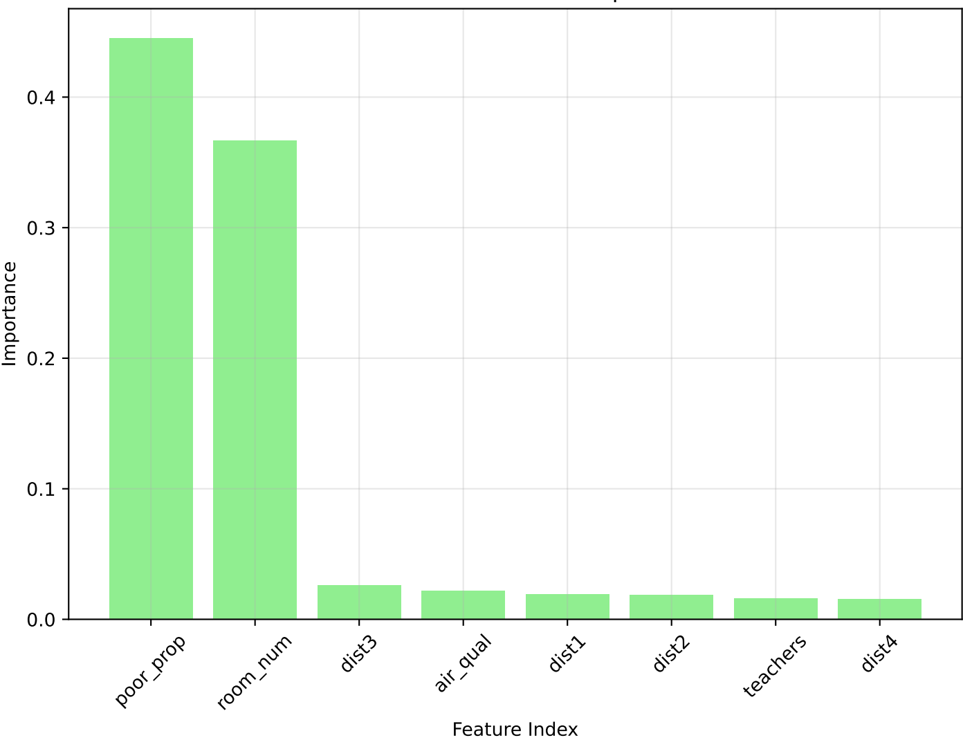
Random Forest Feature Importance
