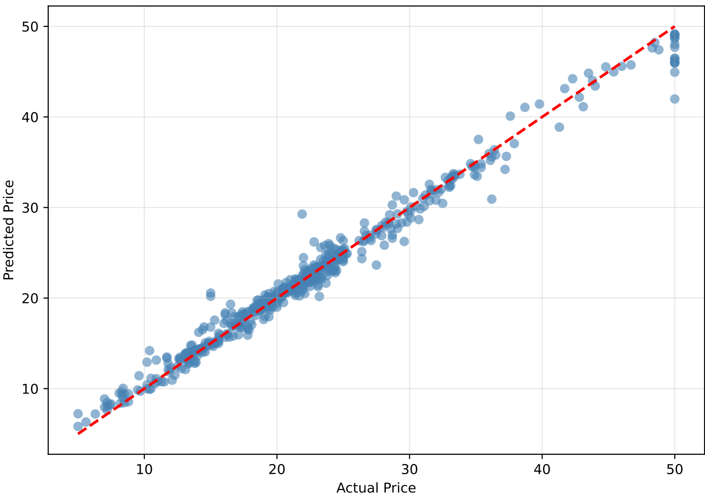
Best Model: Random Forest ( R^2 = 0.982 )
