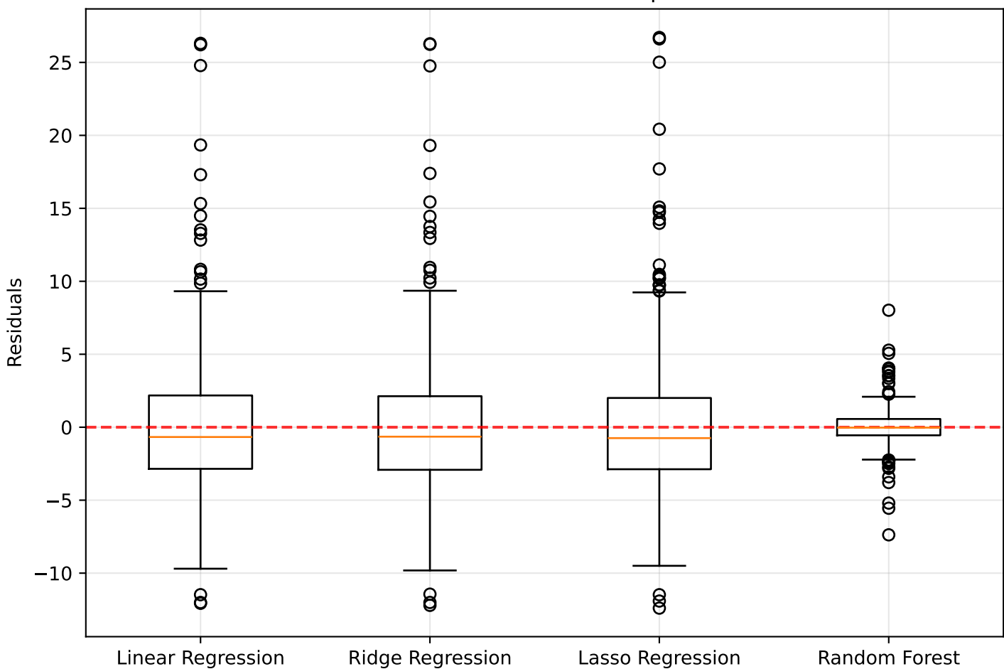
Residual Distribution Comparison
