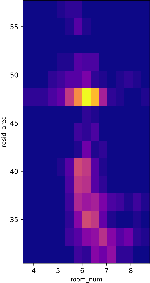
2D Density
