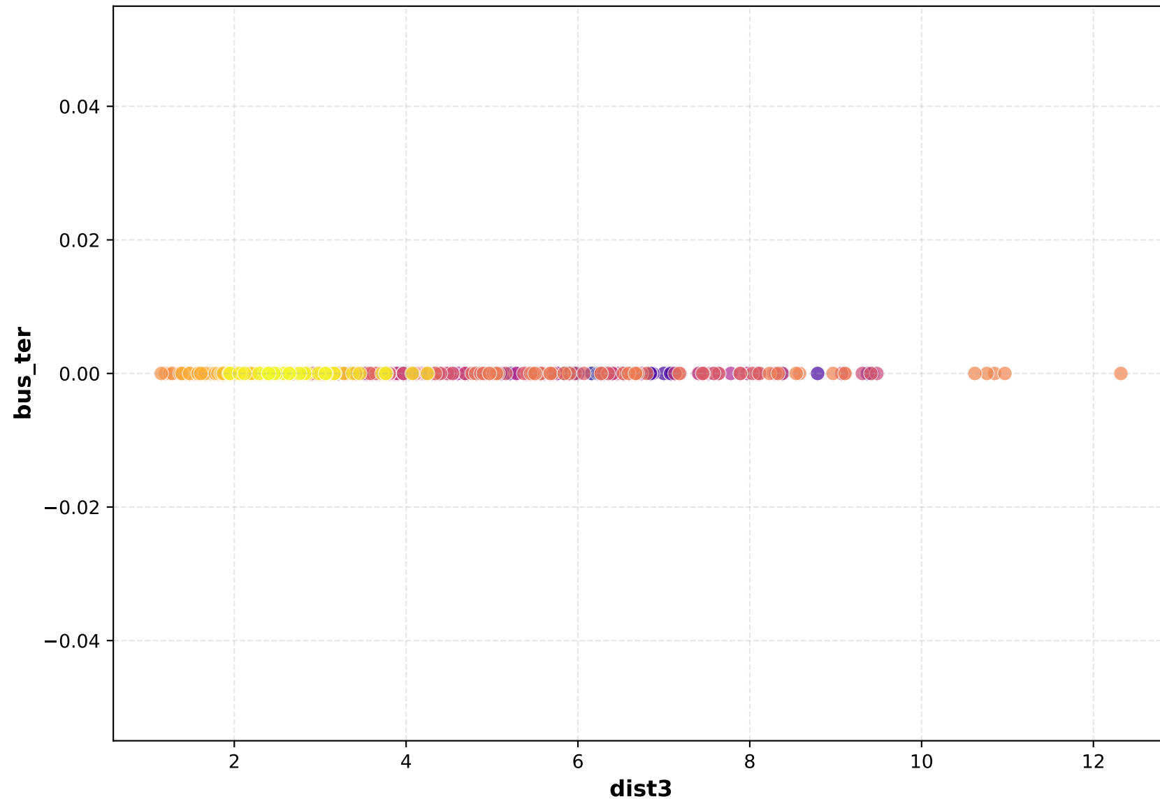
Scatter Plot
