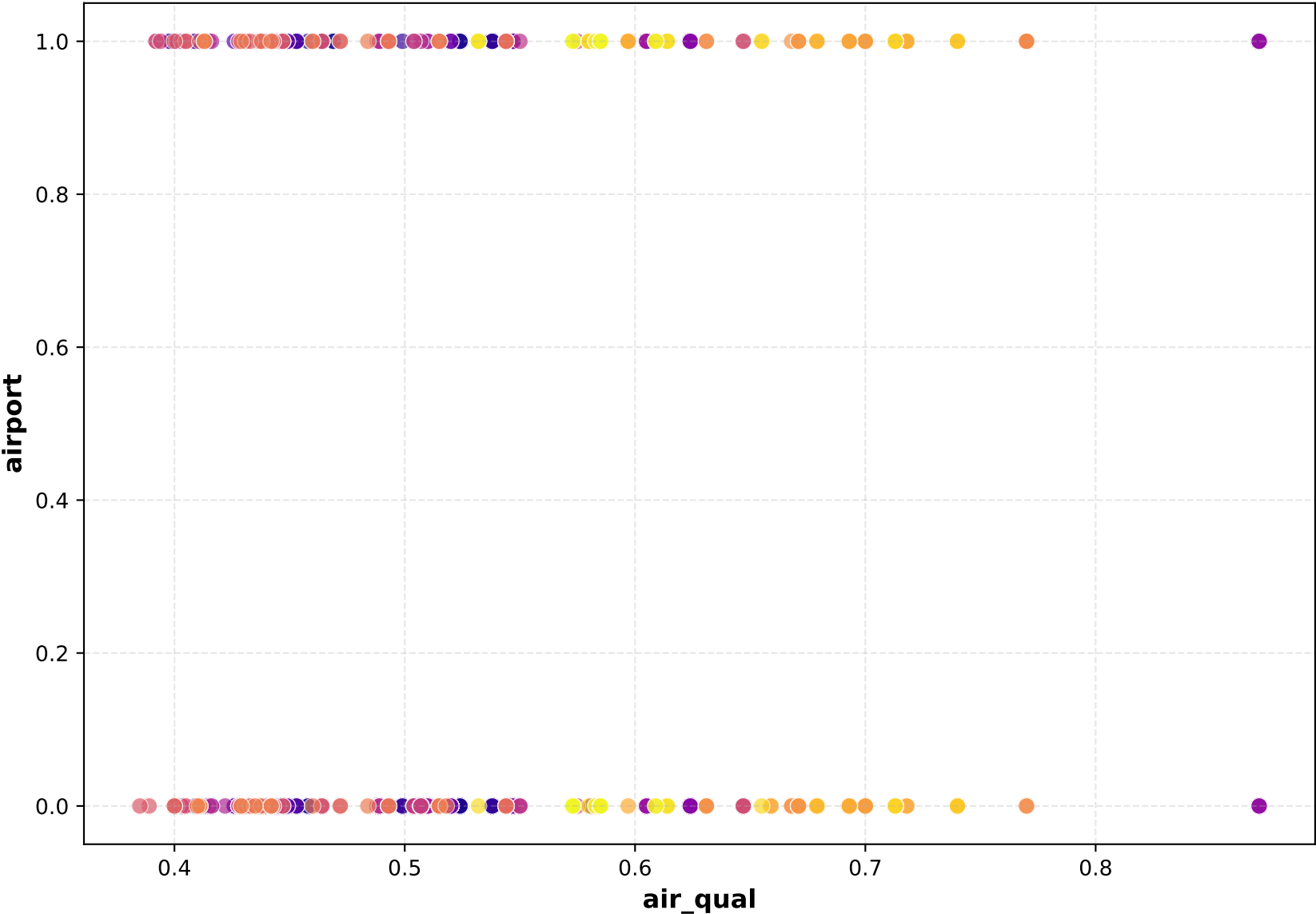
Scatter Plot
