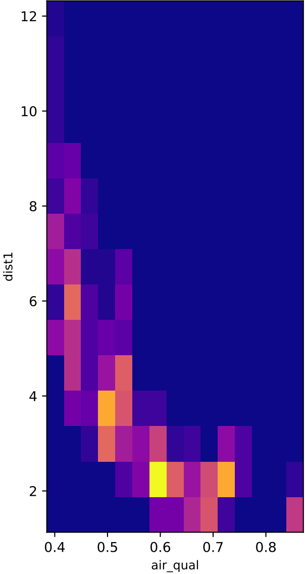
2D Density
