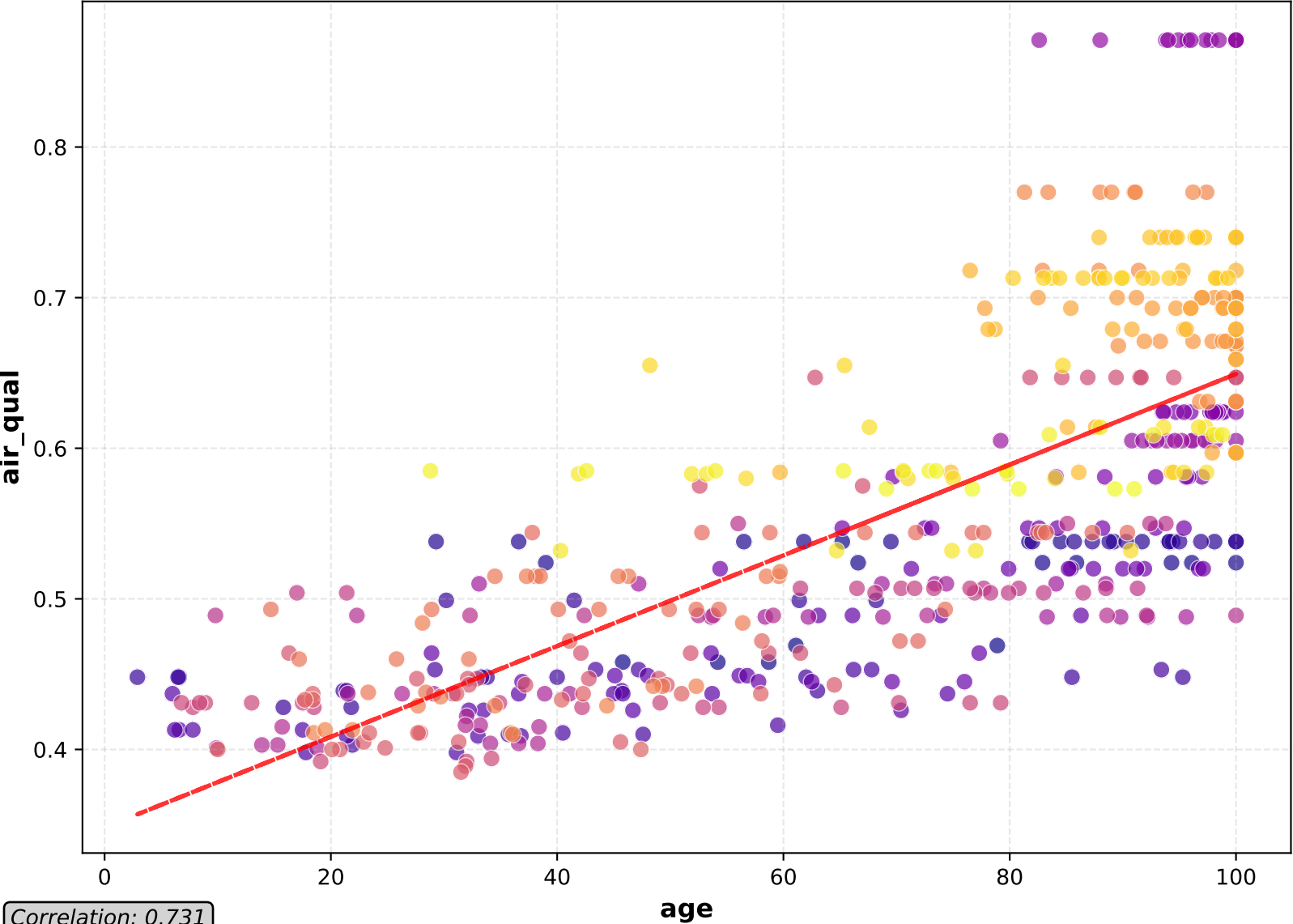
Scatter Plot
