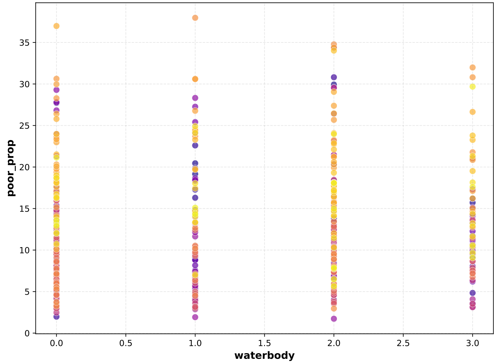
Scatter Plot
