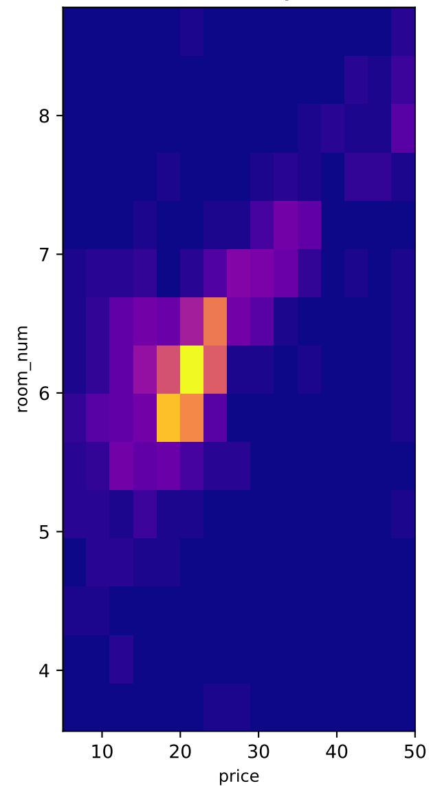
2D Density
