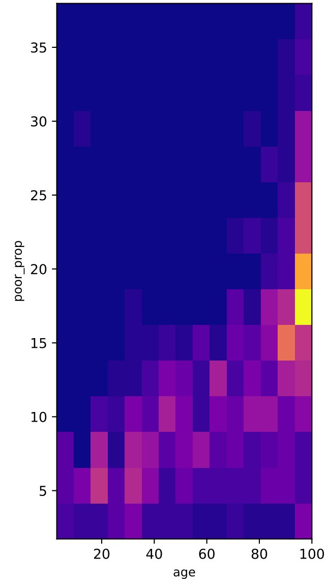
2D Density
