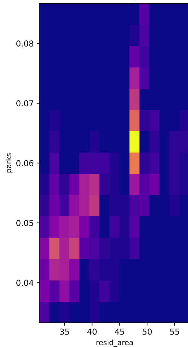
2D Density
