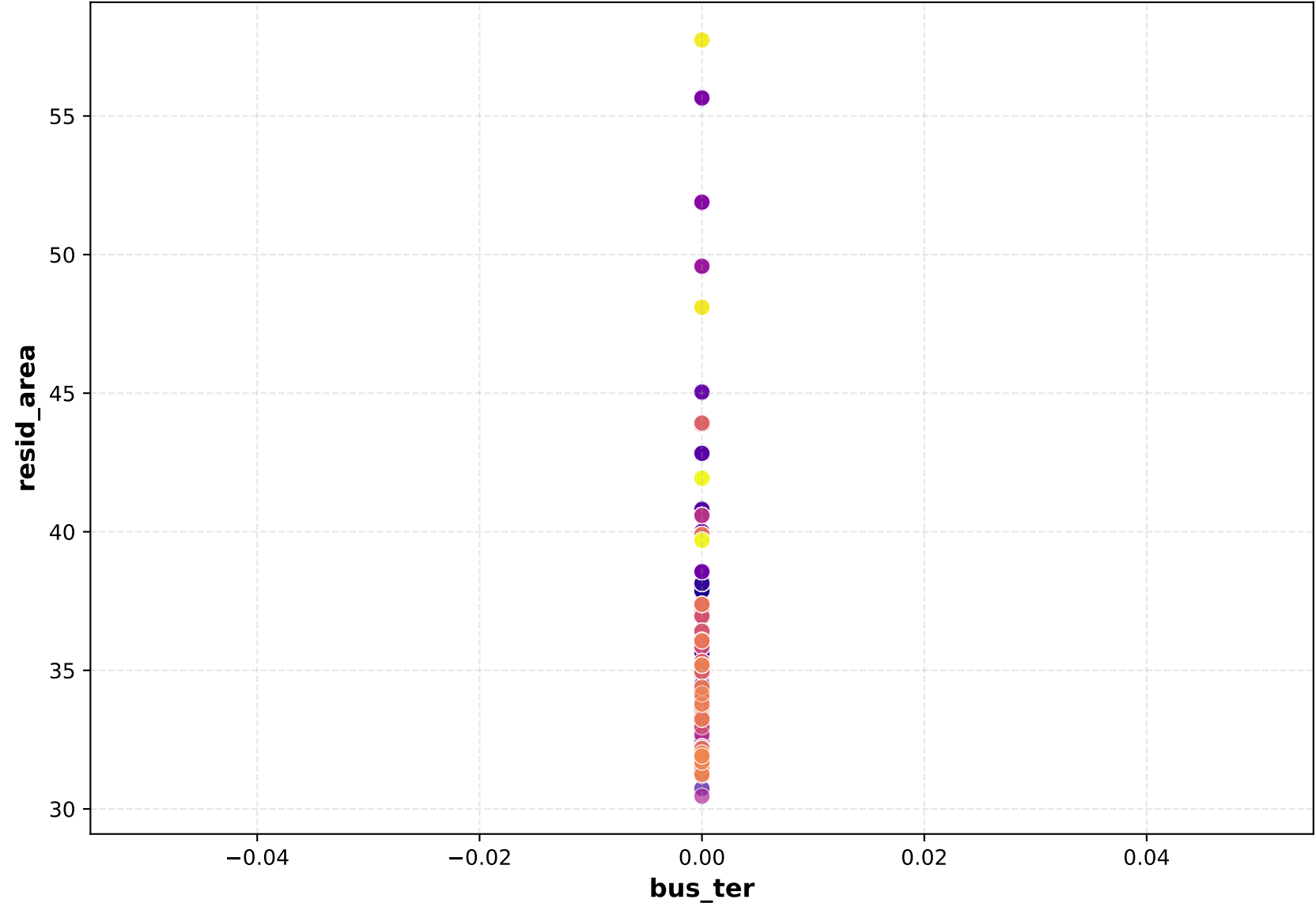
Scatter Plot
