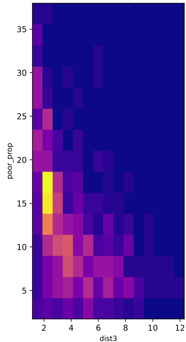
2D Density
