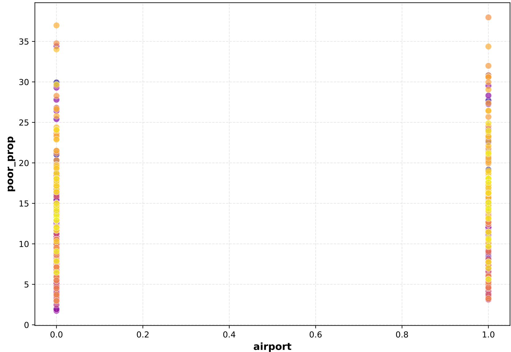
Scatter Plot
