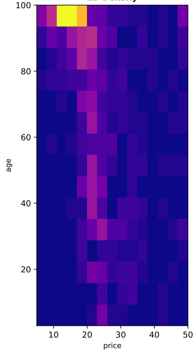
2D Density
