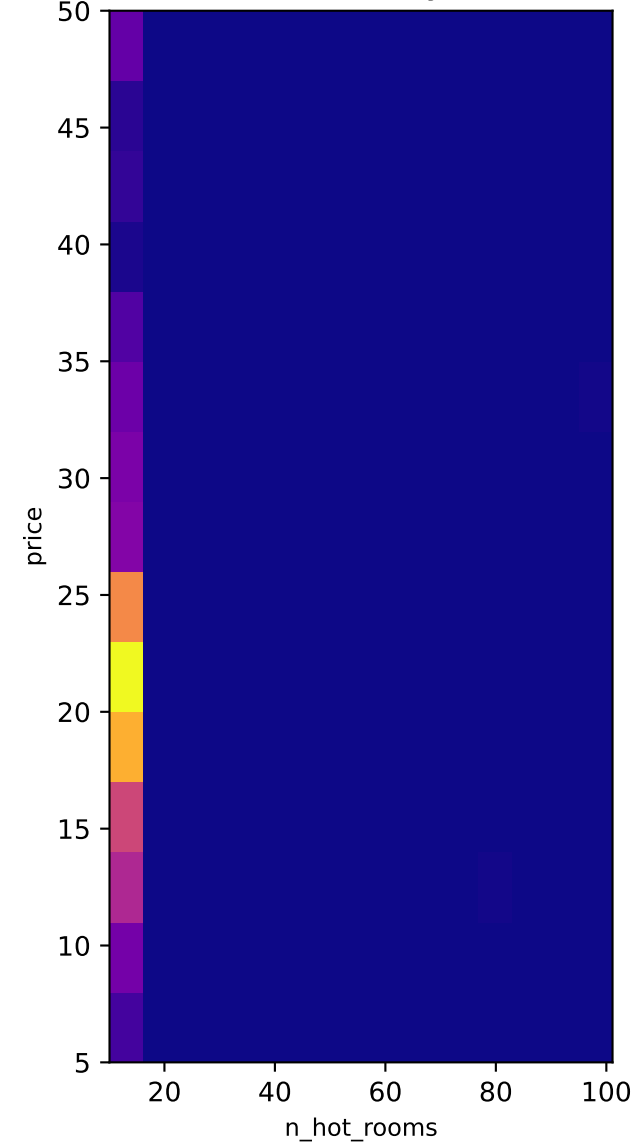
2D Density
