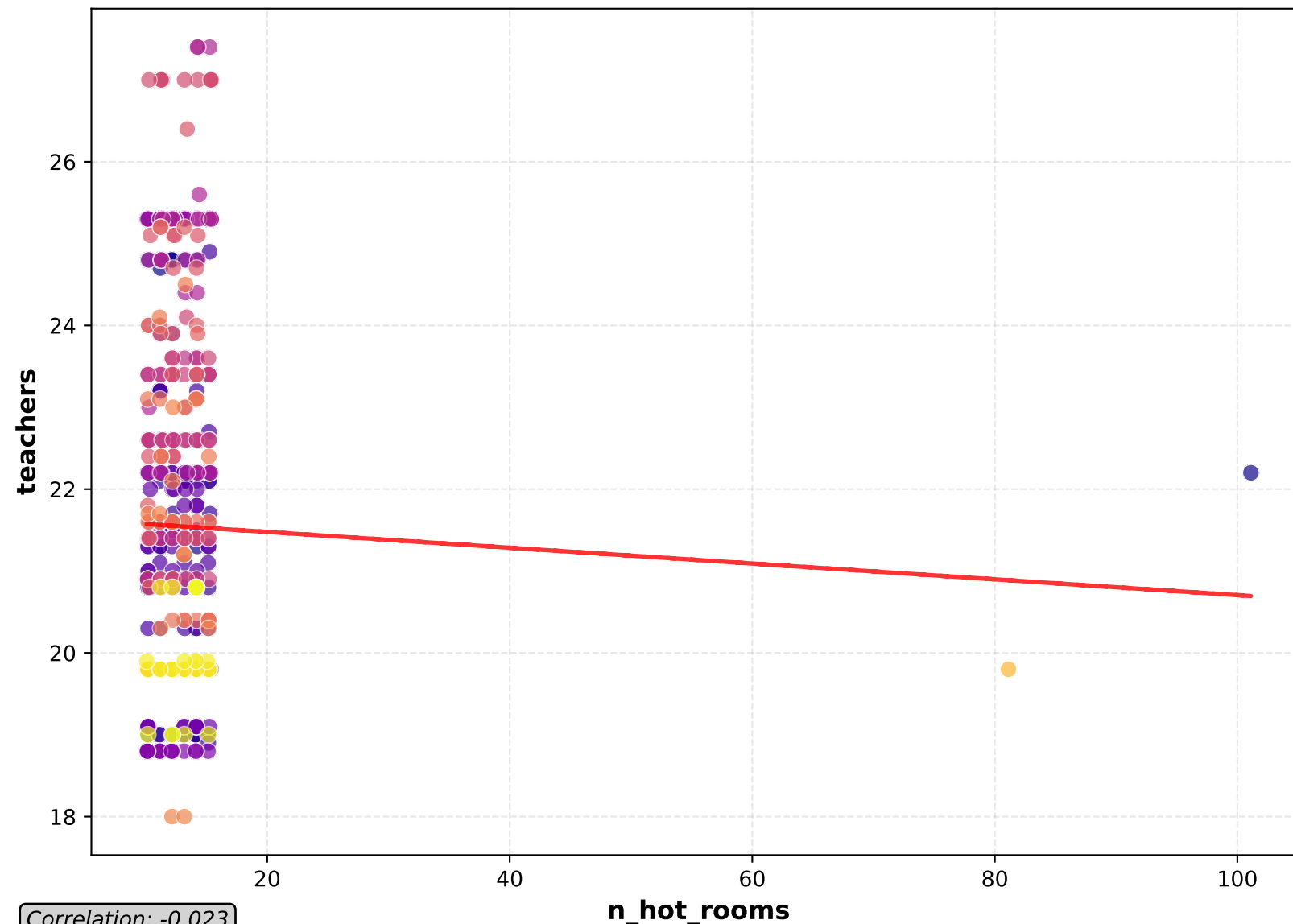
Scatter Plot
