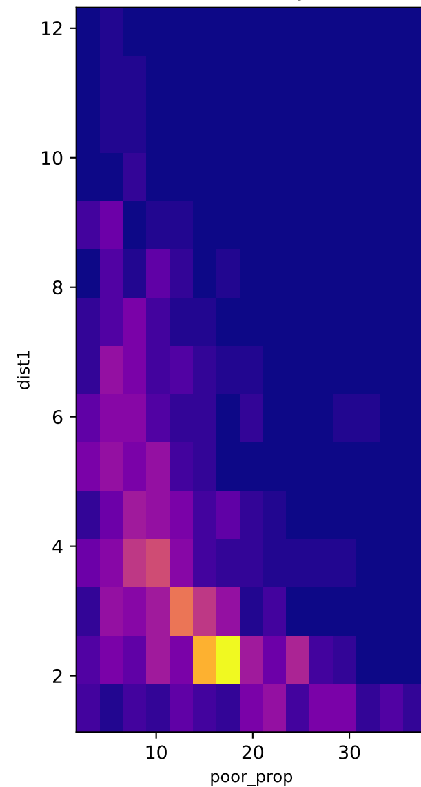
2D Density
