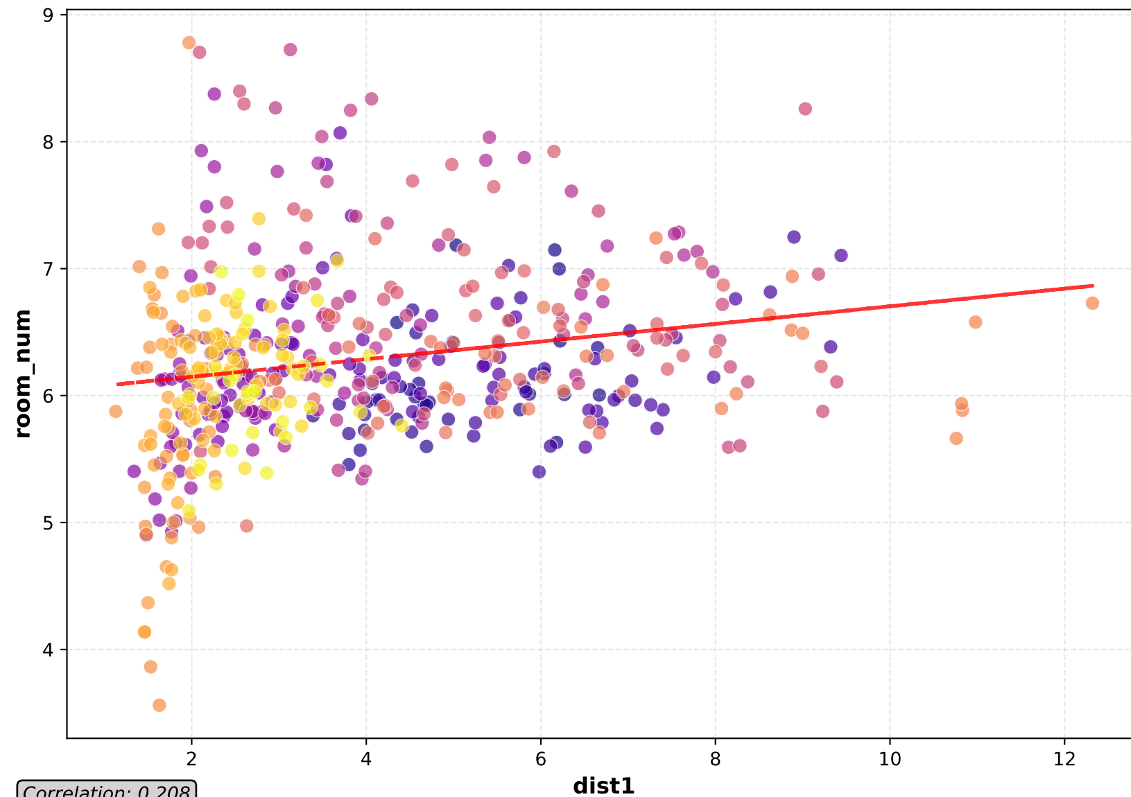
Scatter Plot
