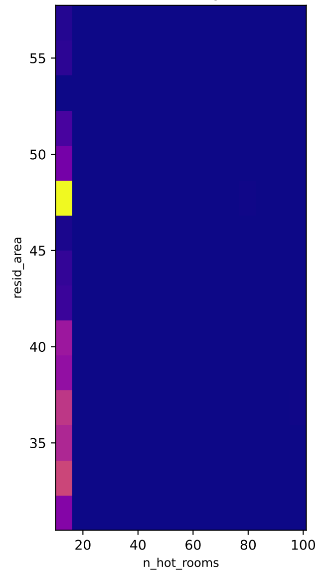
2D Density
