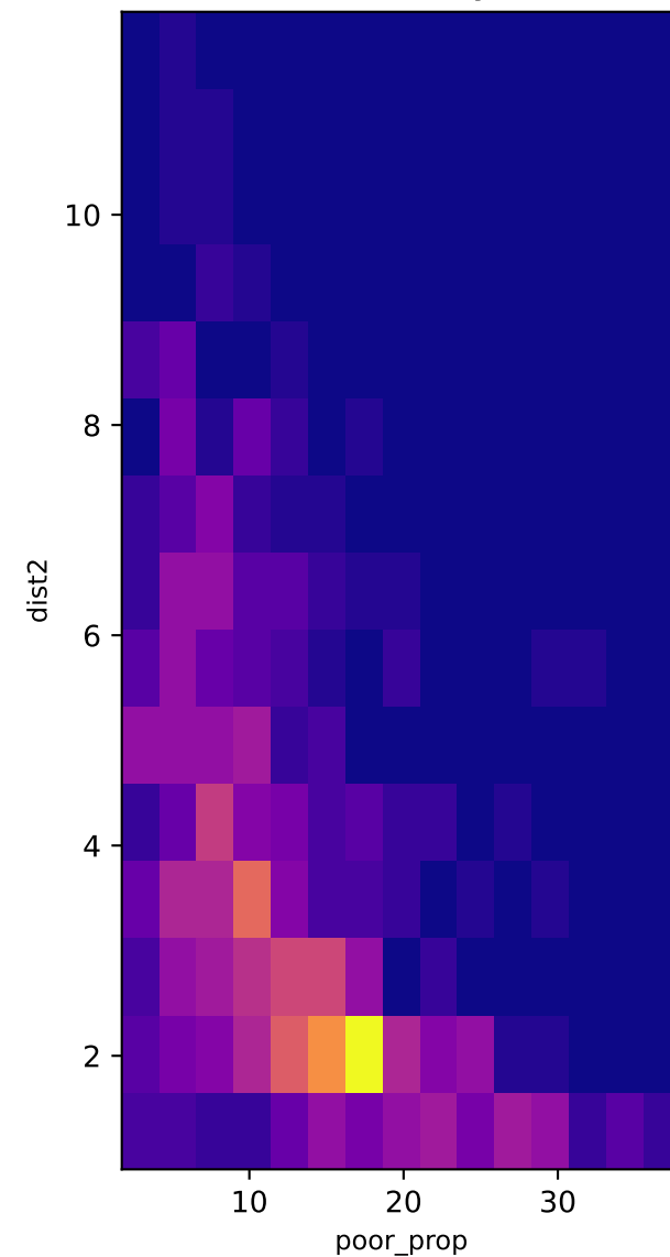
2D Density
