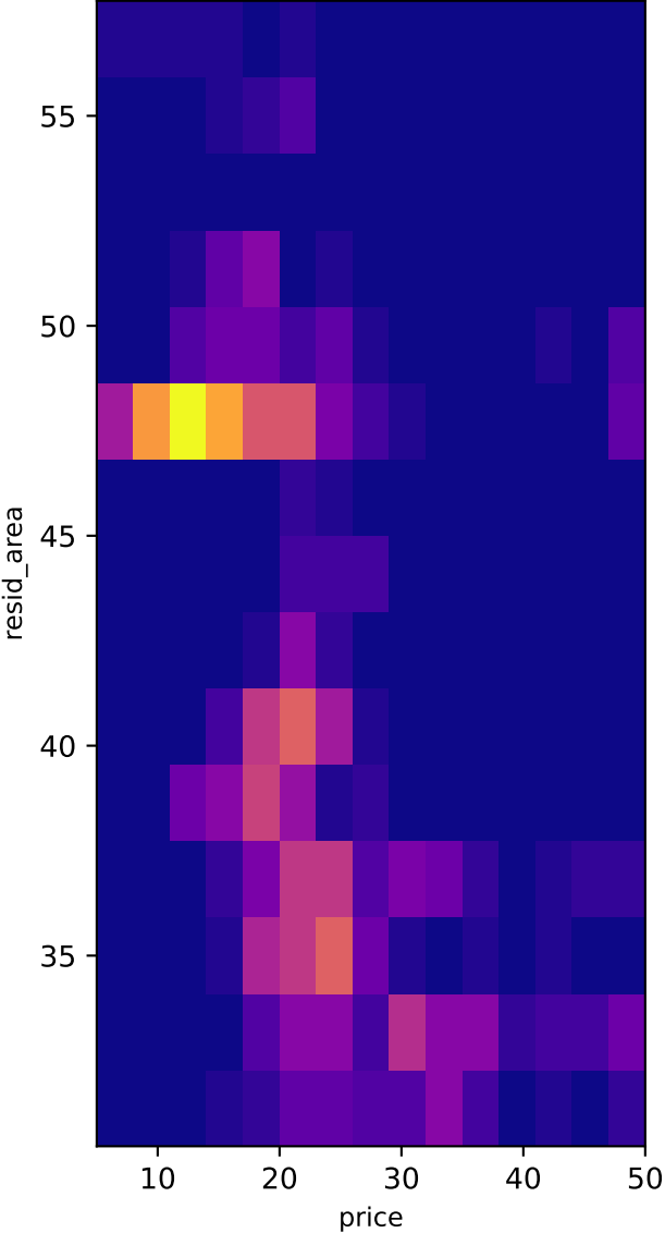
2D Density
