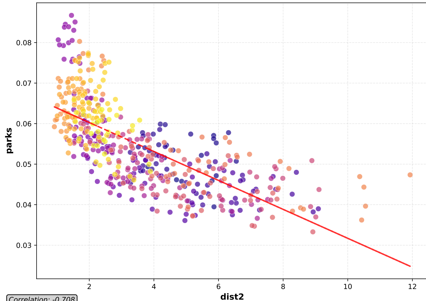
Scatter Plot
