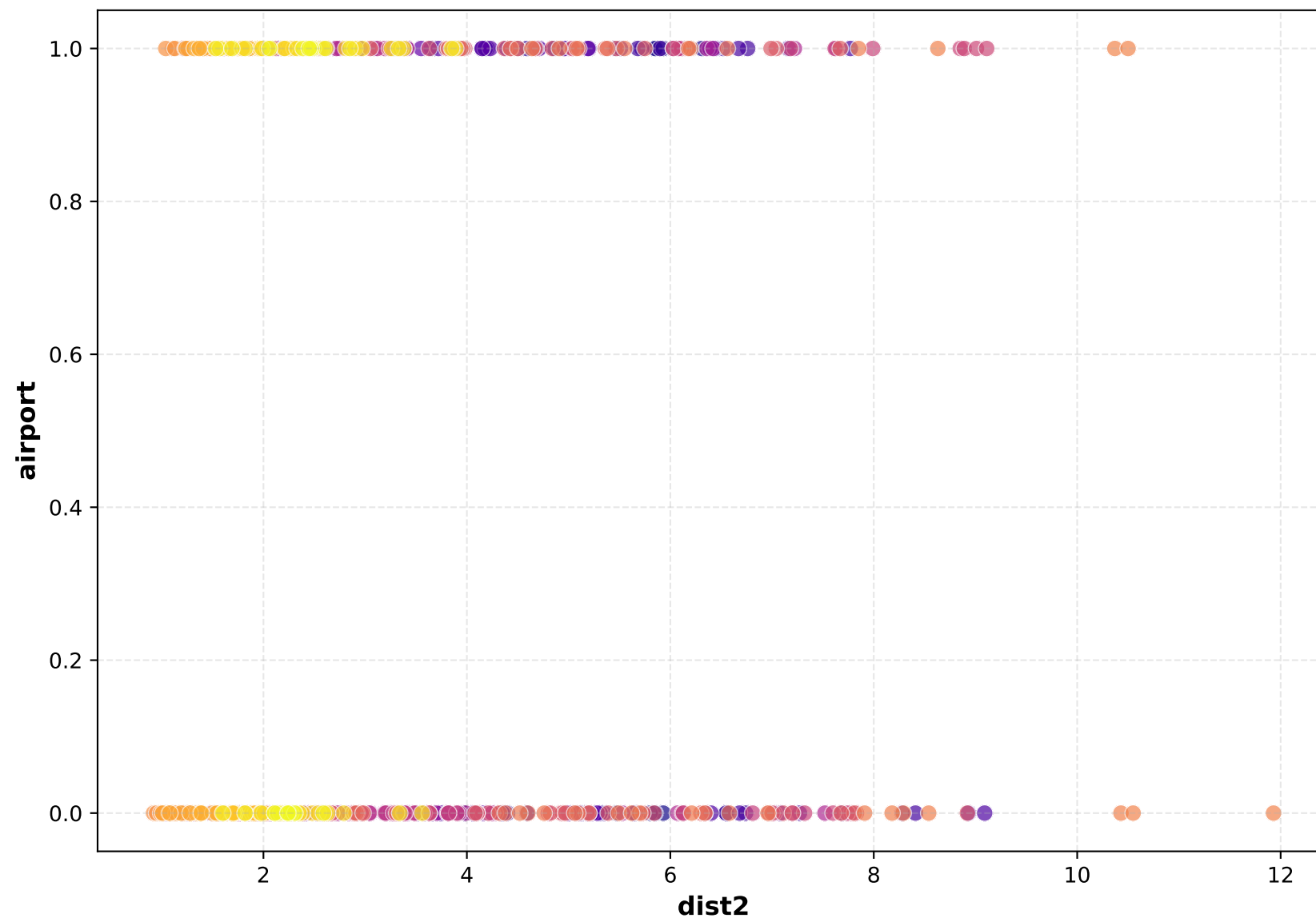
Scatter Plot
