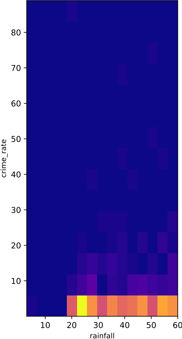
2D Density
