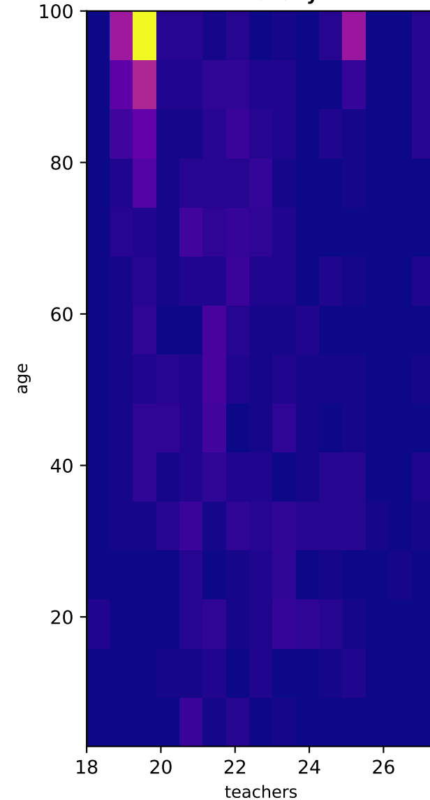
2D Density
