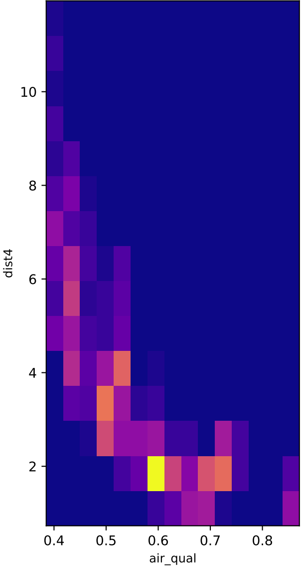
2D Density
