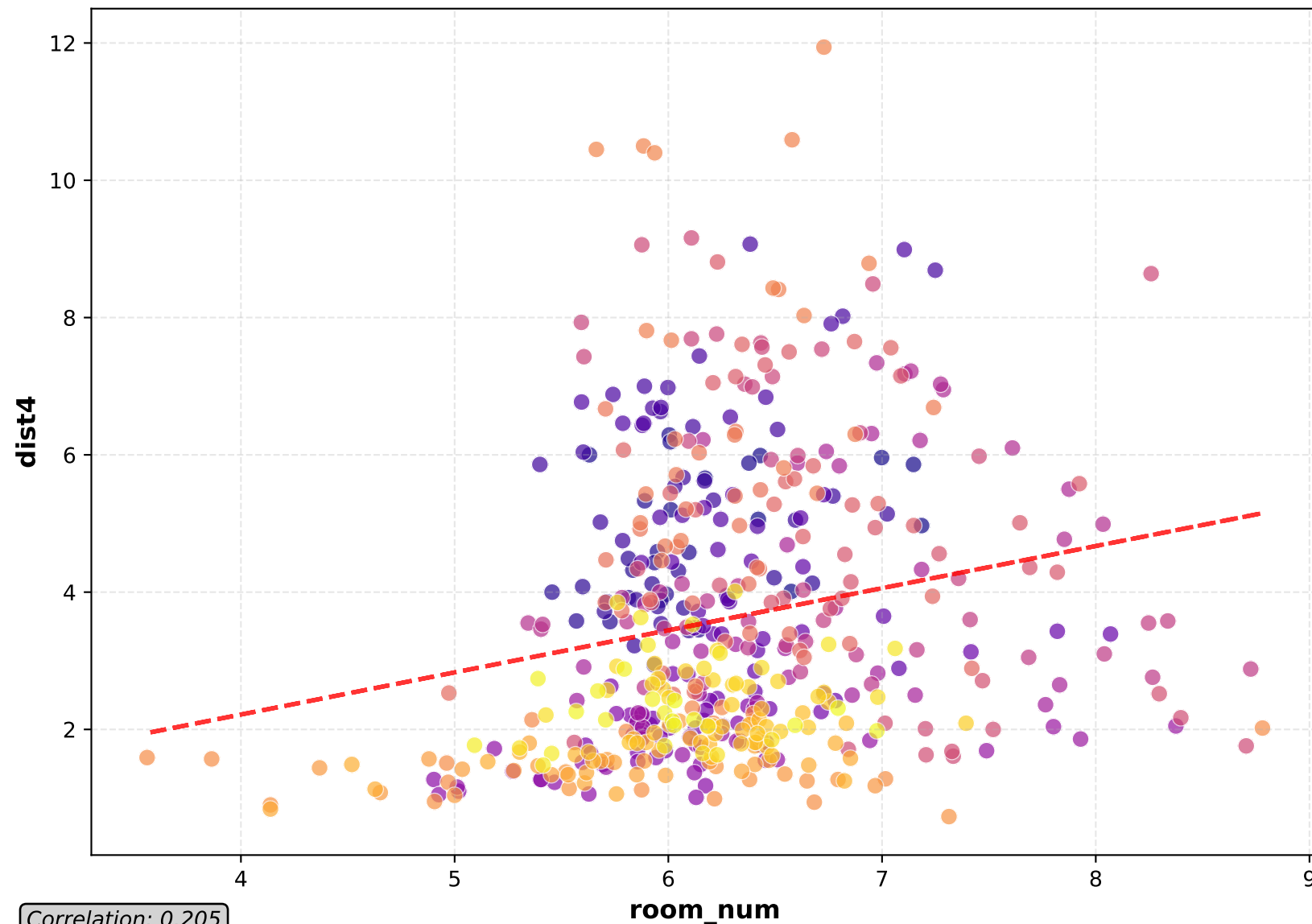
Scatter Plot
