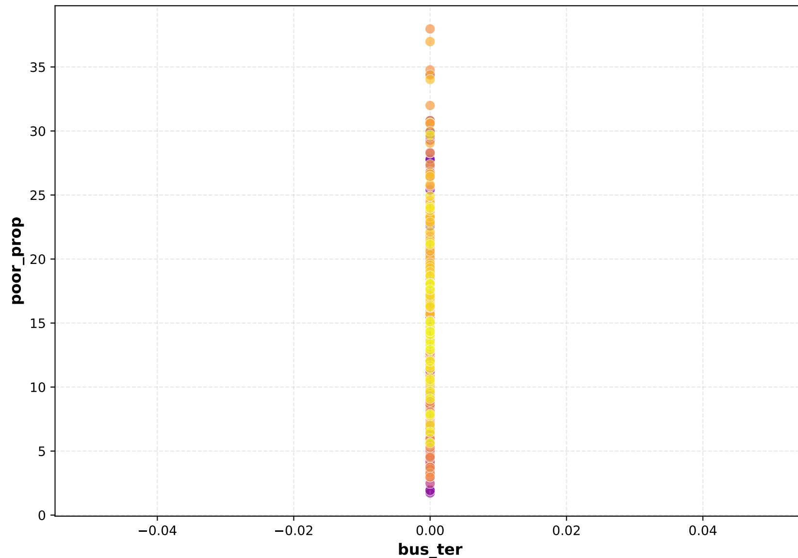
Scatter Plot
