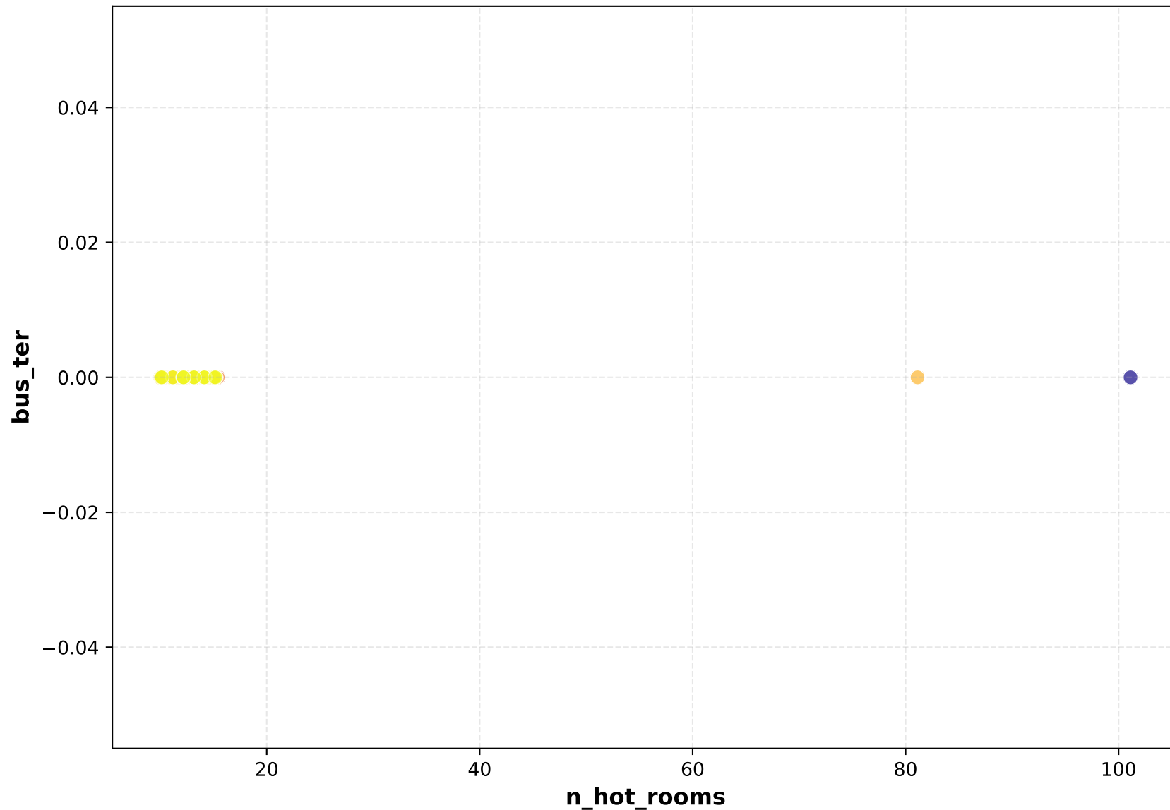
Scatter Plot
