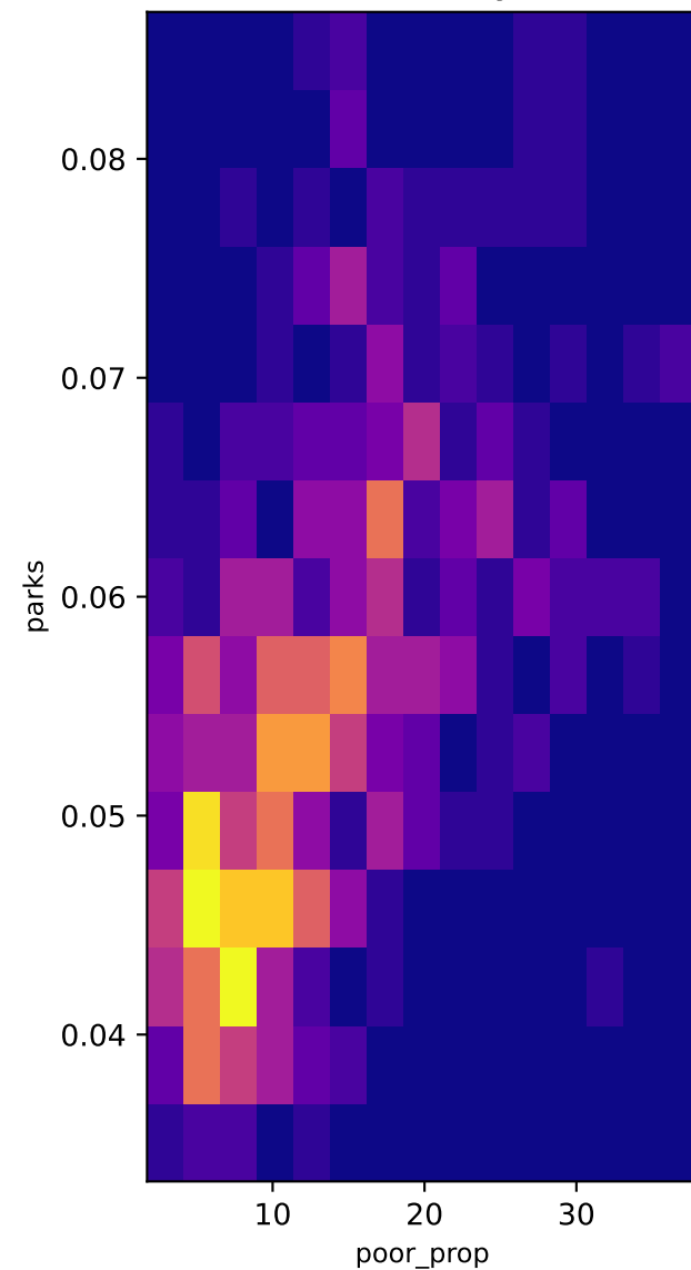
2D Density
