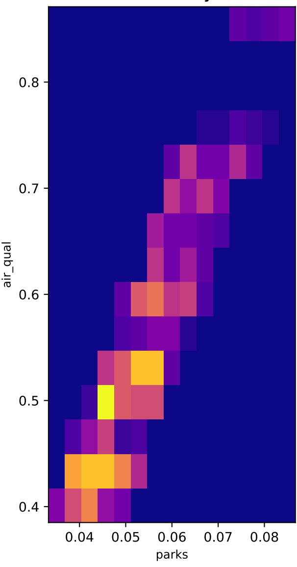
2D Density
