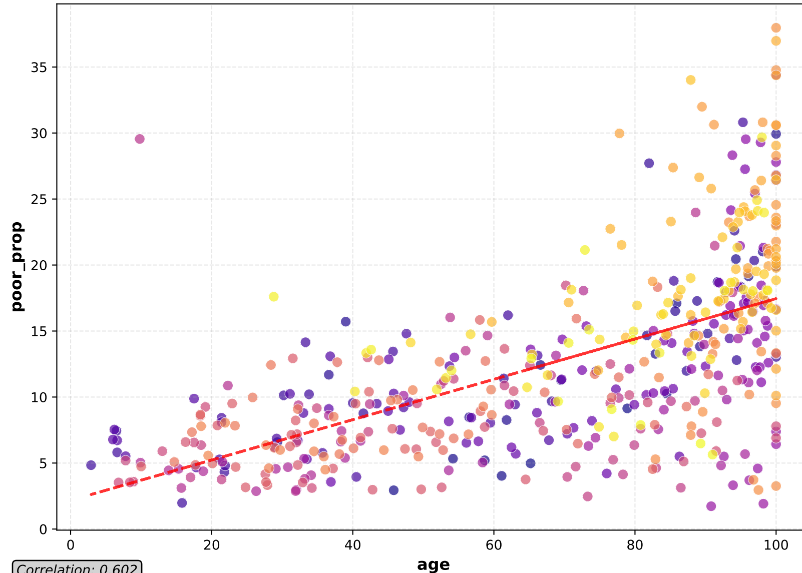
Scatter Plot
