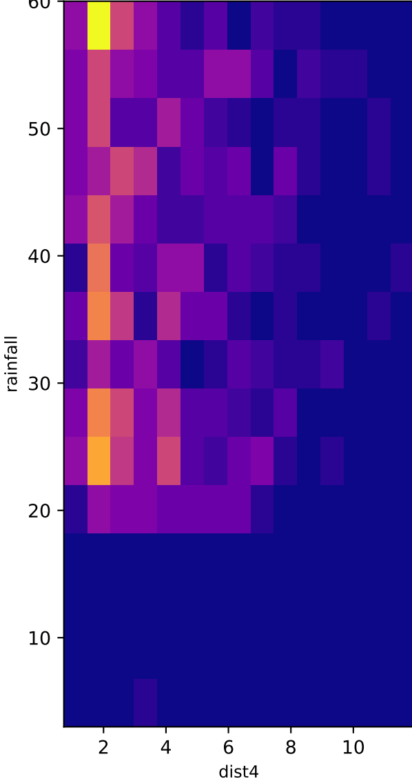
2D Density
