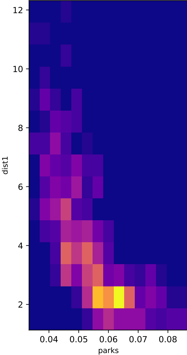
2D Density
