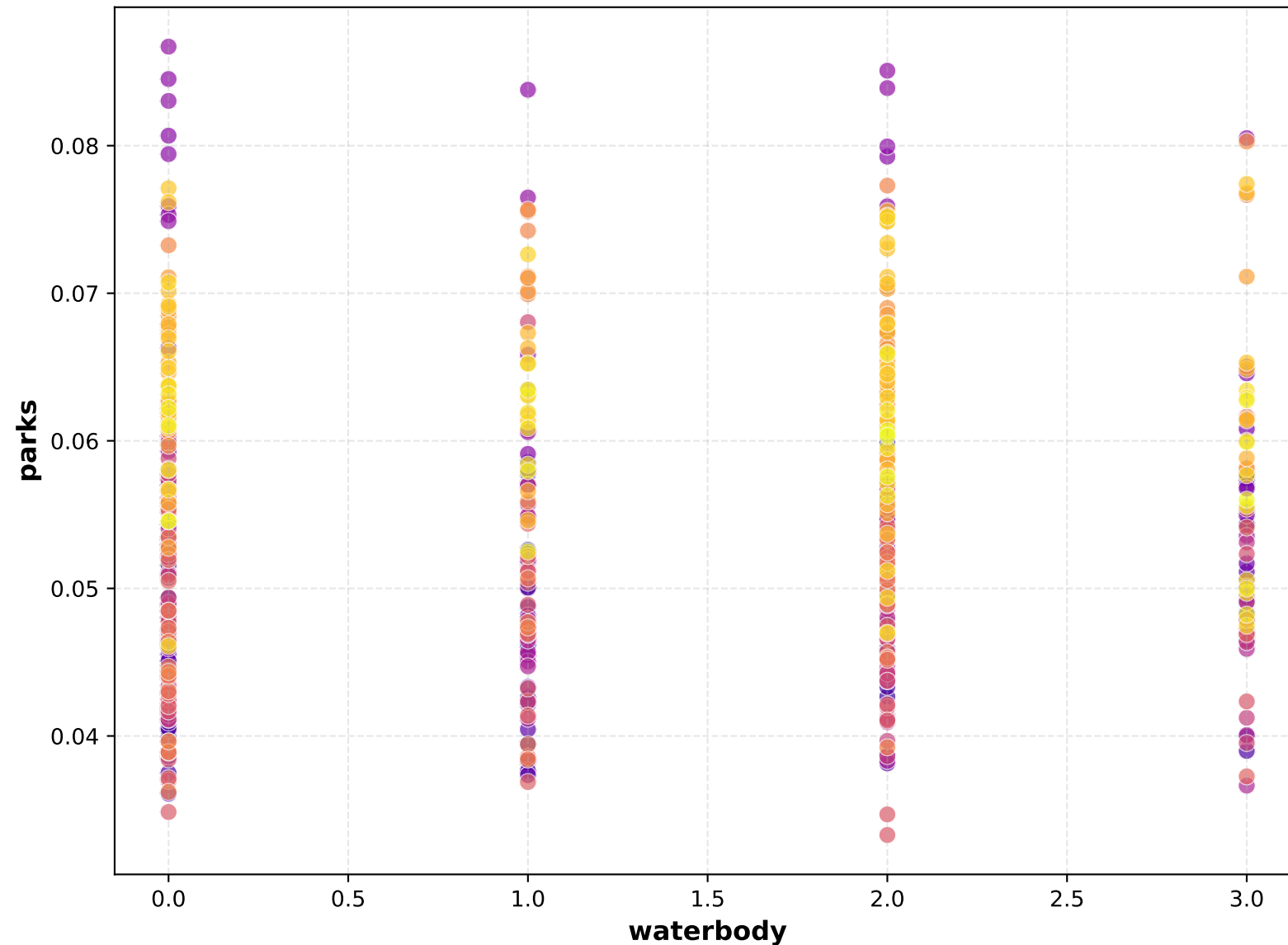
Scatter Plot
