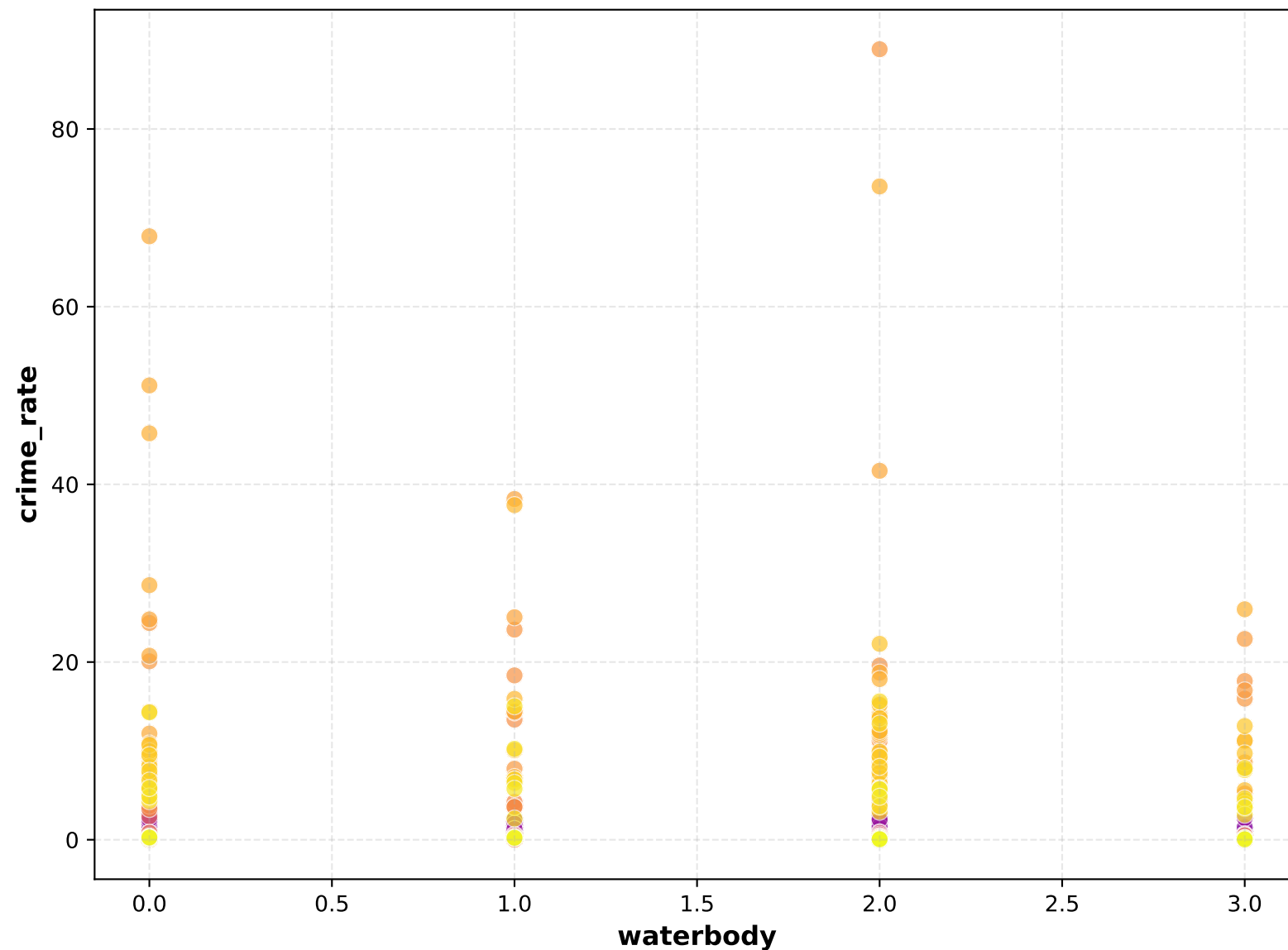
Scatter Plot
