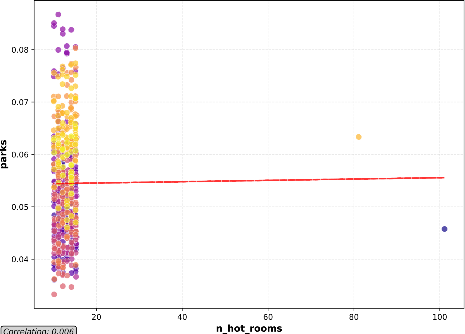
Scatter Plot
