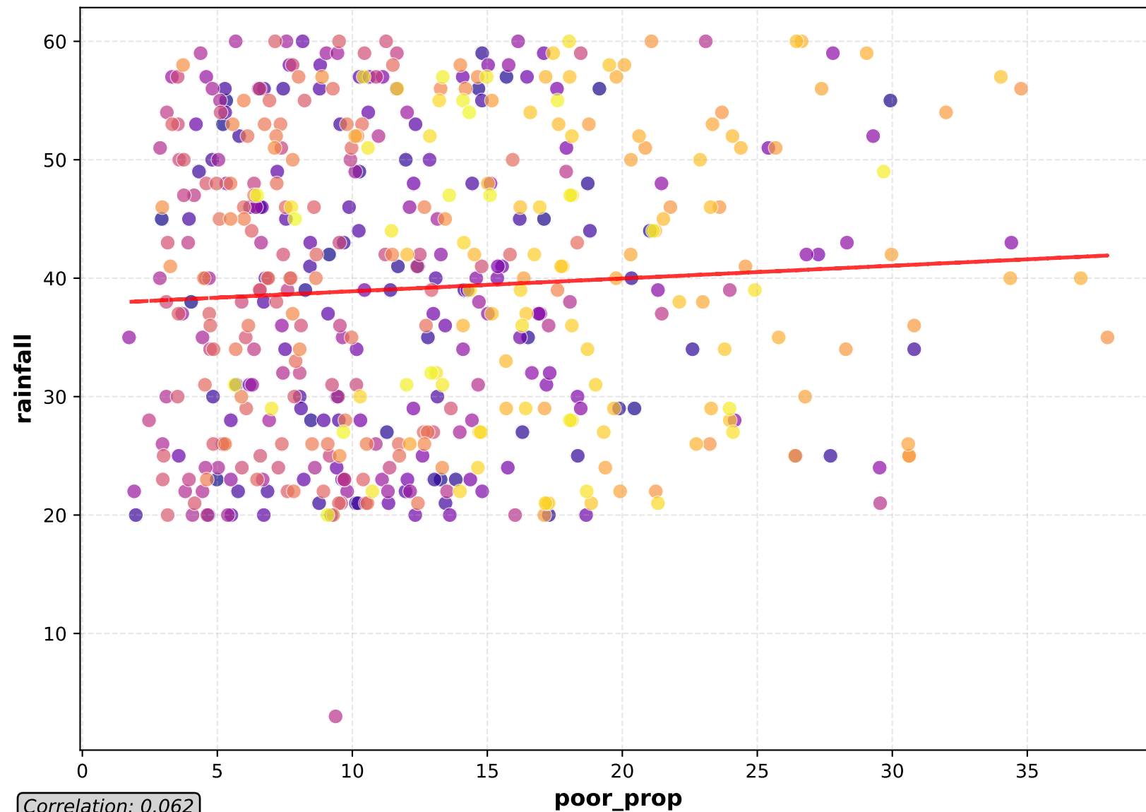
Scatter Plot
