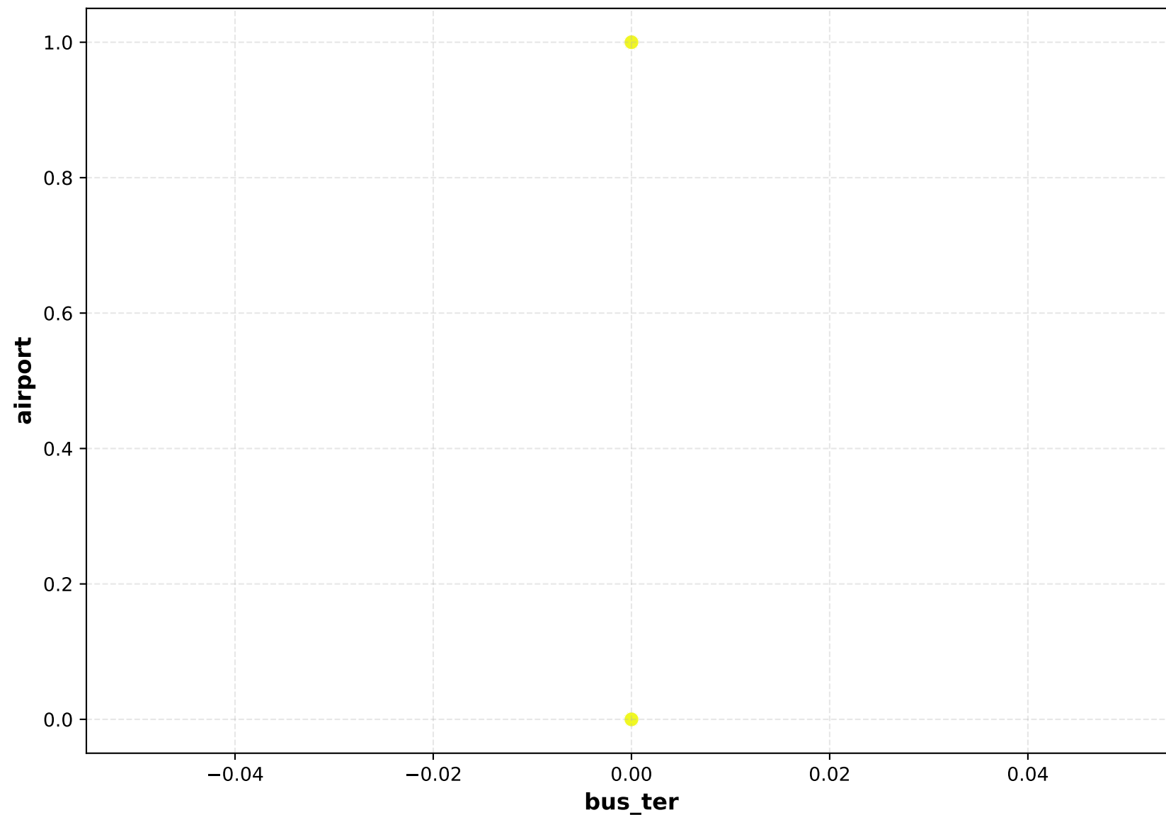
Scatter Plot
