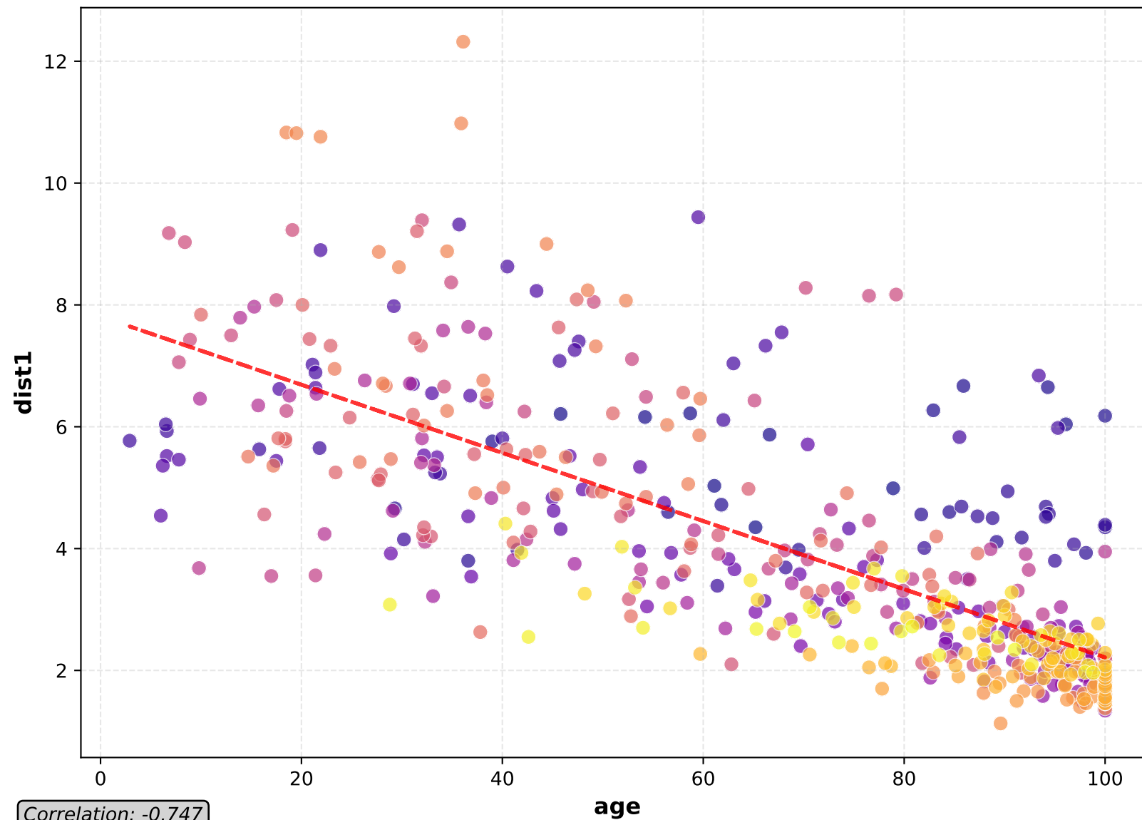
Scatter Plot
