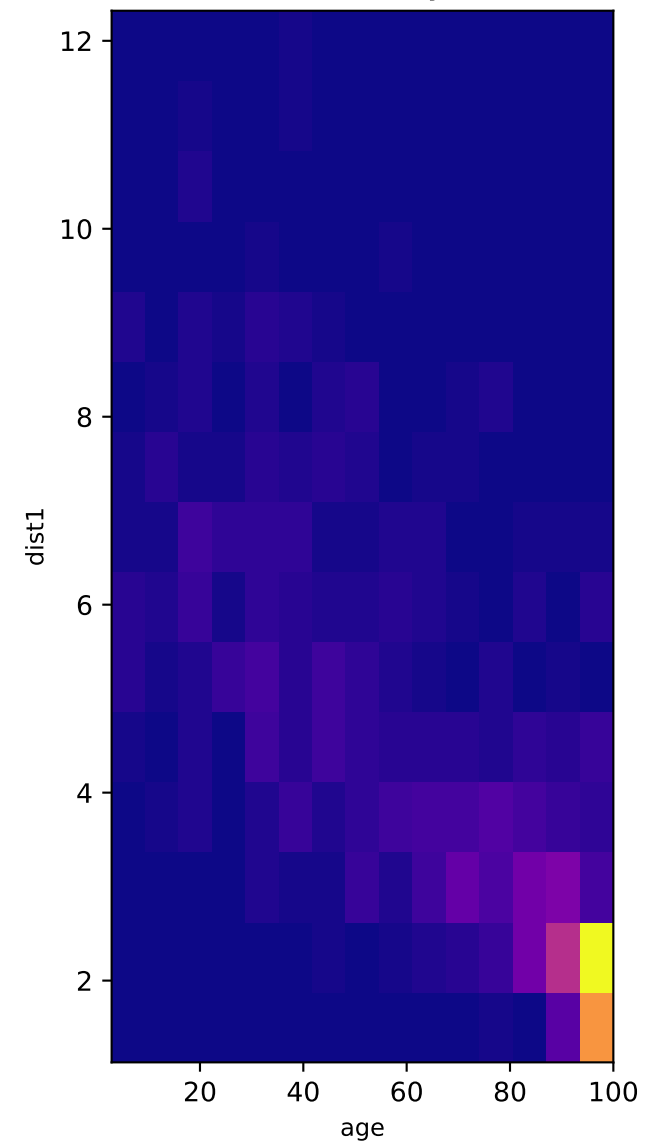
2D Density
