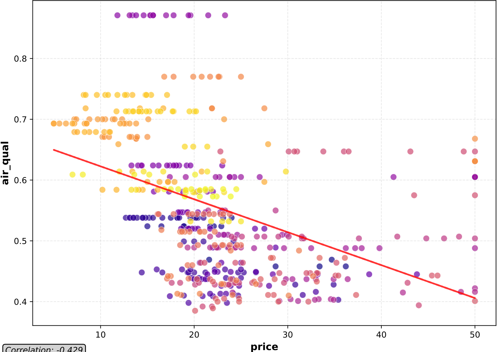
Scatter Plot
