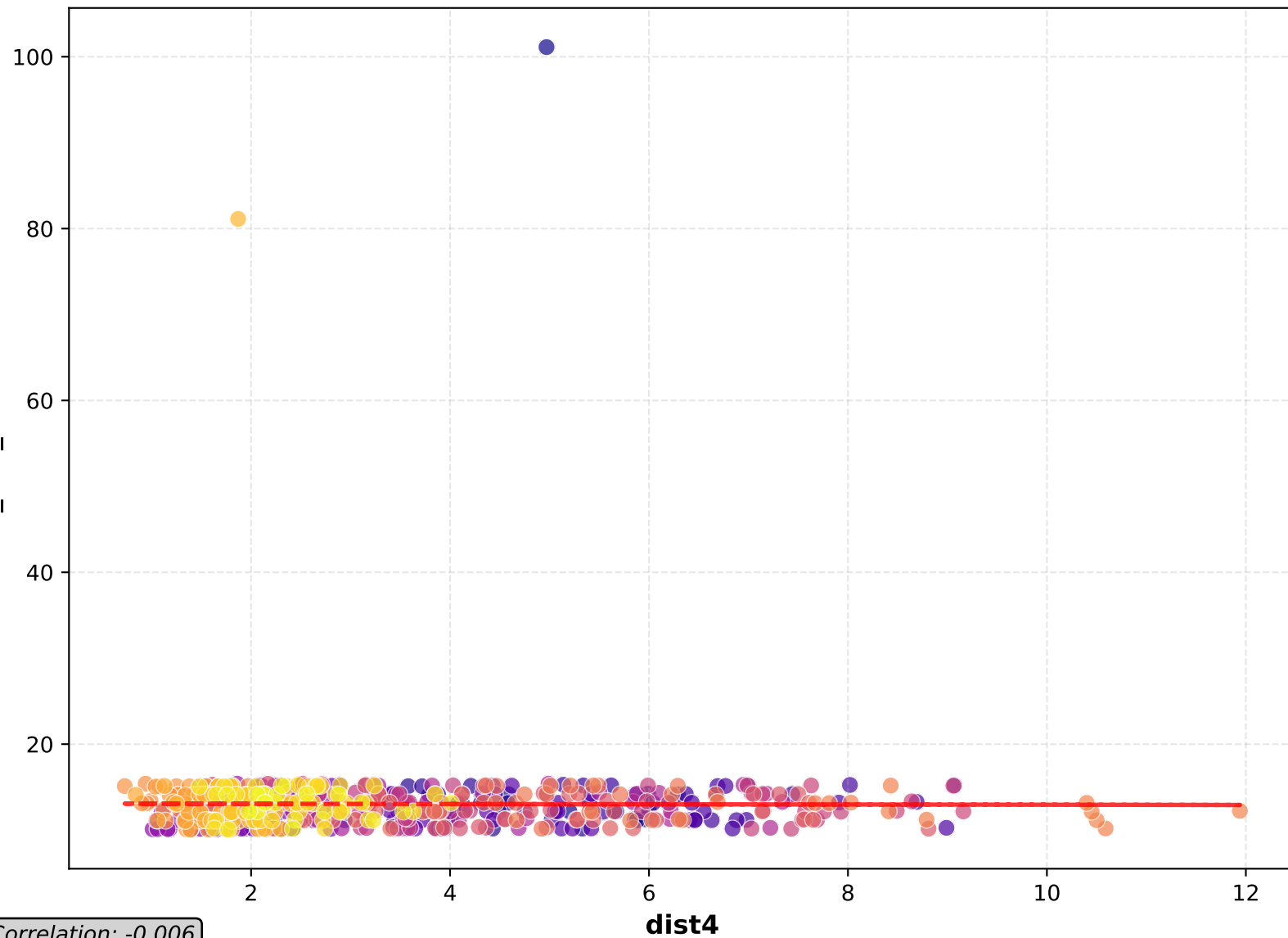
Scatter Plot
