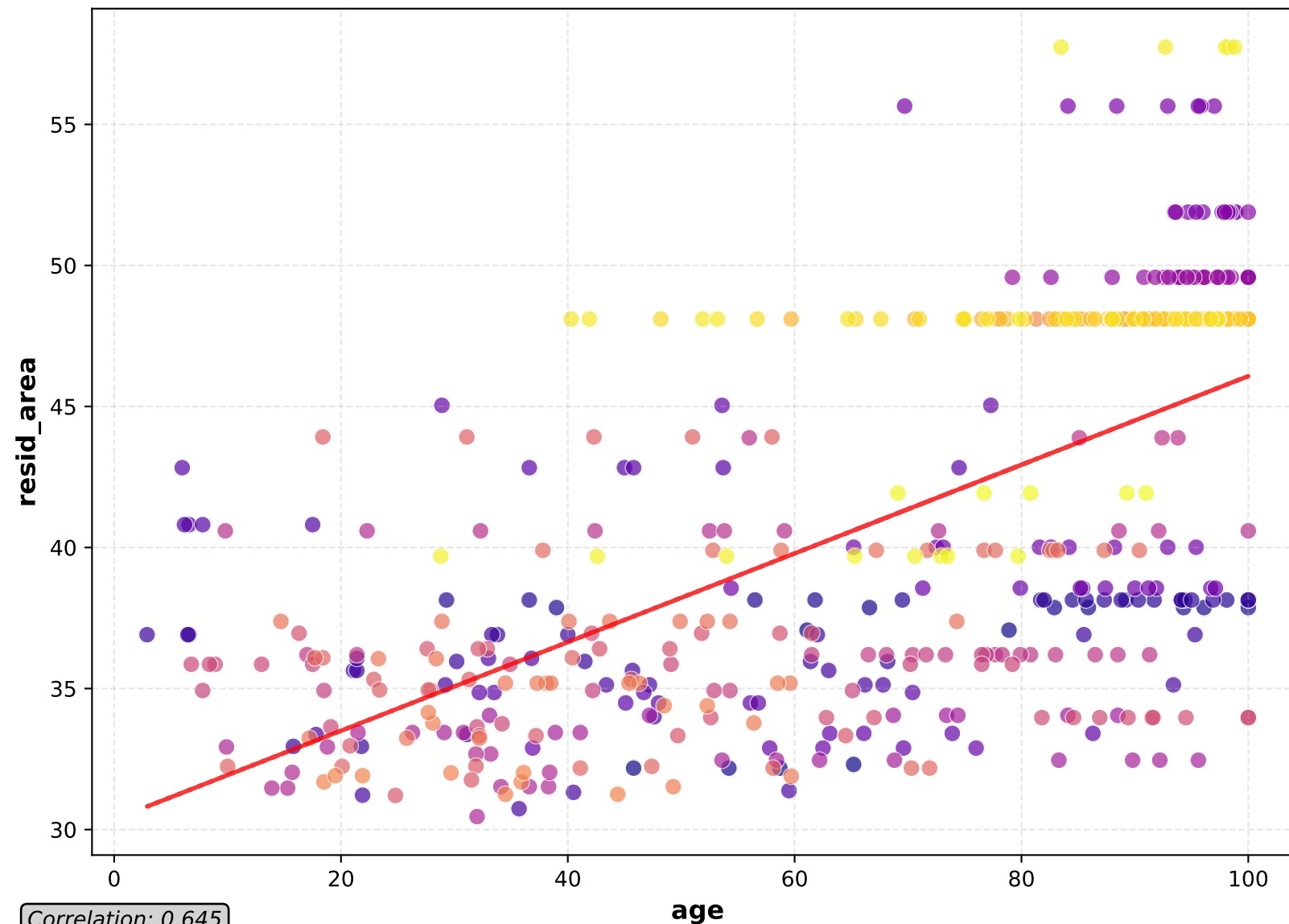
Scatter Plot
