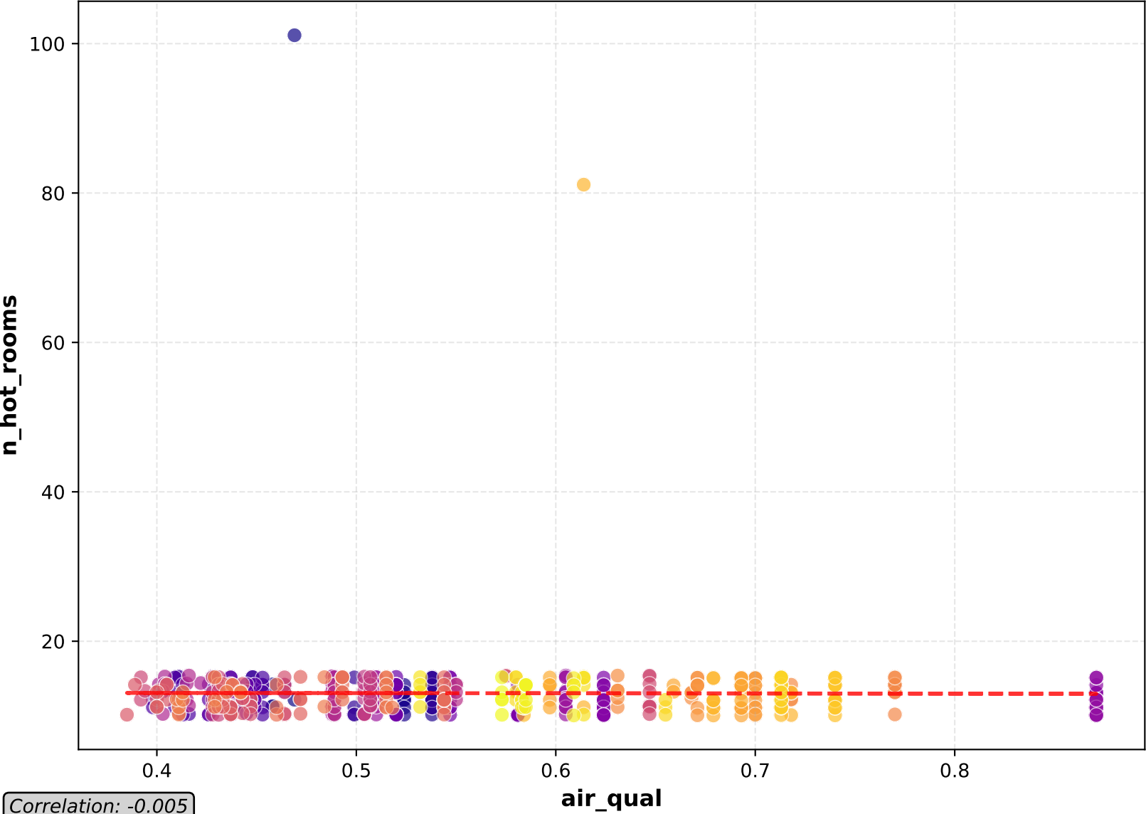
Scatter Plot
