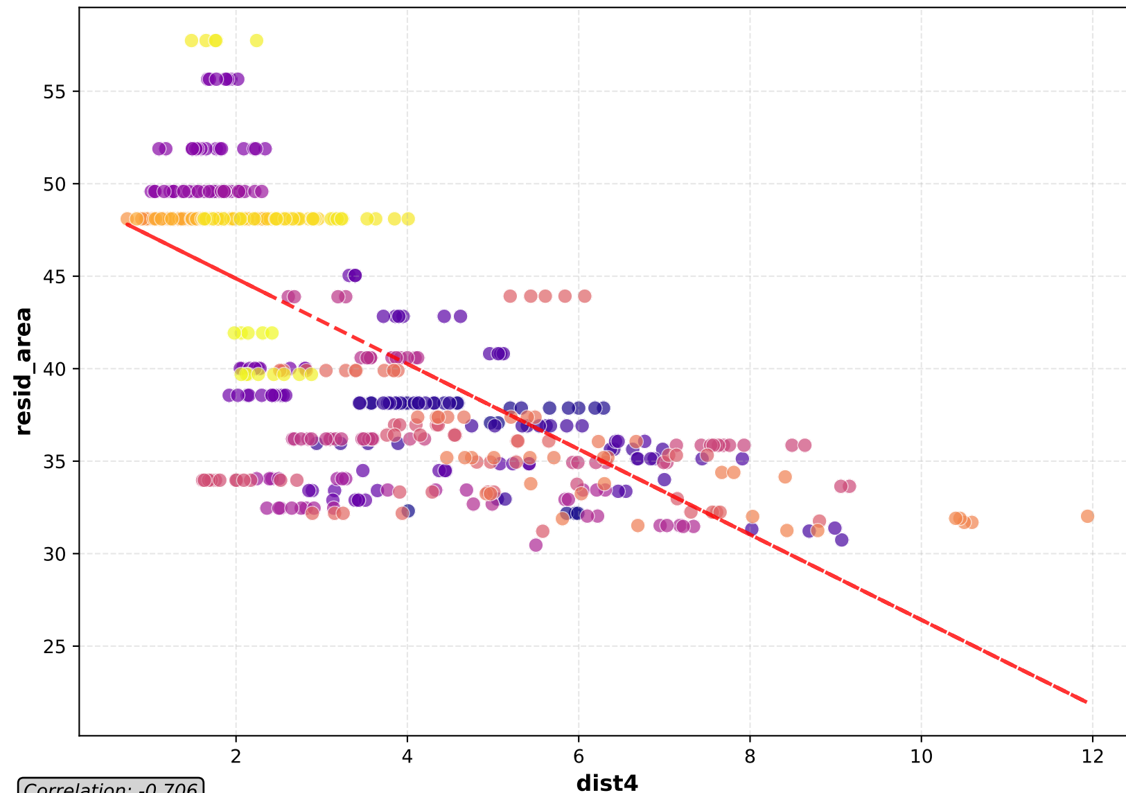
Scatter Plot
