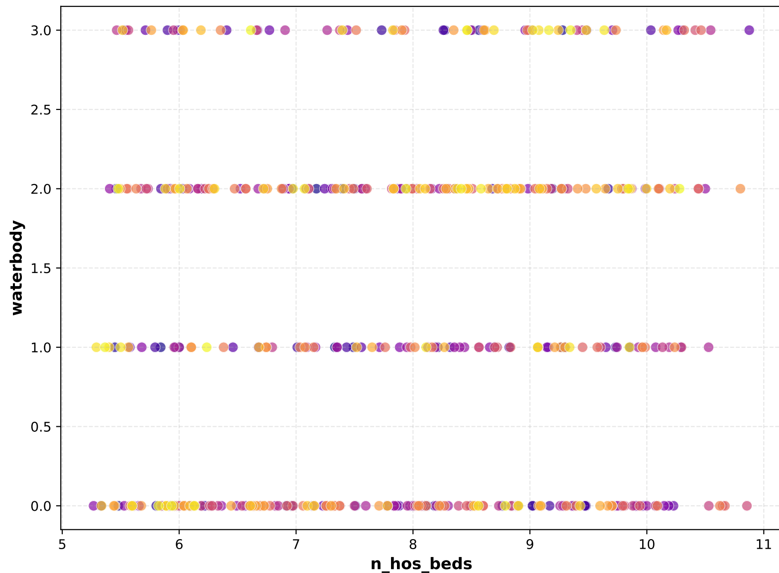
Scatter Plot
