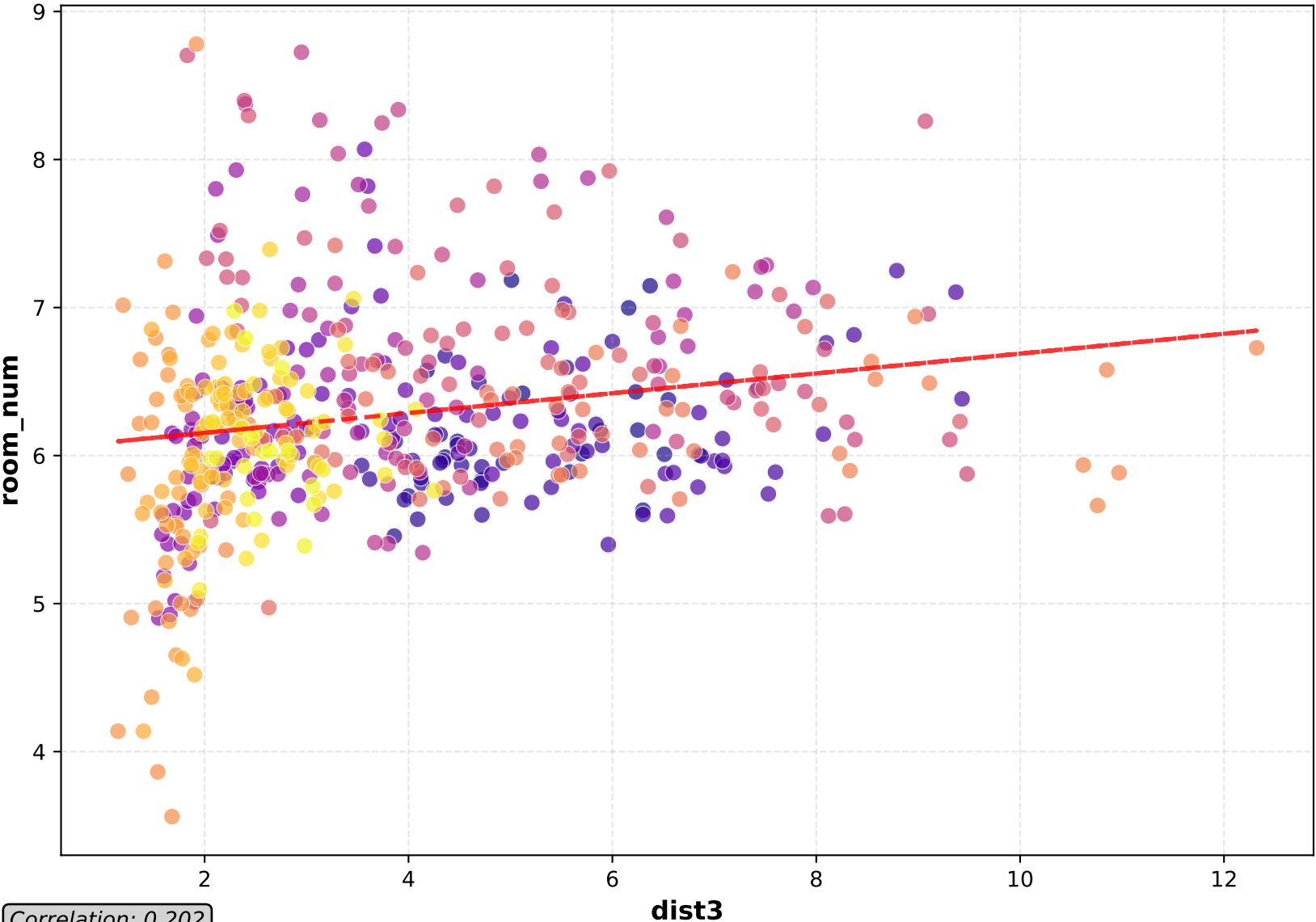
Scatter Plot
