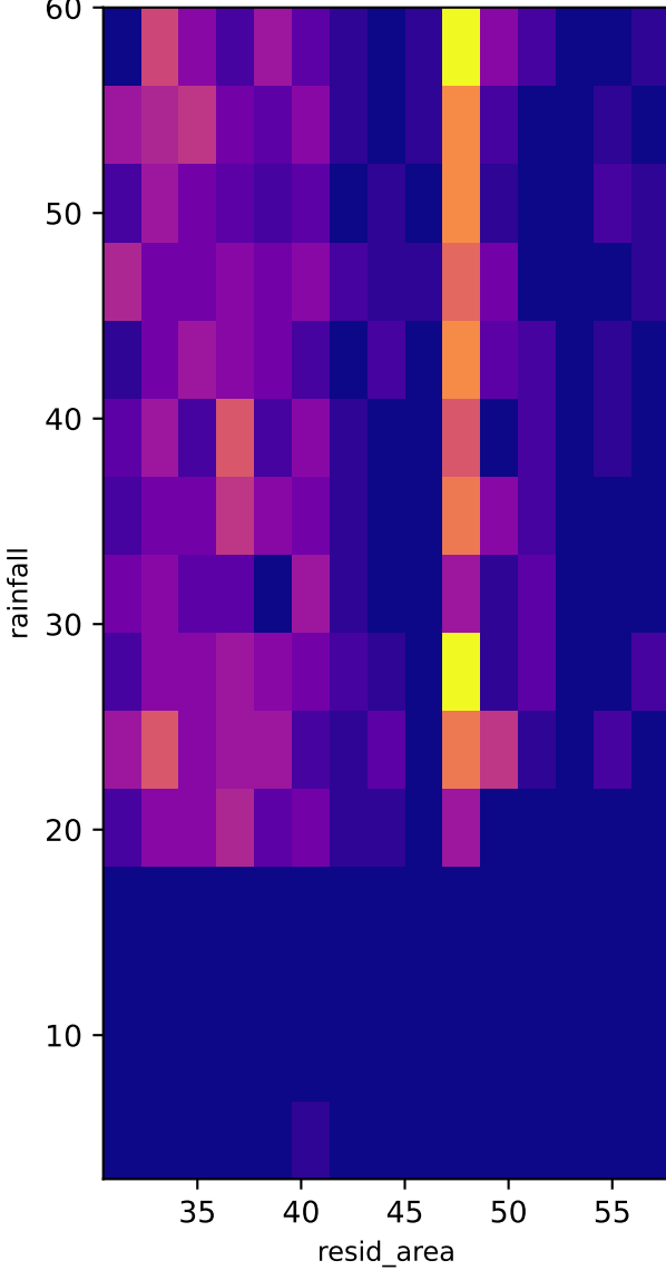
2D Density
