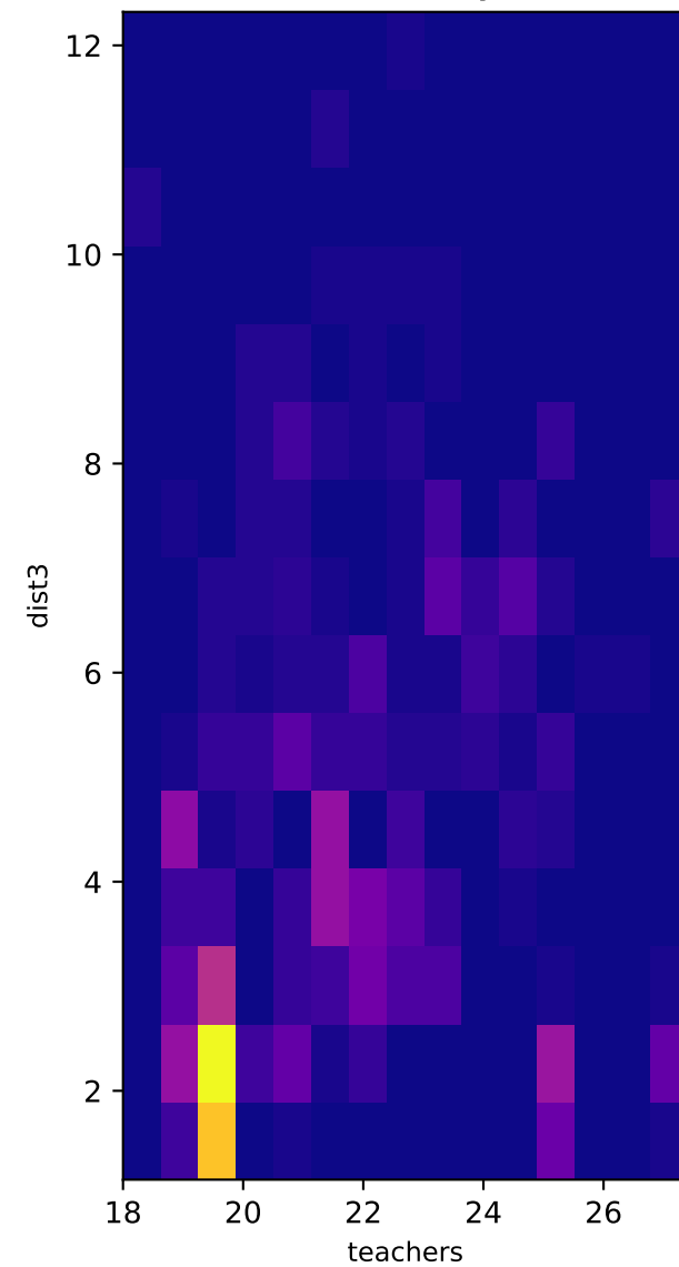
2D Density
