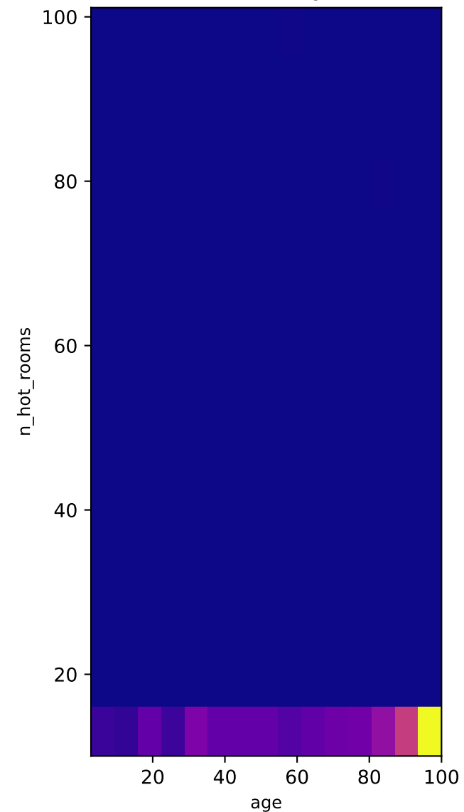
2D Density
