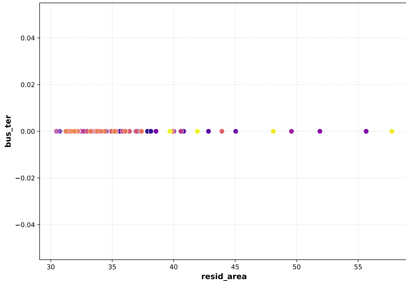
Scatter Plot
