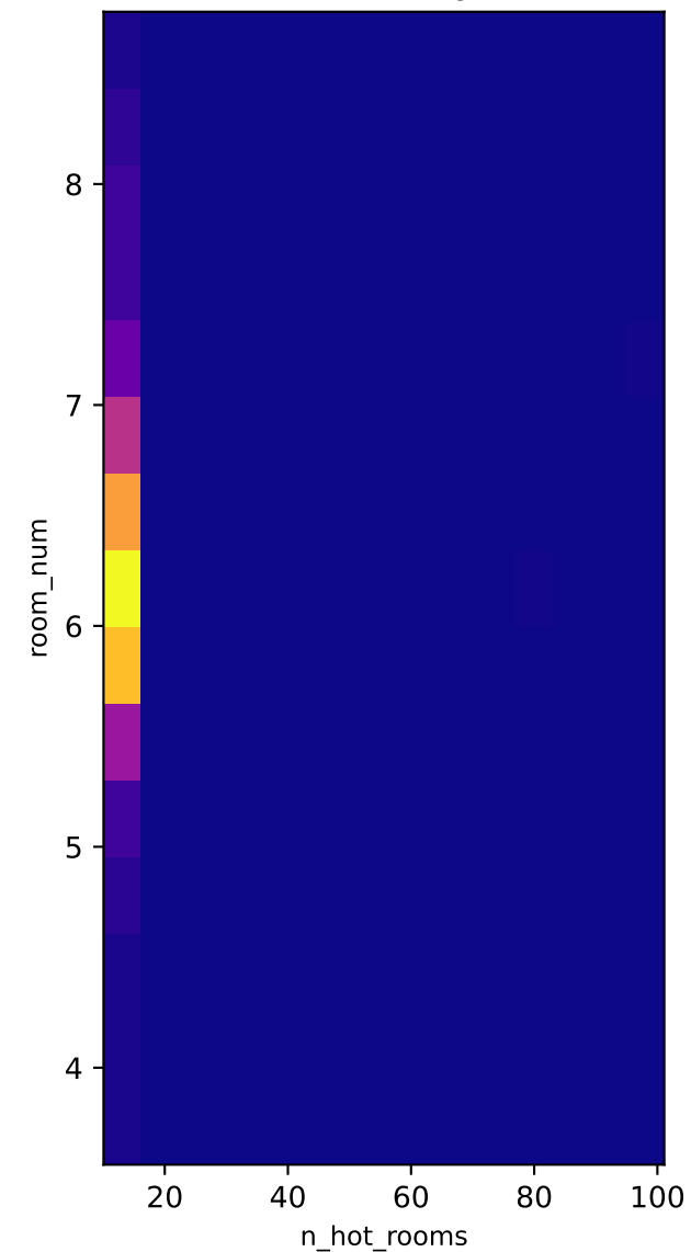
2D Density
