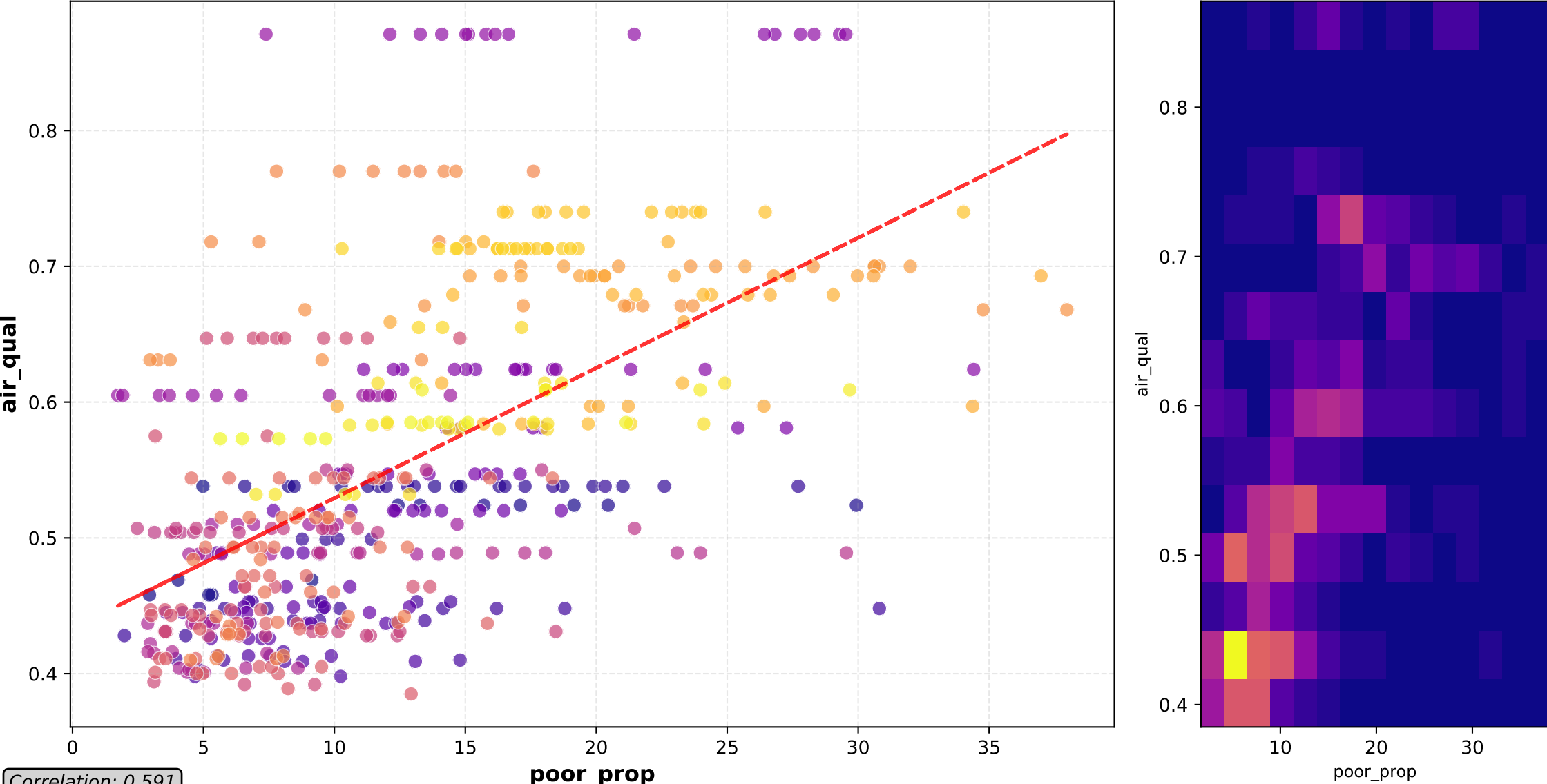
Scatter Plot
