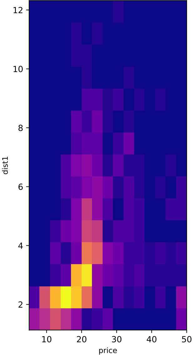
2D Density
