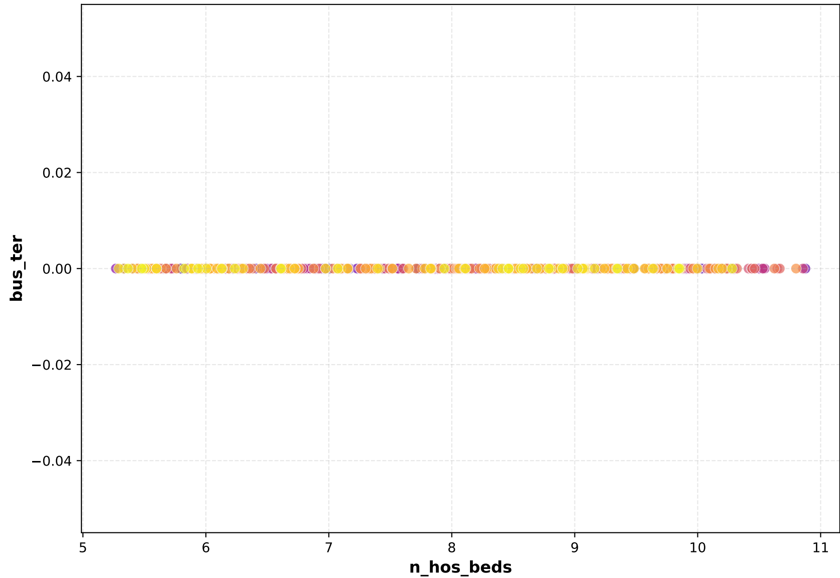
Scatter Plot
