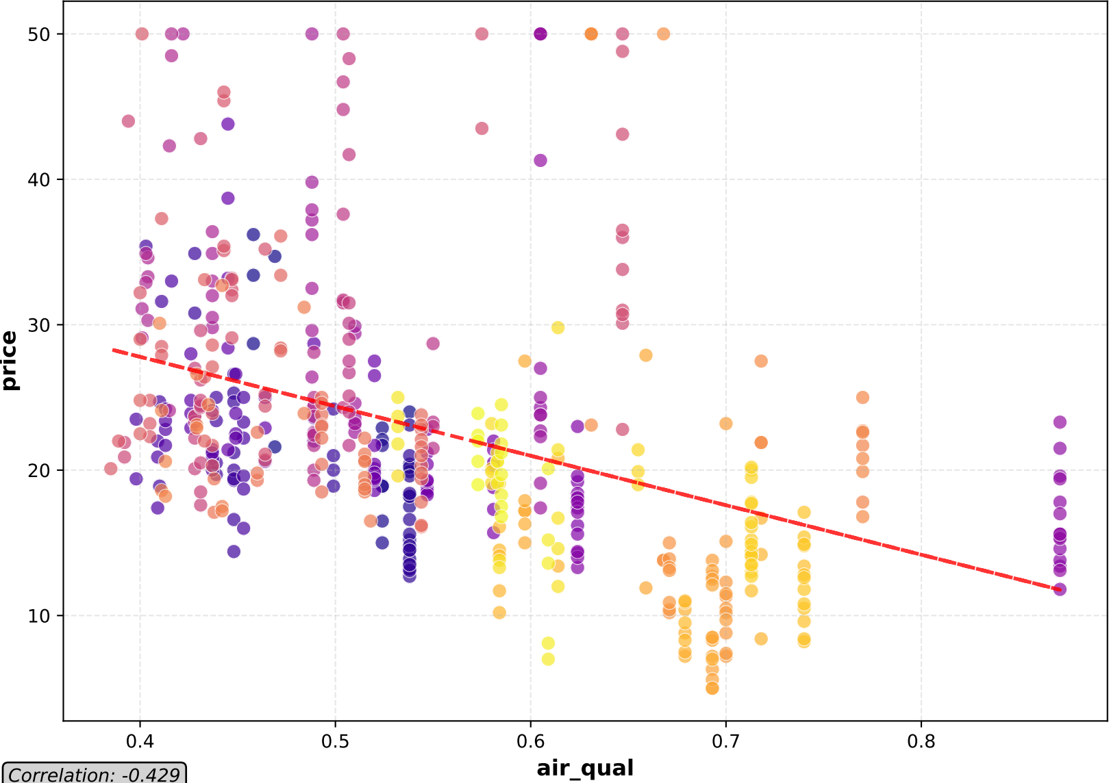
Scatter Plot
