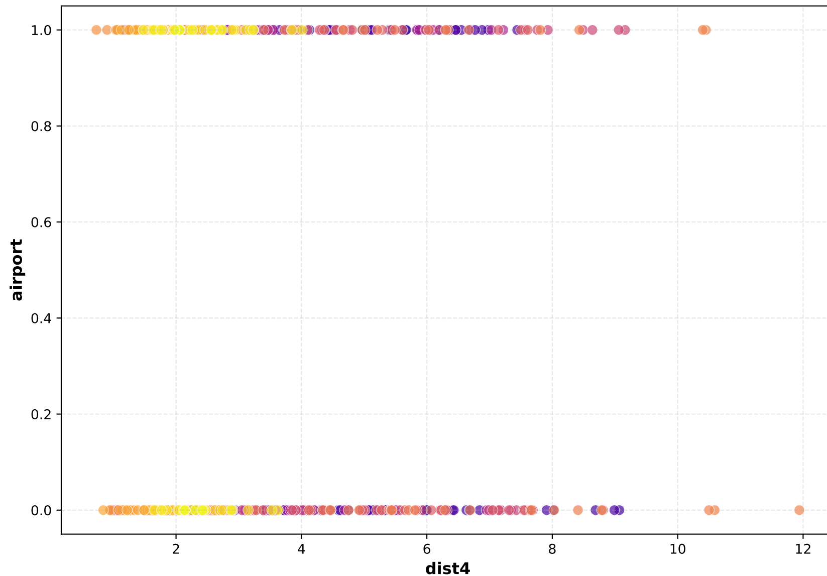
Scatter Plot
