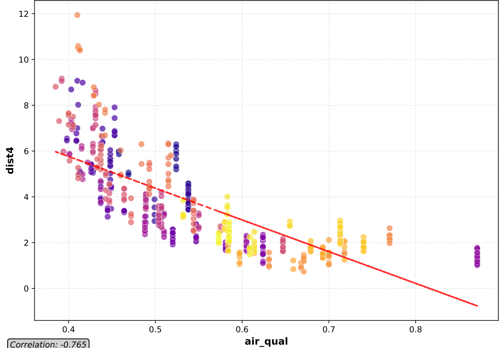
Scatter Plot
