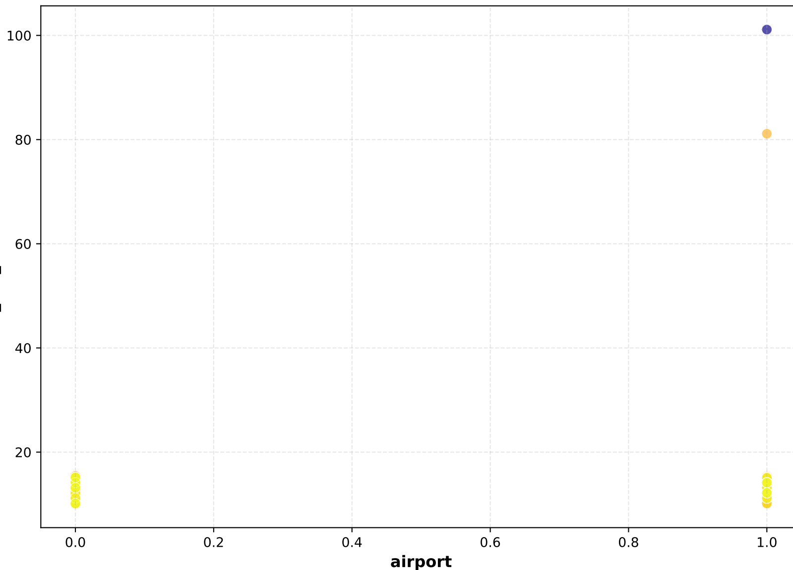
Scatter Plot
