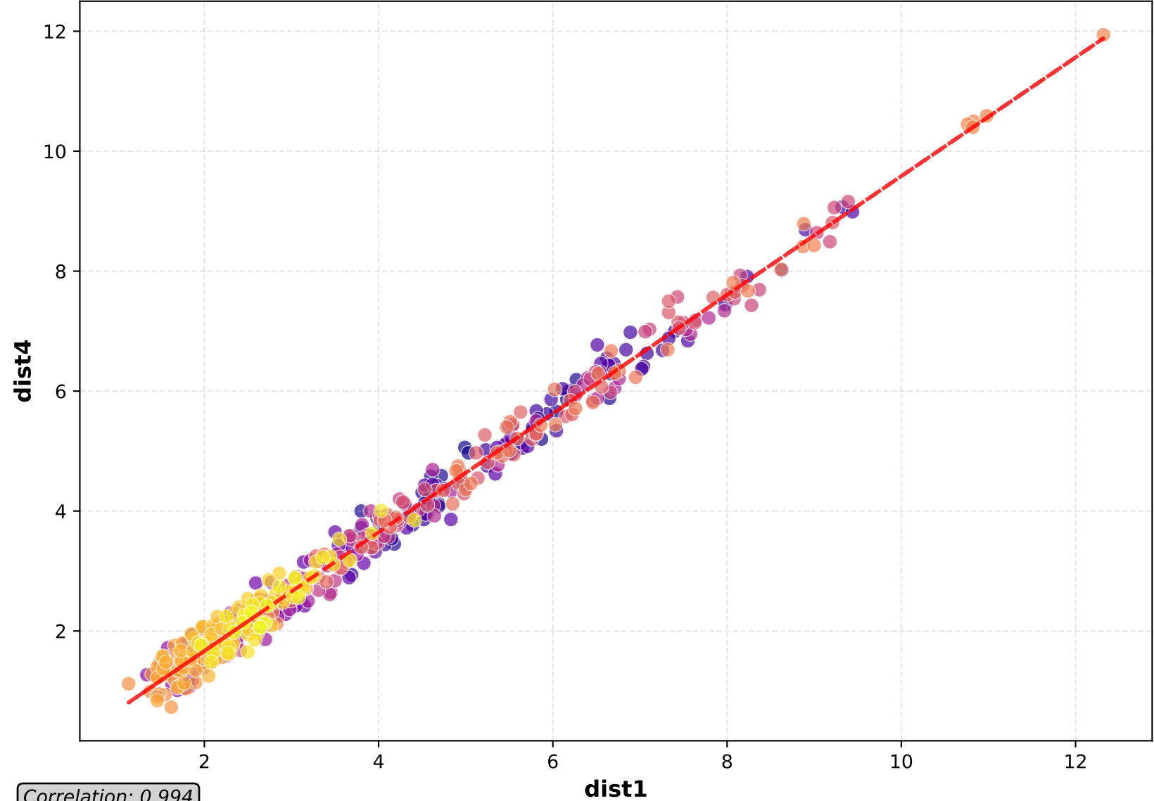
Scatter Plot
