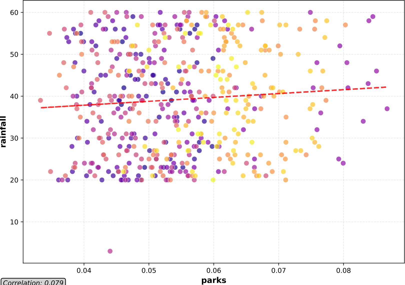
Scatter Plot
