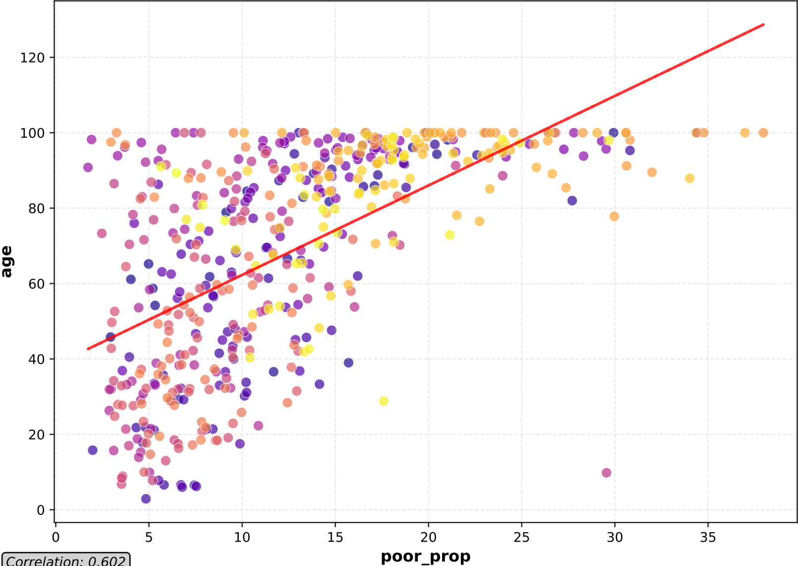
Scatter Plot
