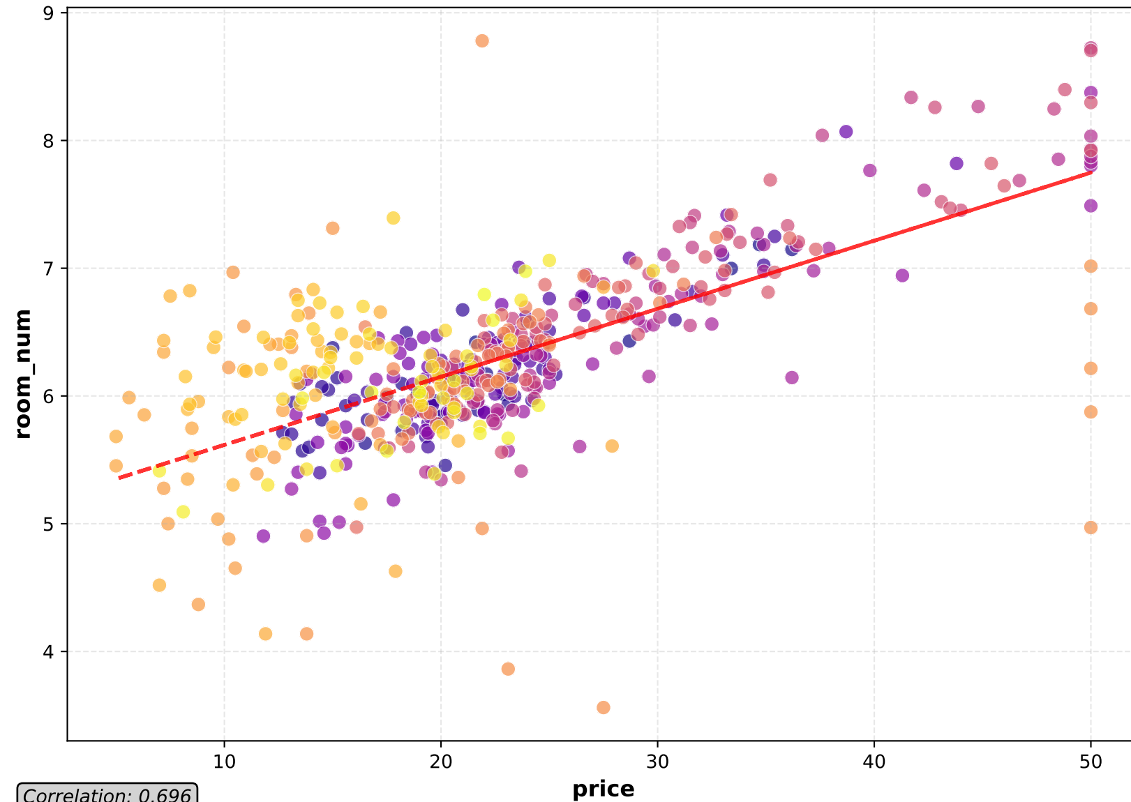
Scatter Plot
