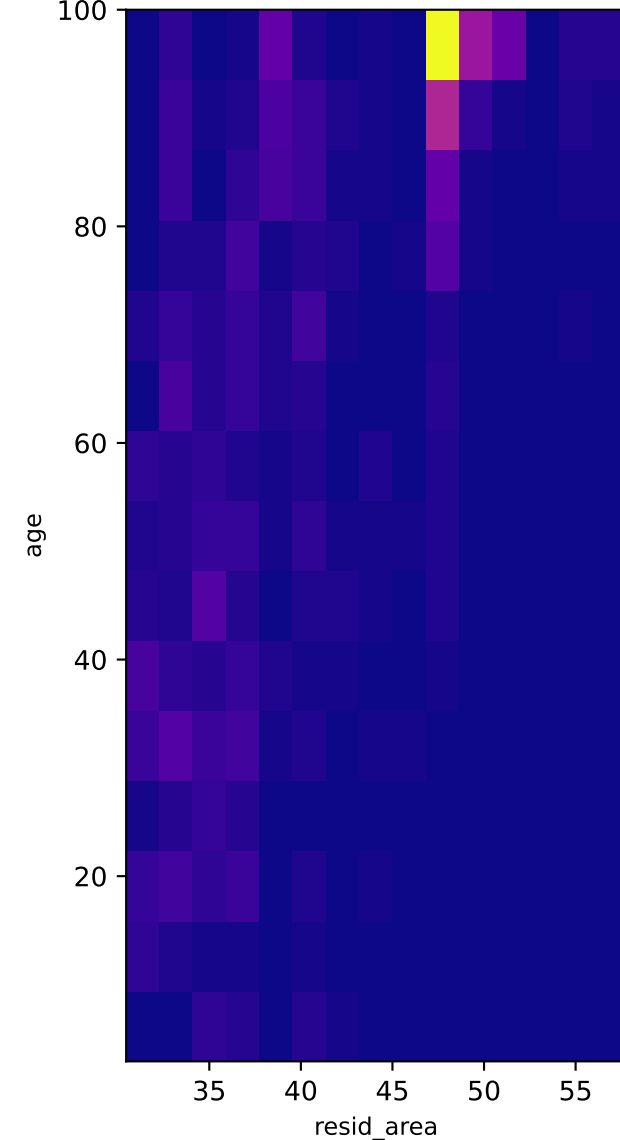
2D Density
