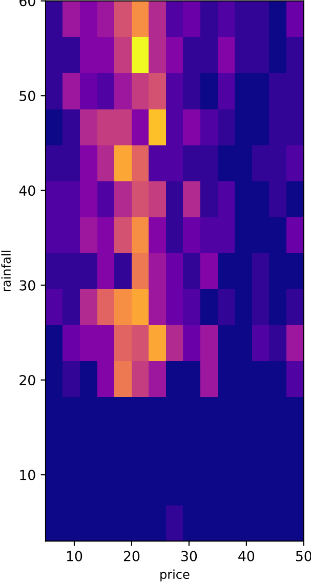
2D Density
