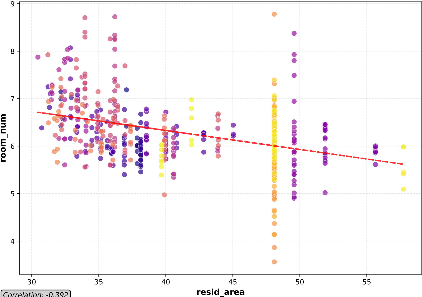
Scatter Plot
