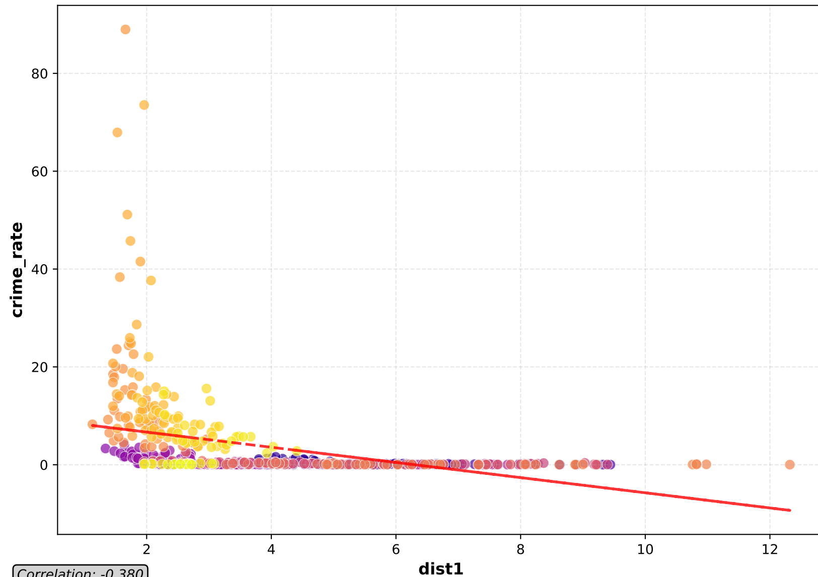
Scatter Plot
