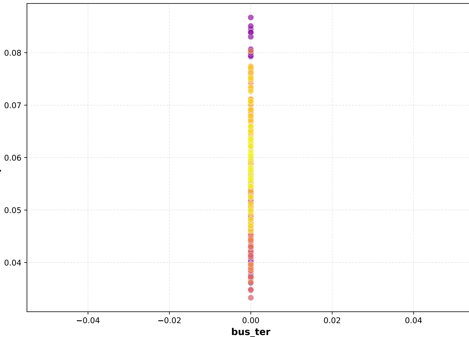
Scatter Plot
