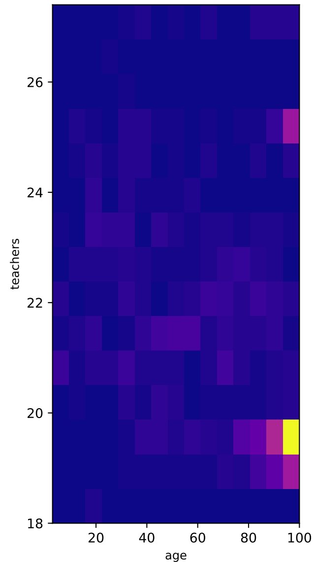
2D Density
