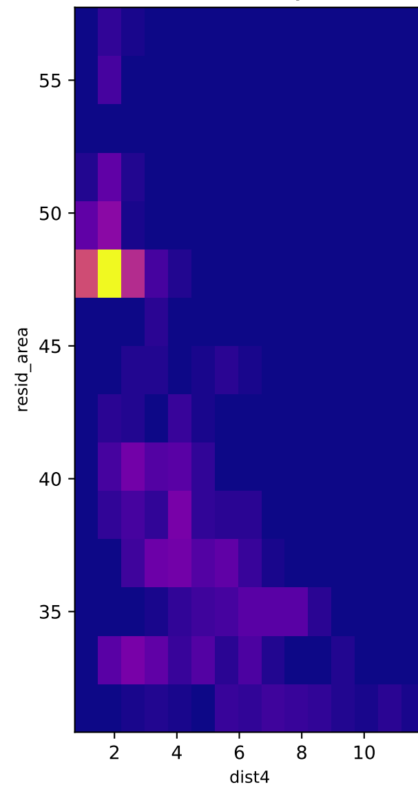
2D Density
