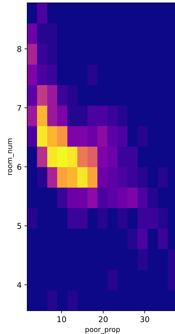
2D Density
