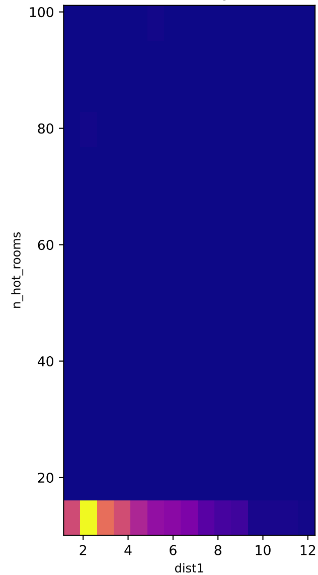
2D Density
