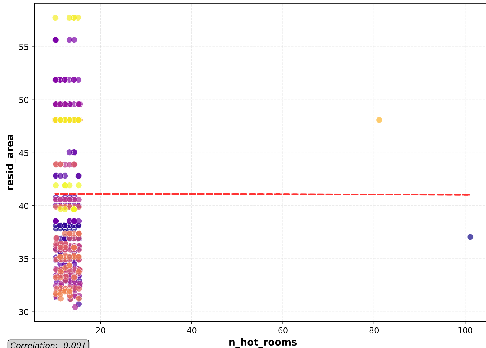
Scatter Plot
