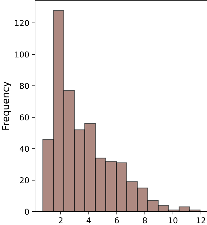
dist4 Distribution
