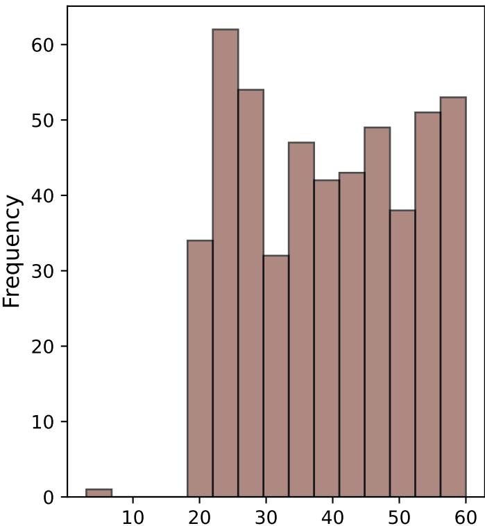
rainfall Distribution
