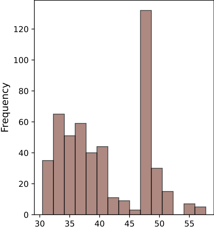
resid_area Distribution
