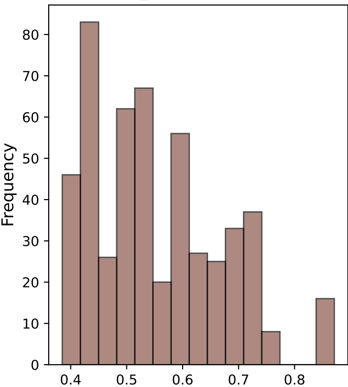
air_qual Distribution
