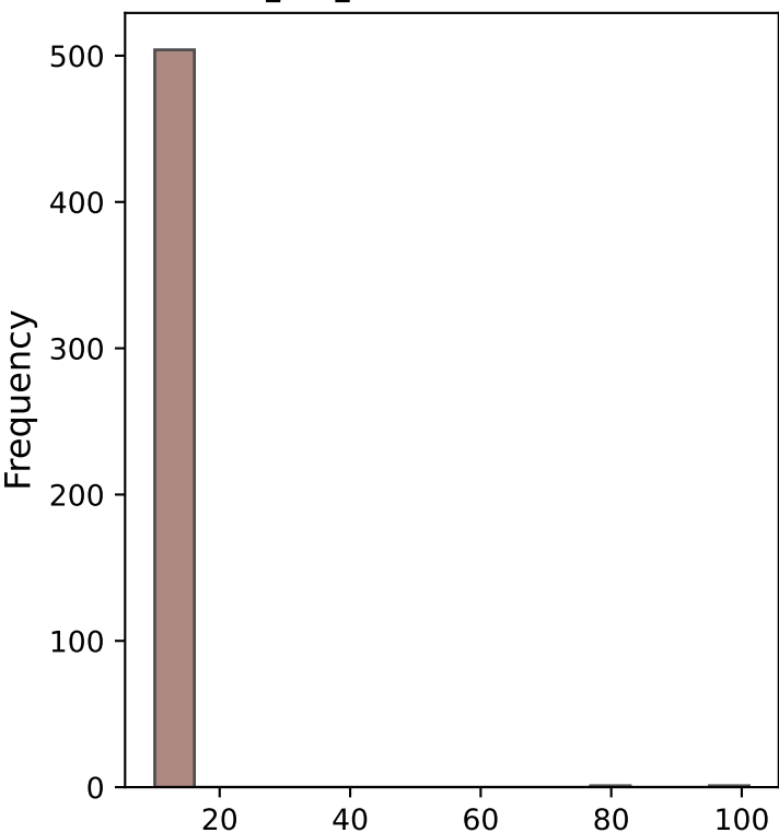
n_hot_rooms Distribution
