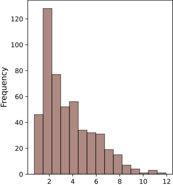
dist4 Distribution
