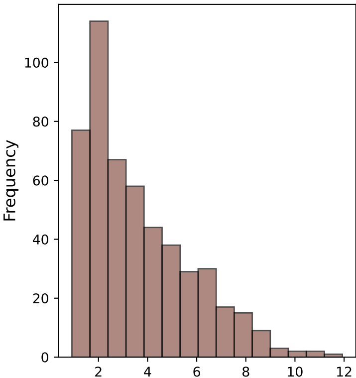
dist2 Distribution
