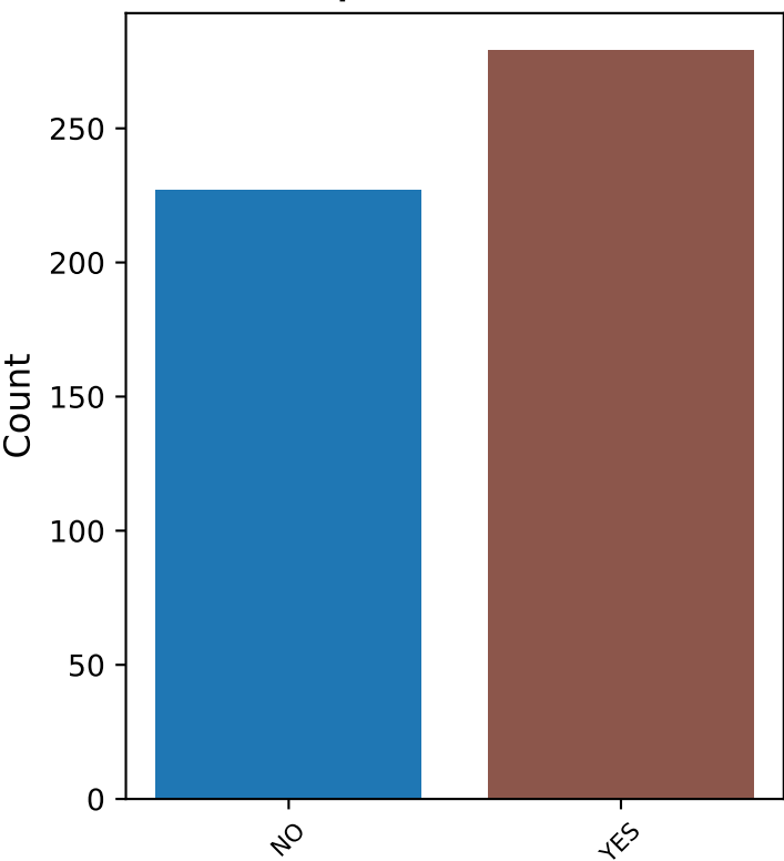
airport Distribution
