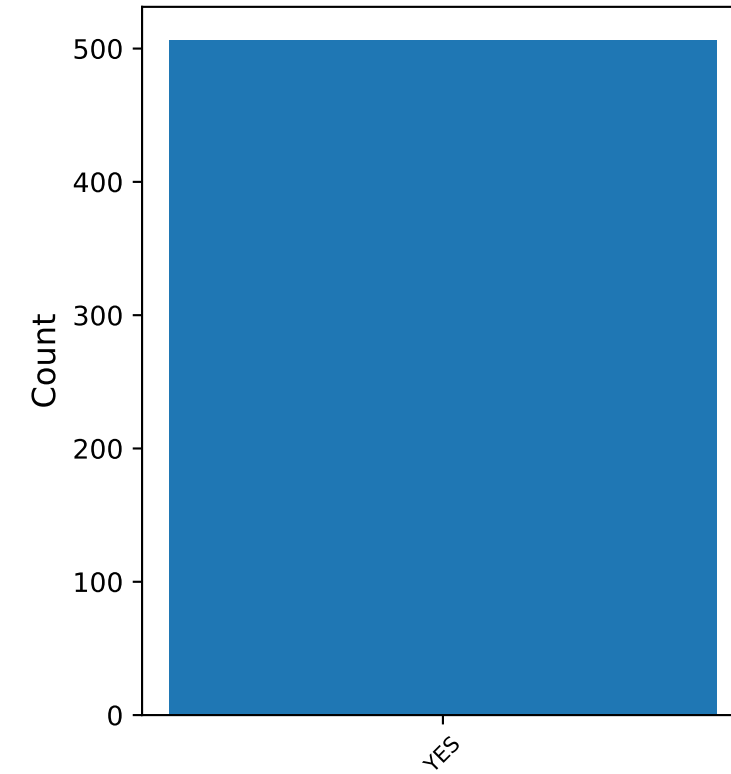
bus_ter Distribution
