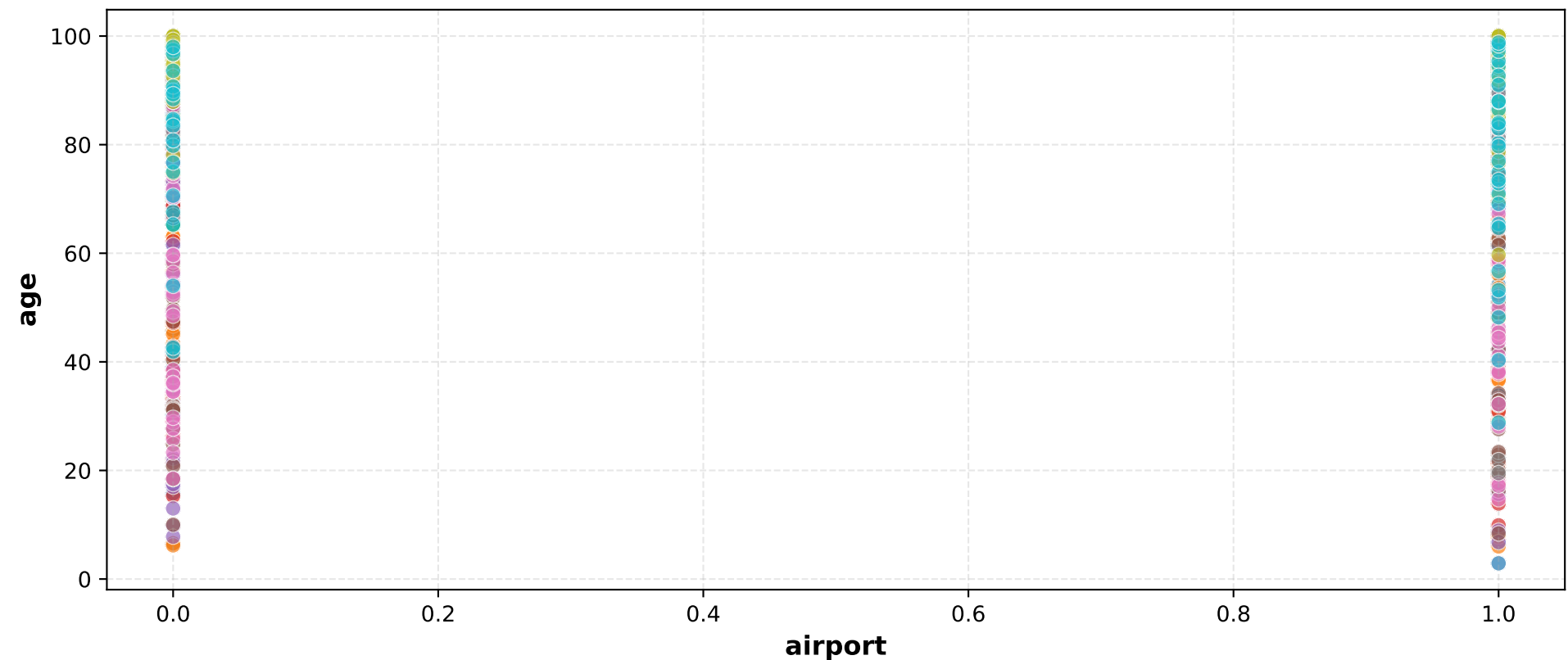
Scatter Plot
