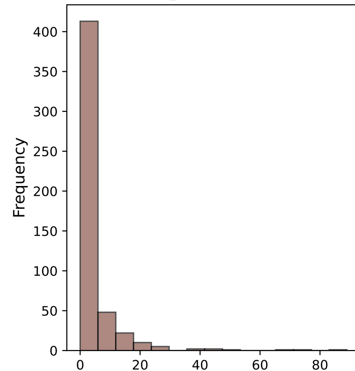
crime_rate Distribution
