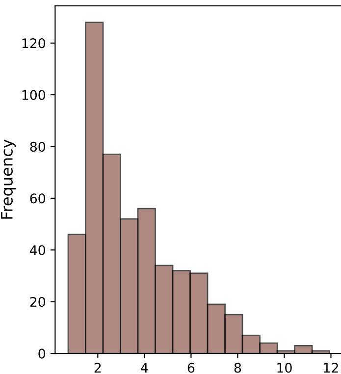
dist4 Distribution
