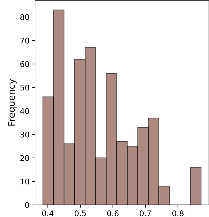
air_qual Distribution
