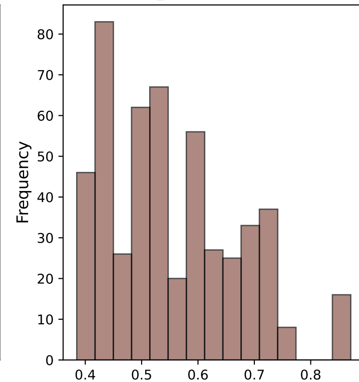
air_qual Distribution
