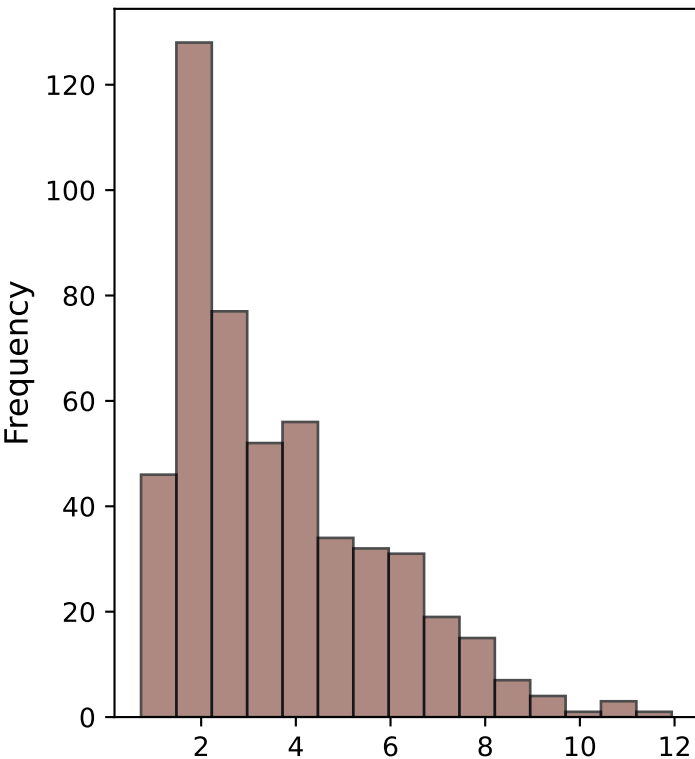
dist4 Distribution
