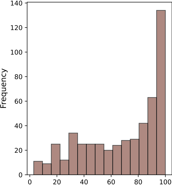
age Distribution
