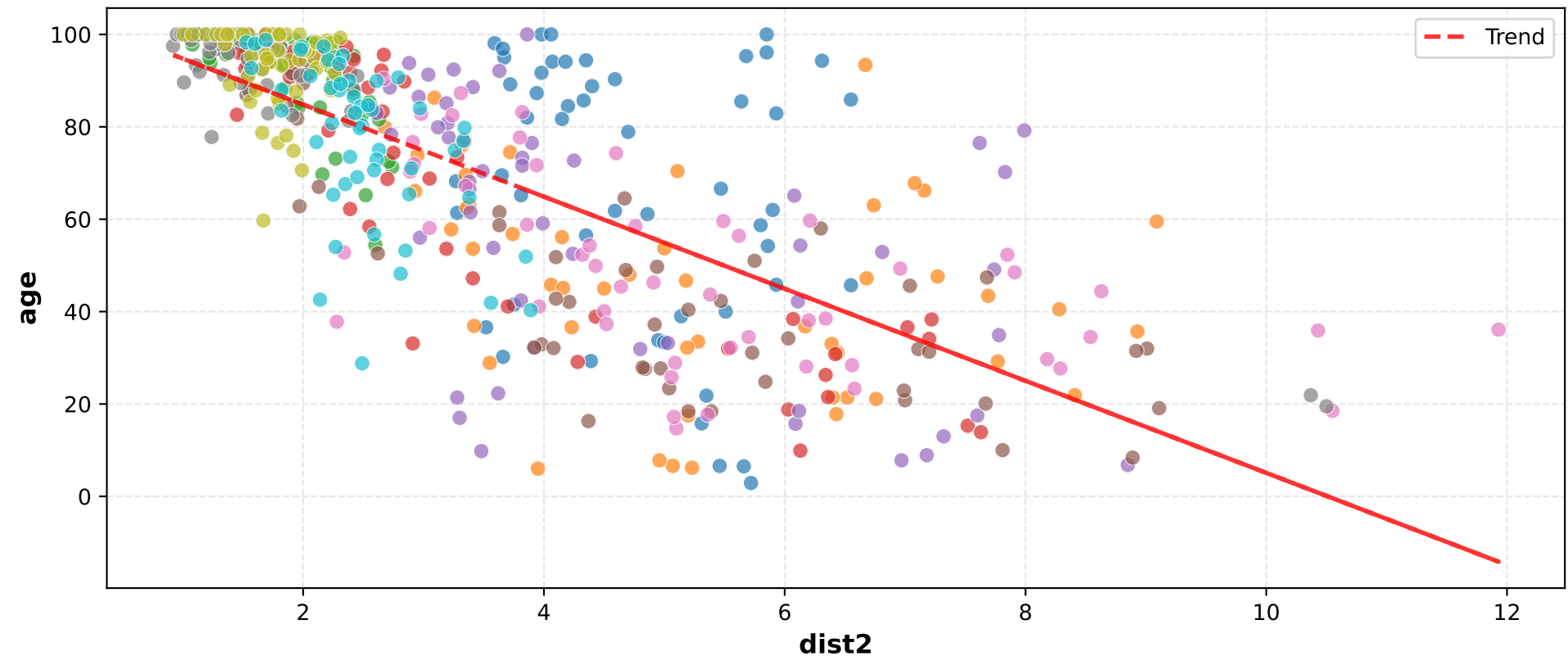
Scatter Plot
