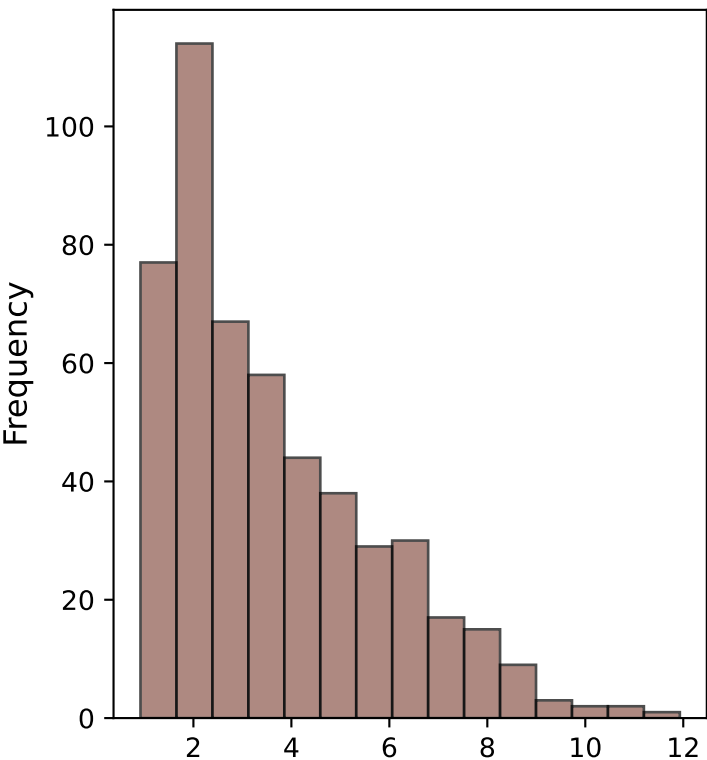
dist2 Distribution
