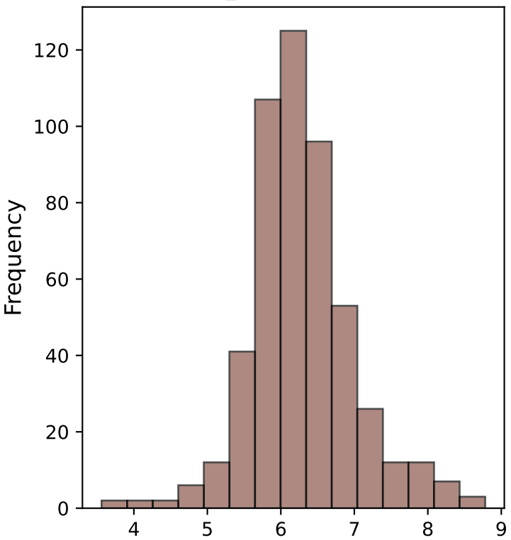
room_num Distribution
