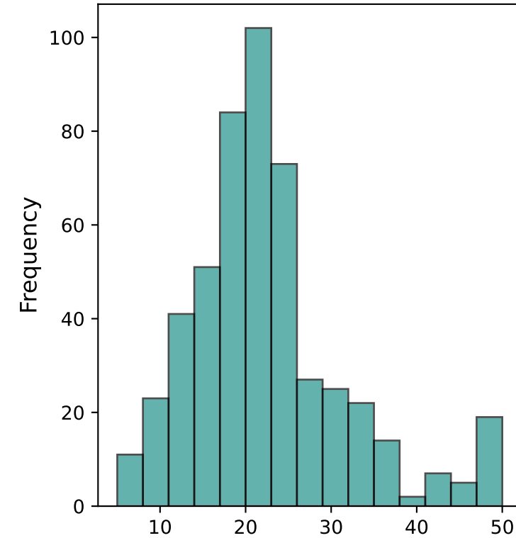
price Distribution
