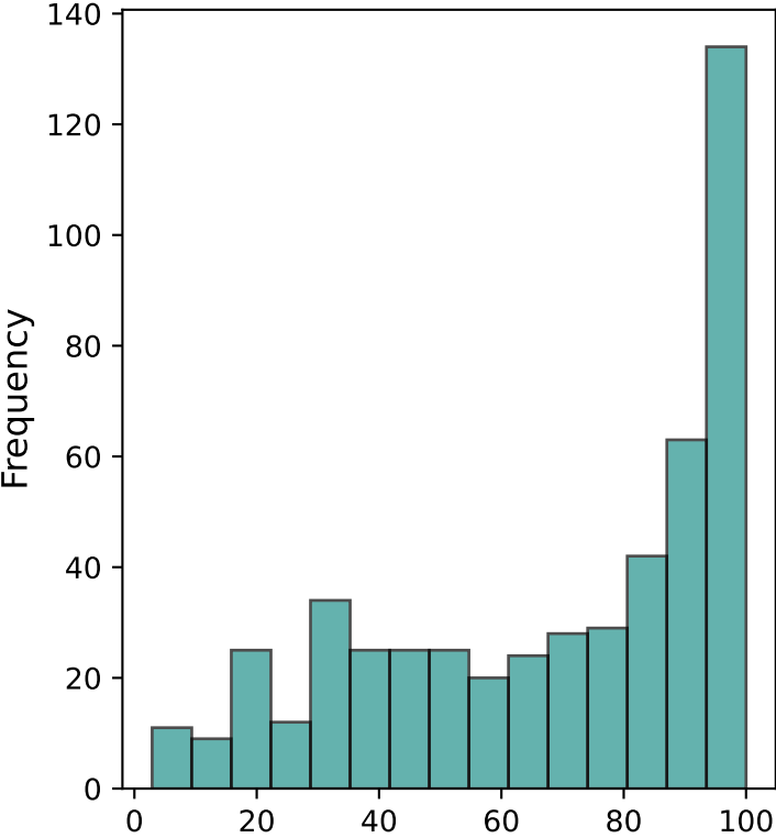
age Distribution
