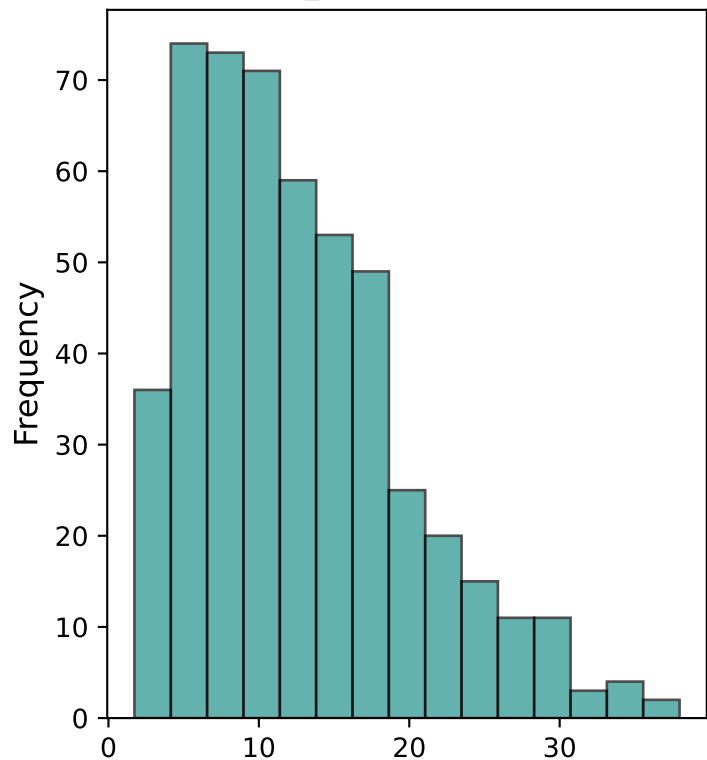
poor_prop Distribution
