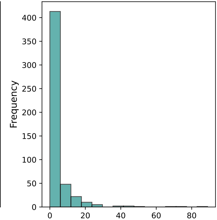
crime_rate Distribution
