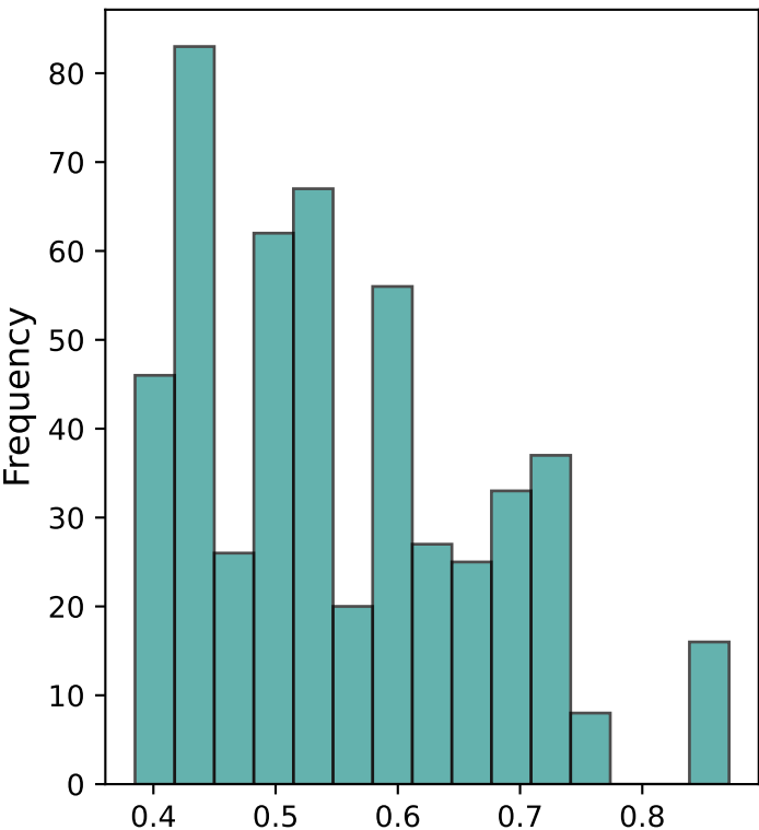
air_qual Distribution
