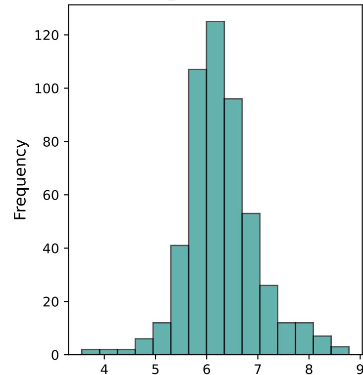
room_num Distribution
