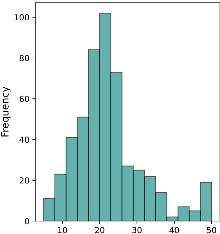
price Distribution
