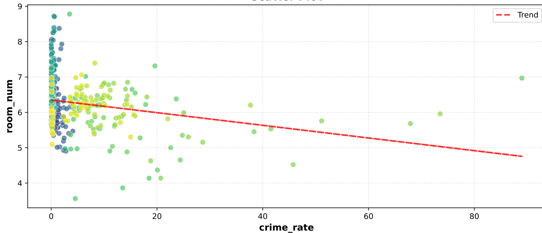
Scatter Plot
