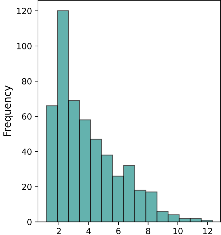
dist3 Distribution
