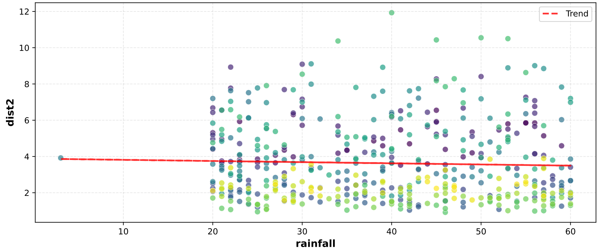
Scatter Plot
