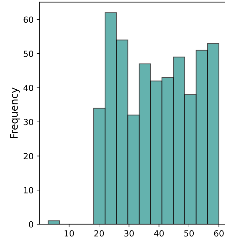
rainfall Distribution
