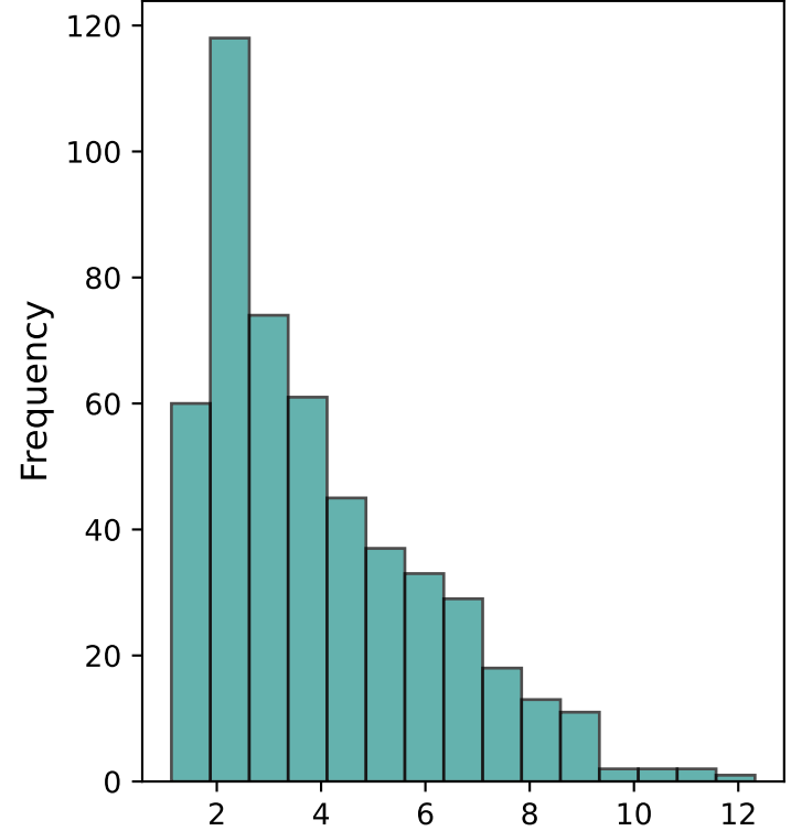
dist1 Distribution
