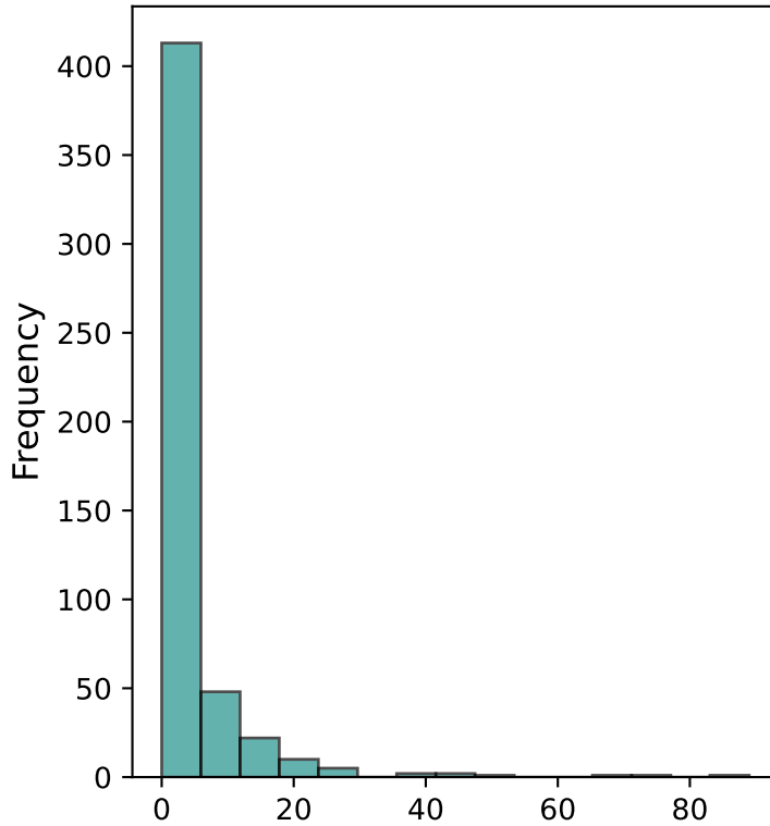
crime_rate Distribution
