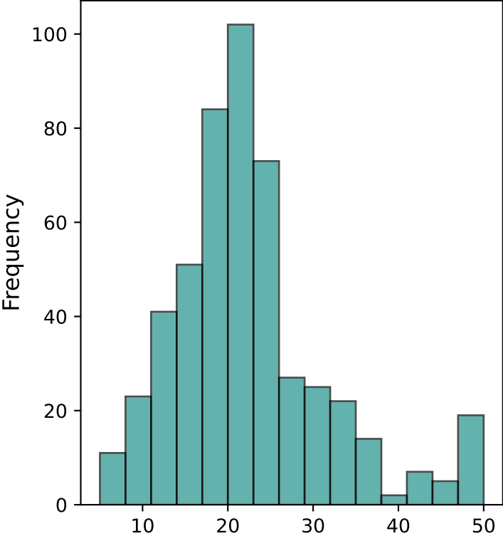
price Distribution
