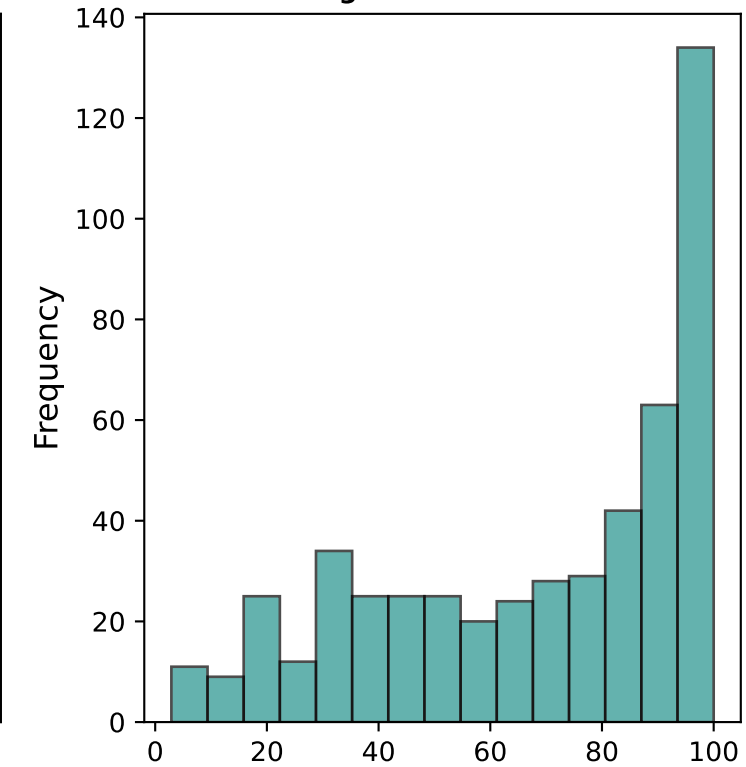
age Distribution
