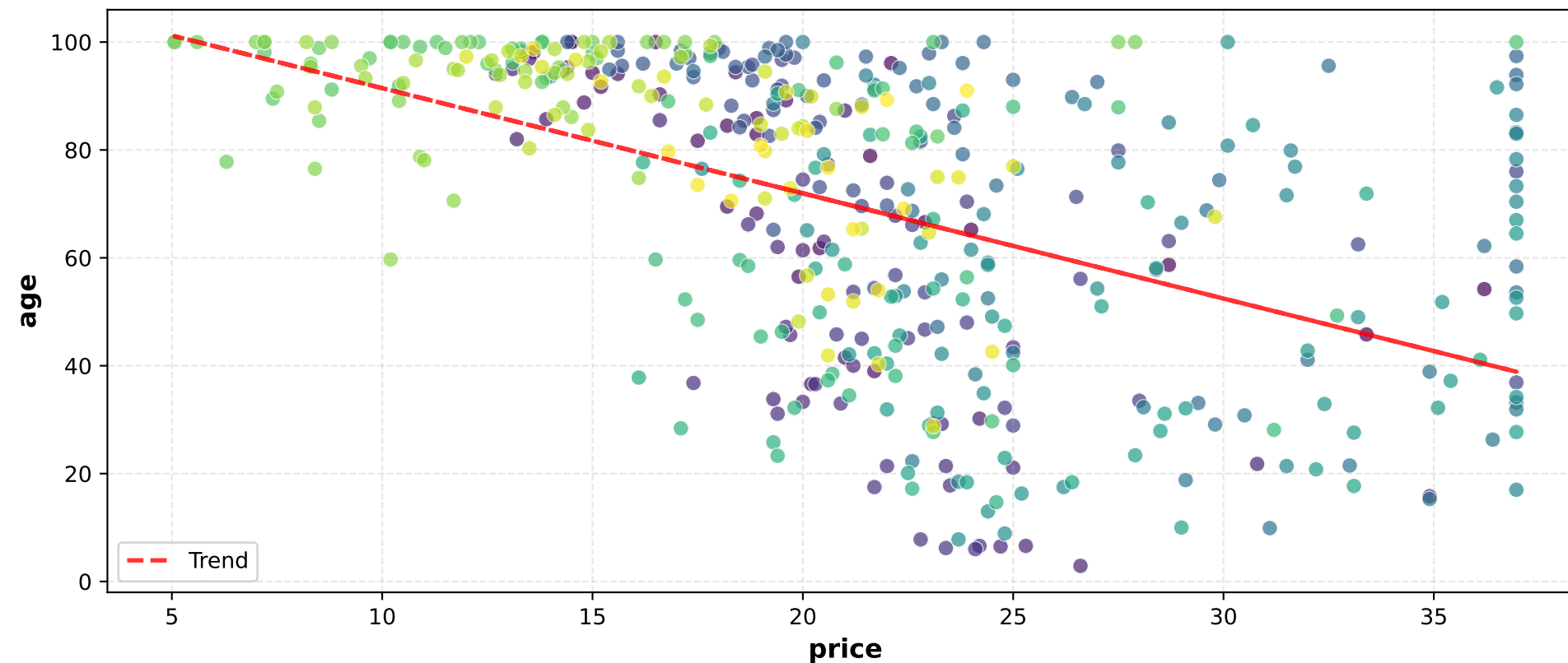
Scatter Plot
