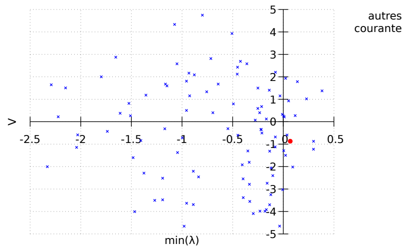
Scatter des solutions
