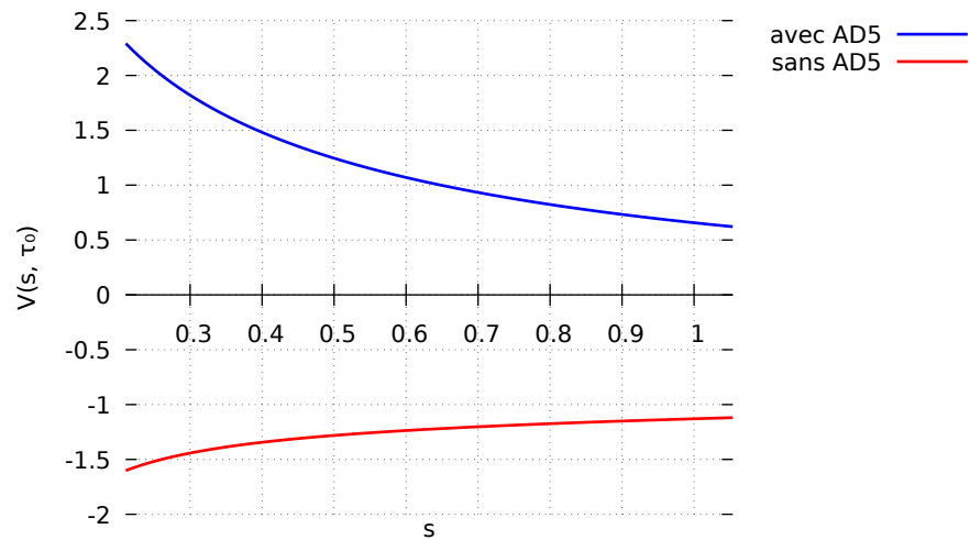
Scatter des solutions
