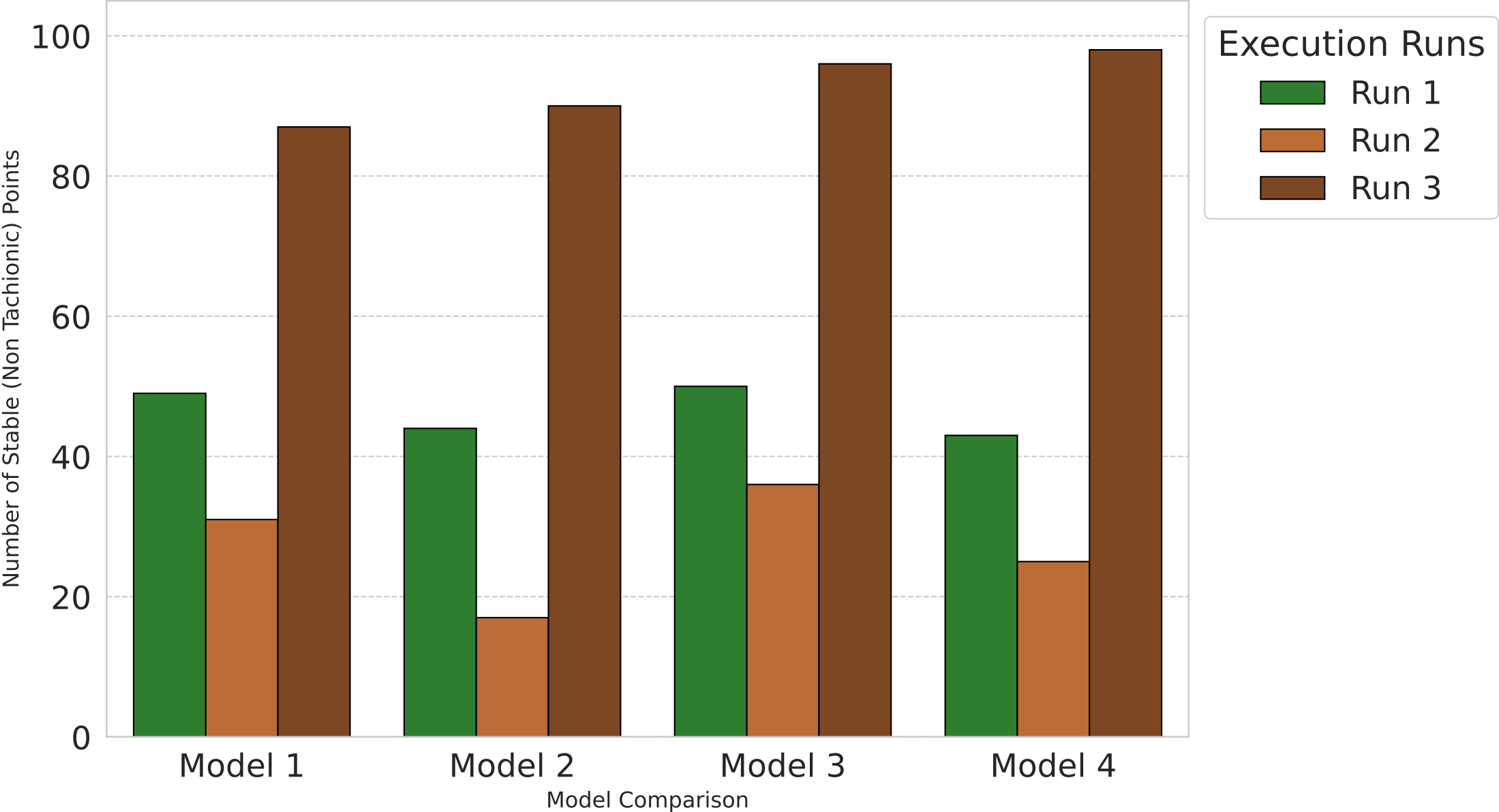
Stability Analysis: Count of Non-Tachyonic Vacua
