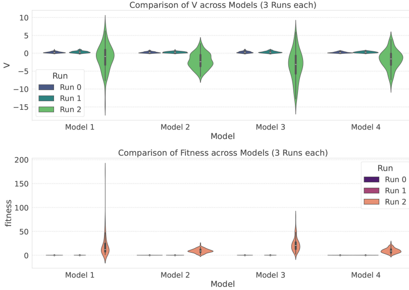
Fig. 8. Comparison of V (top) and fitness (bottom) across the four models. Each model is shown with its three independent runs.
