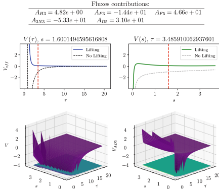
Fig. 5. Lifting acting primarily on the dilaton s .
