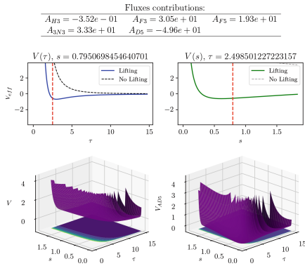
Fig. 6. Lowering of the potential along the moduli directions after lifting, leading to negative regions or flattening.
