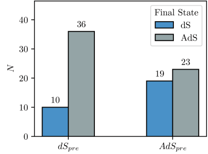
Fig. 2. Transition between vacuum types (original database).
