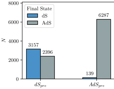
Fig. 1. Transition between vacuum types (new solutions).
