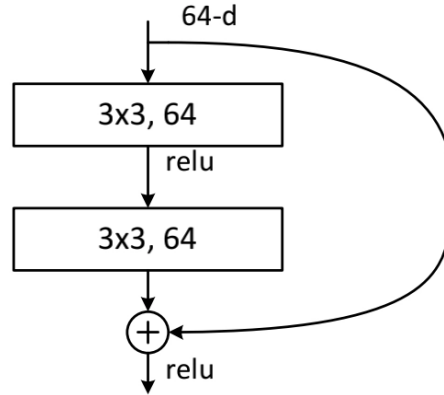
Figure 1: Resnet
