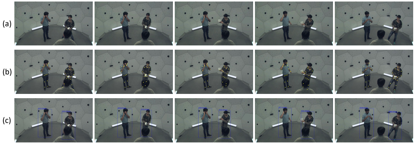
Figure 6: Visualizations of (a) the original video frames, (b) the predicted 2D joint maps, and (c) the output 2D box maps of CPP, respectively.
