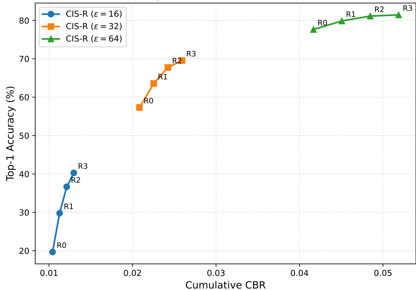
Accuracy-CBR Trade-off under Different \varepsilon
