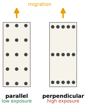
a Array geometry sets exposure
