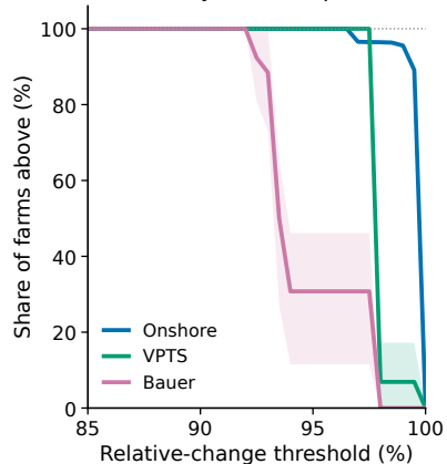
Universality (bootstrap 95% CI)
