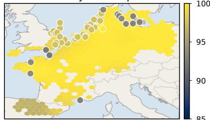
Sensitivity across space
