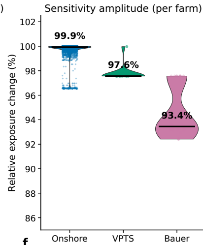
Mechanism: concentration \Rightarrow sensitivity
