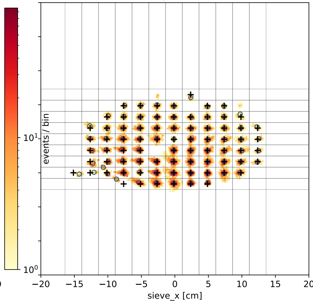
Foil 1 (y tar =0 cm)
