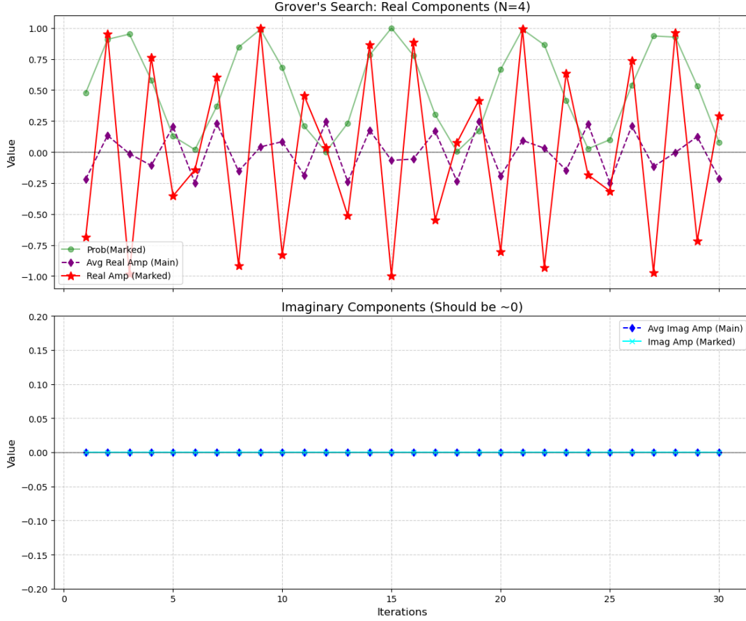
Figure 3: Probability of measuring the marked state and the corresponding real amplitudes over multiple Grover iterations.
