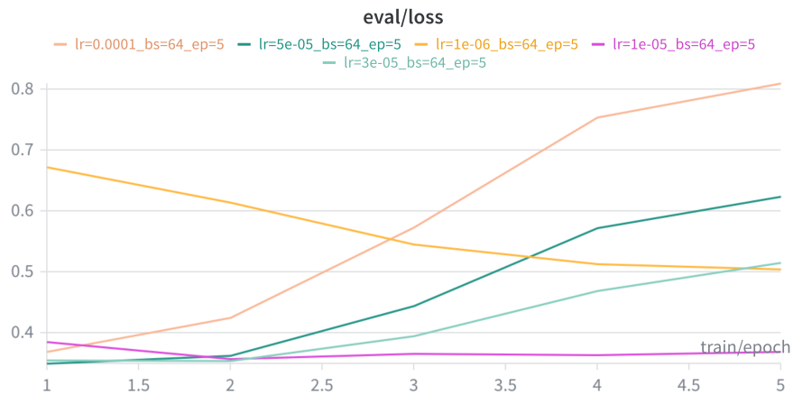
Figure 2: Loss across different learning rates
