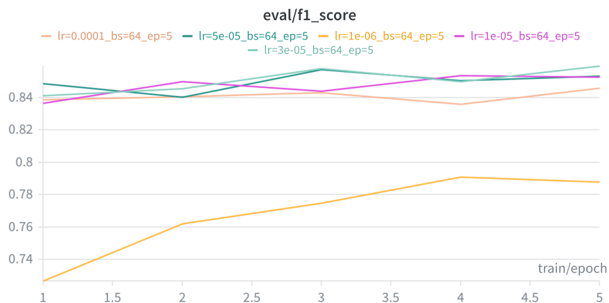
Figure 1: F1-score across different learning rates
