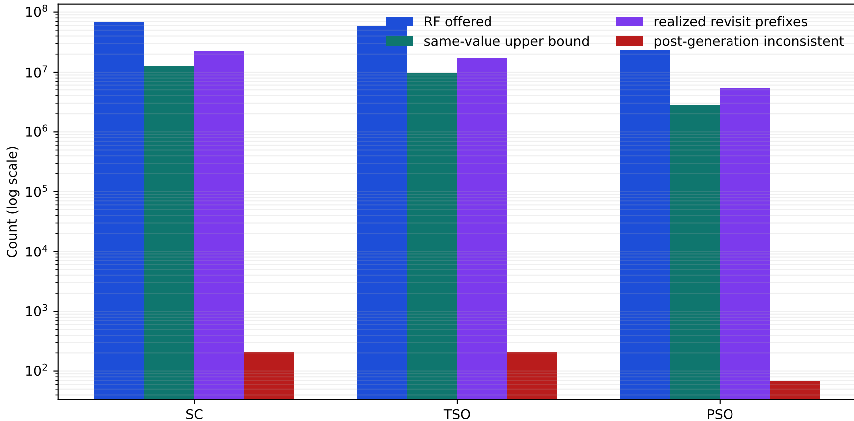
725-task search funnel: opportunity exists before candidate generation
