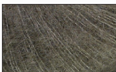
8003 MUDDIE
