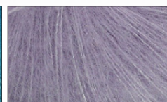
8006 LILAC MIST
