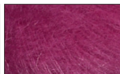
8021 FUCHSIA FLURRY
