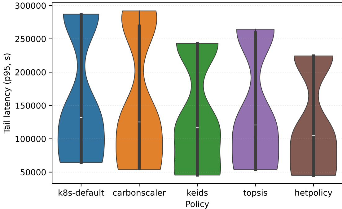
SIM tail latency distribution
