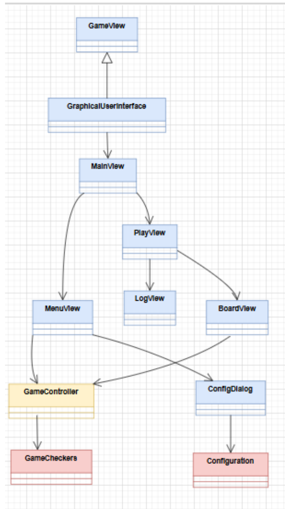
FIGURE 16 – Architecture interne de la GUI.
