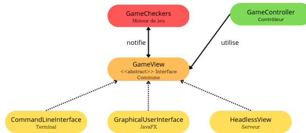
FIGURE 19 – Architecture des modules Model-View
