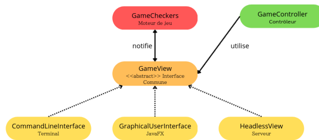
FIGURE 16 – Architecture des modules Model-View
