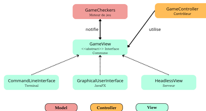
FIGURE 15 – Architecture des modules Model-View
