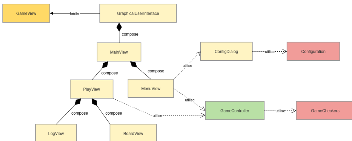
FIGURE 16 – Architecture interne de la GUI.
