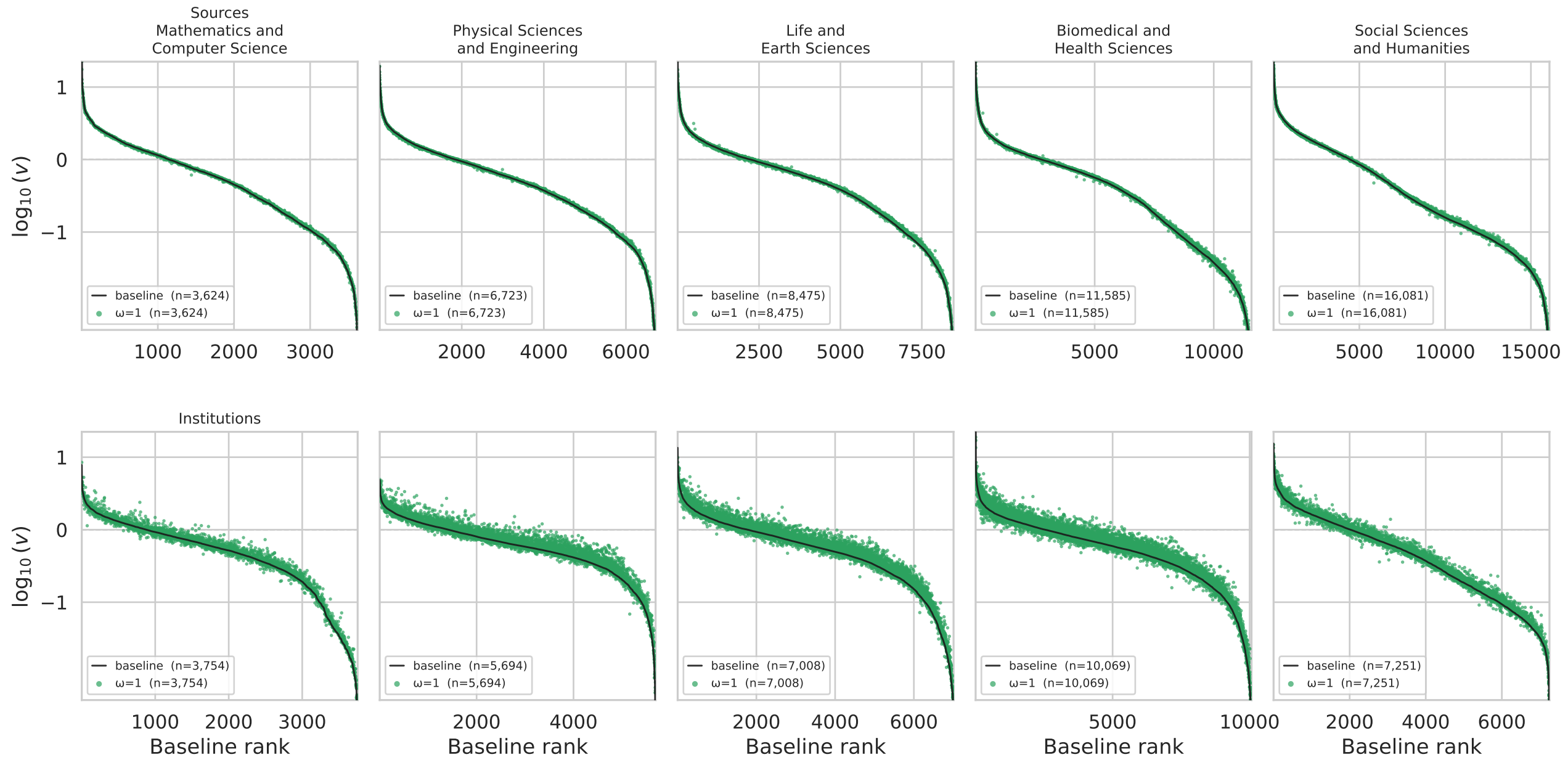
Spectral ranking: baseline vs \omega=1 (window 2020_2024)
