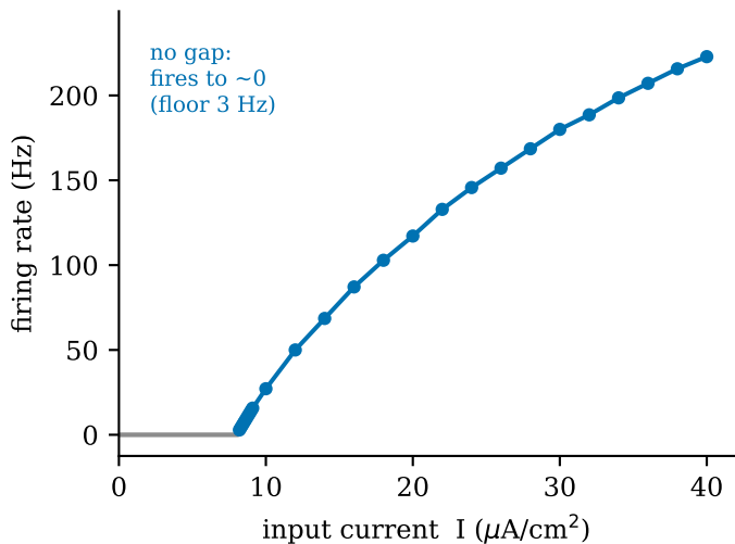
C Connor-Stevens (Type-I)
