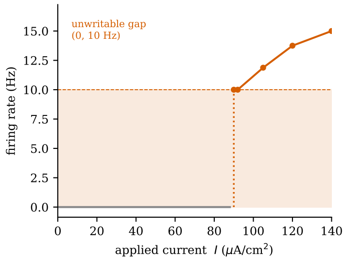
A Morris-Lecar, Hopf regime (Type-II)
