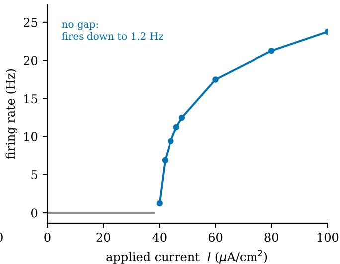
B Morris-Lecar, SNIC regime (Type-I)
