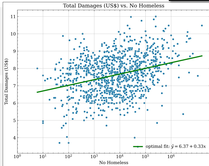
Figure 3.2: ols fit
