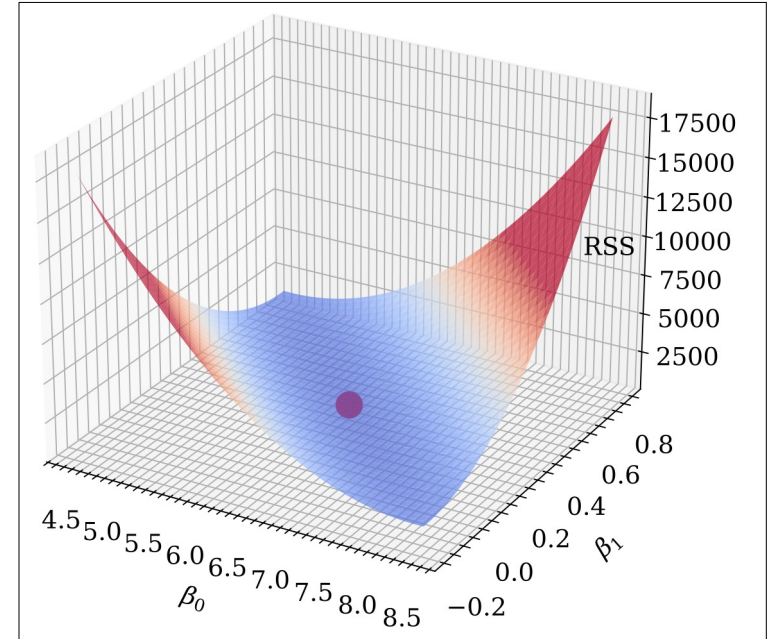
Figure 3.3: Residual sum squared loss surface
