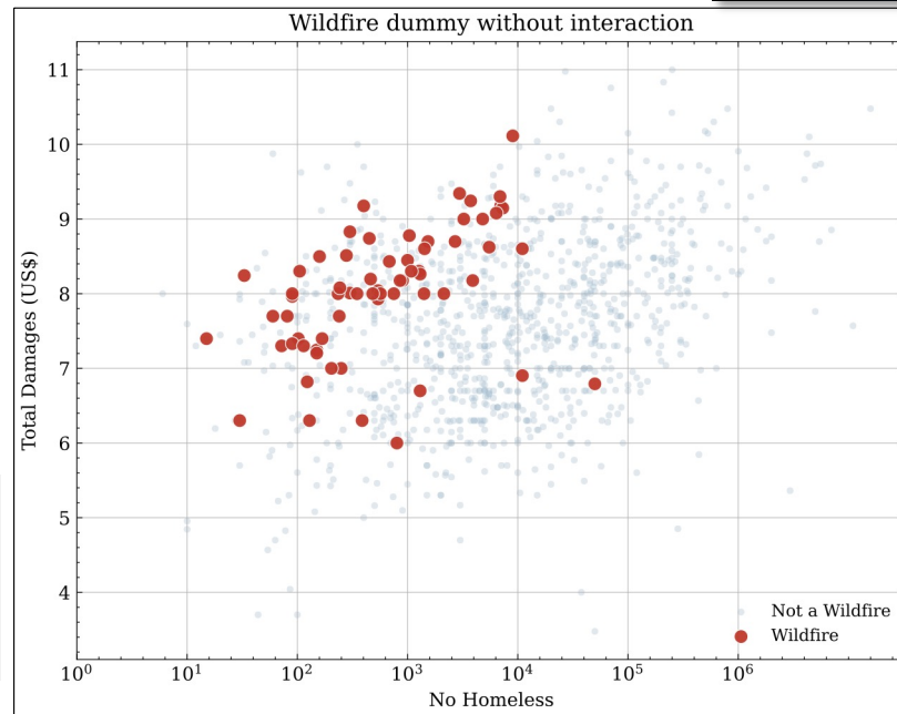
Figure 3.6: dummy variables
