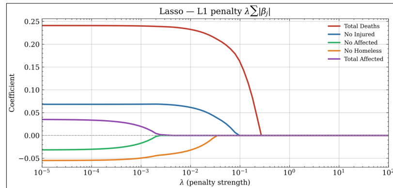
Figure 3.9: lasso
