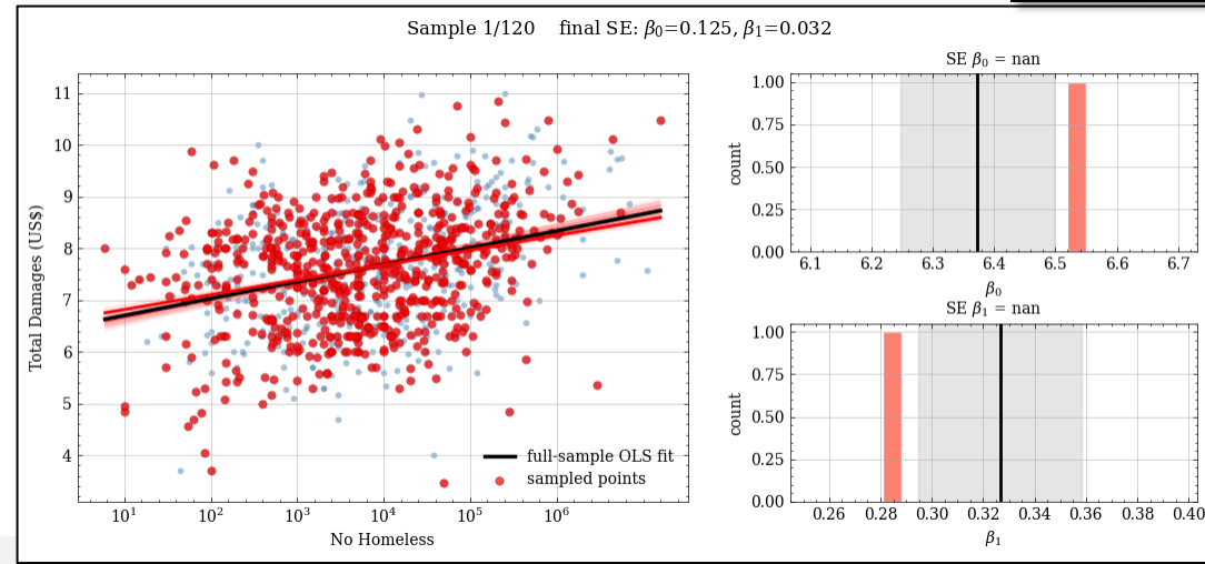
Figure 3.4: standard error
