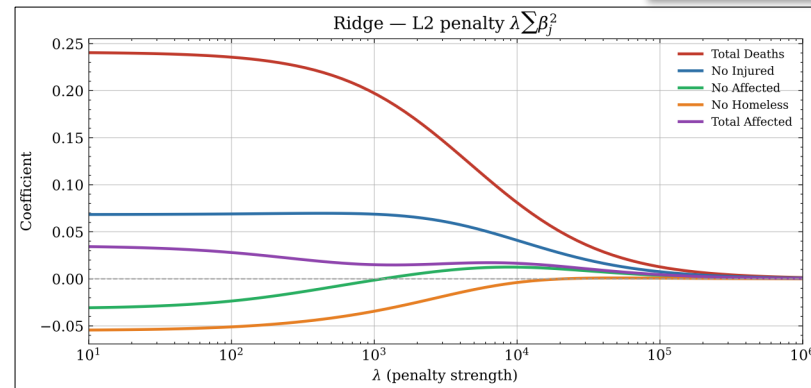
Figure 3.8: ridge
