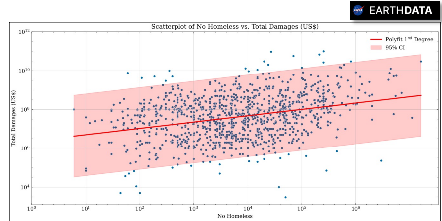
Figure 3.5: confidence band
