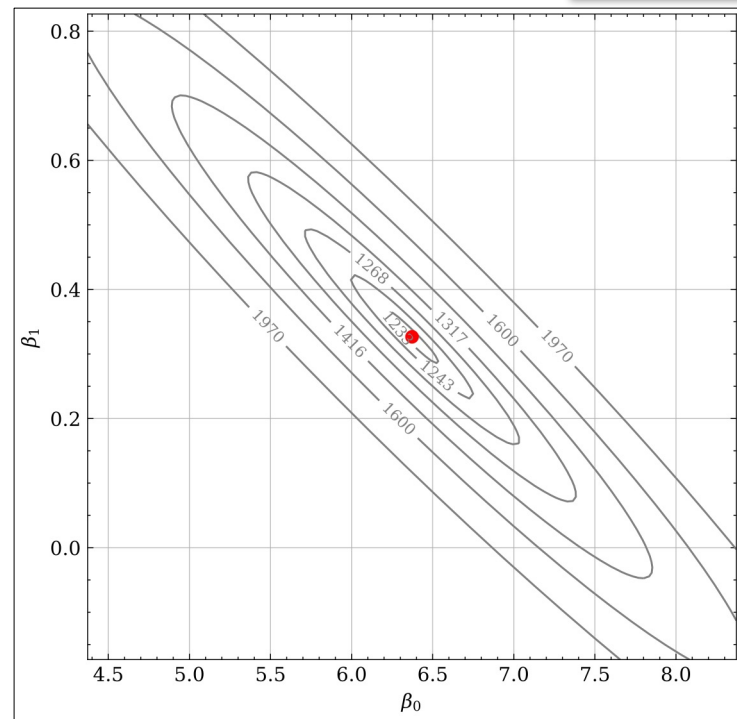
Figure 3.3: rss surface
