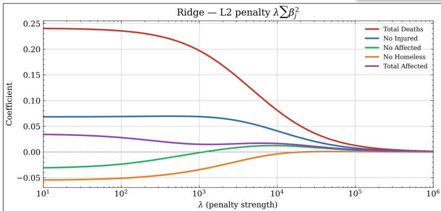
Figure 3.8: ridge
