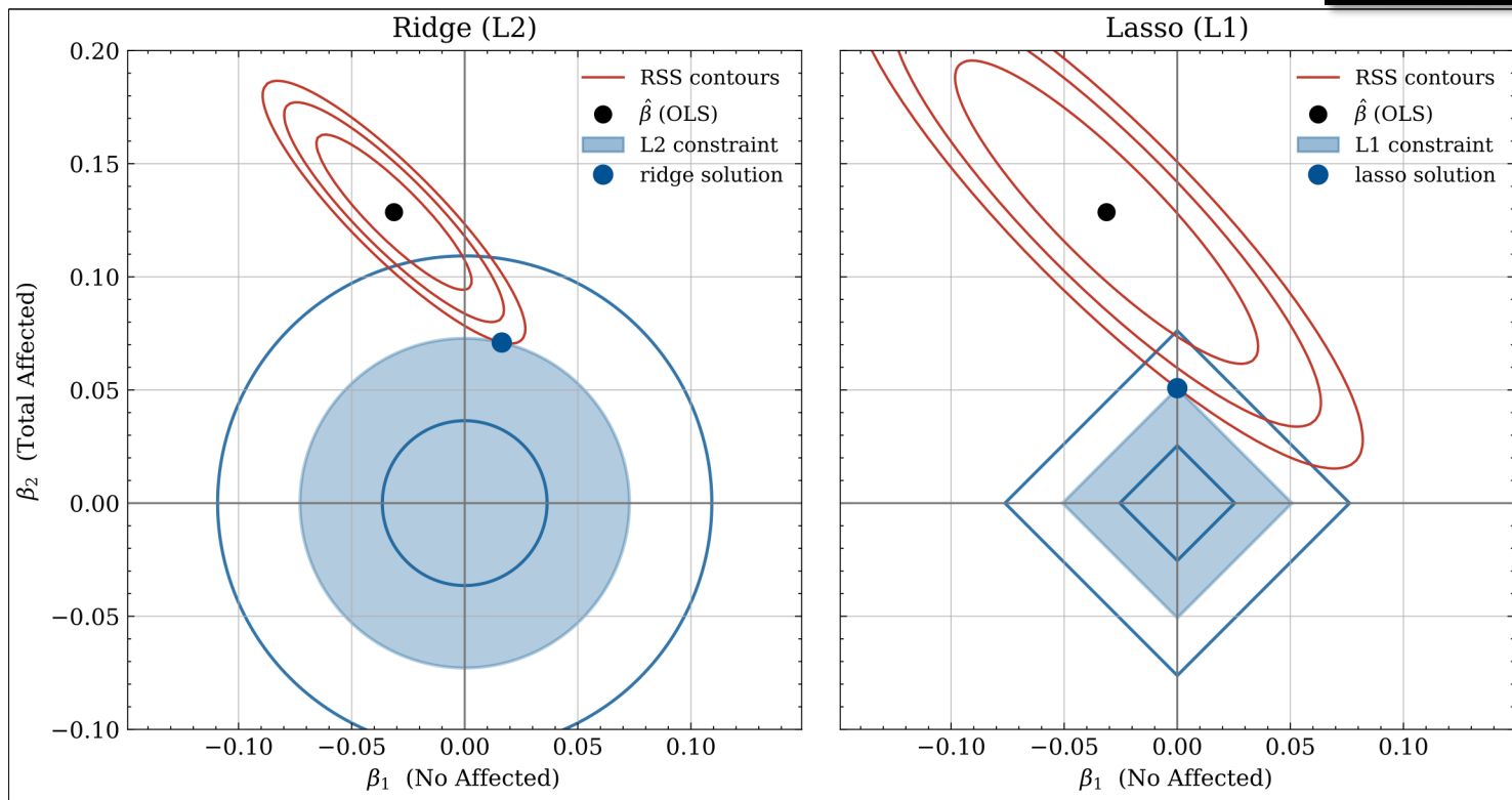
Figure 3.10: constraint geometry
