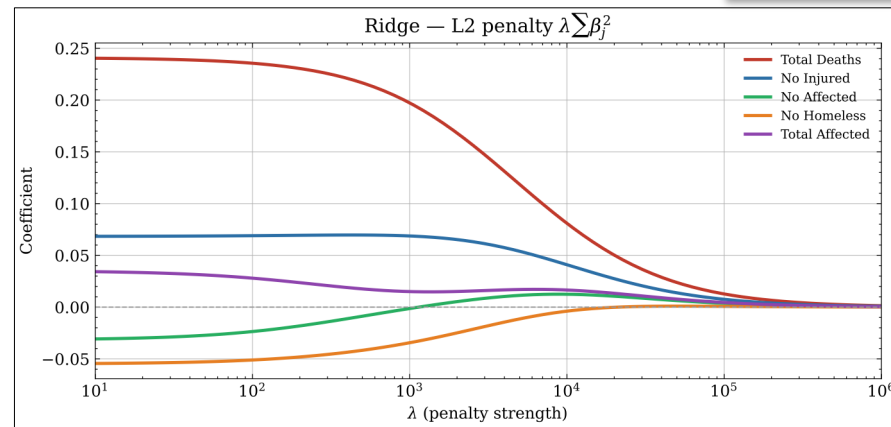
Figure 3.8: ridge
