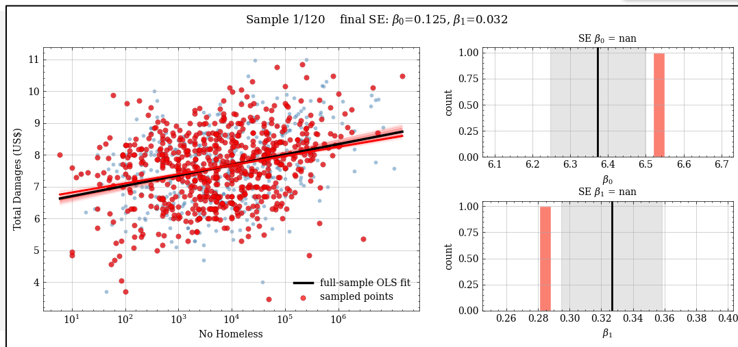
Figure 3.4: standard error
