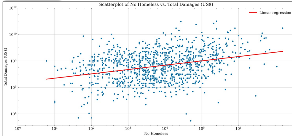
Figure 3.1: line plus noise
