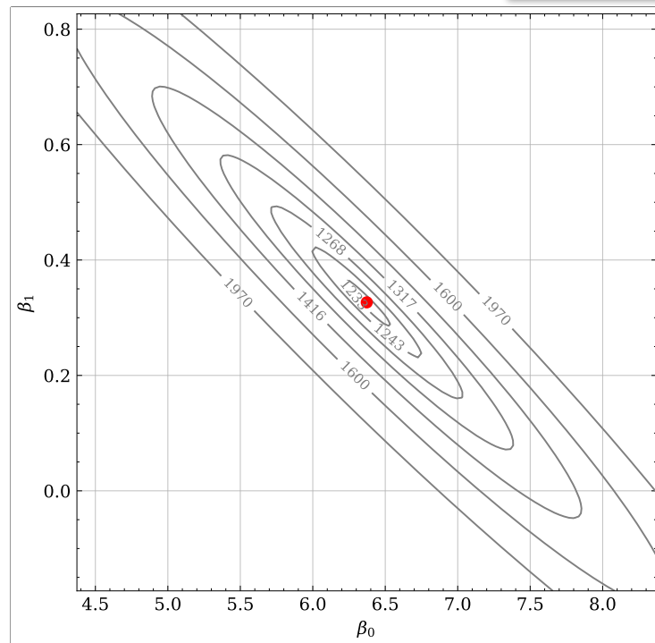
Figure 3.3:rss surface
