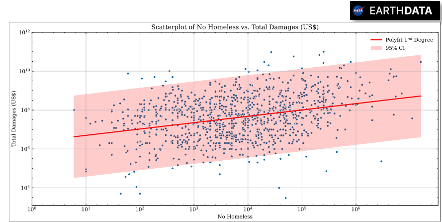
Figure 3.5: confidence band
