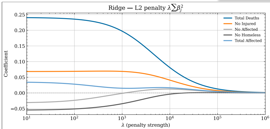
Figure 3.8: ridge
