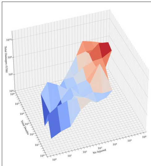
High bias
