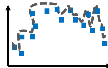
High variance
