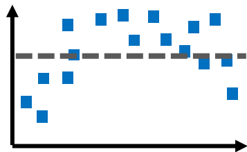
High bias
