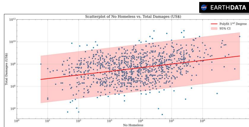
Figure 3.5: confidence band
