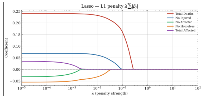
Figure 3.9: lasso
