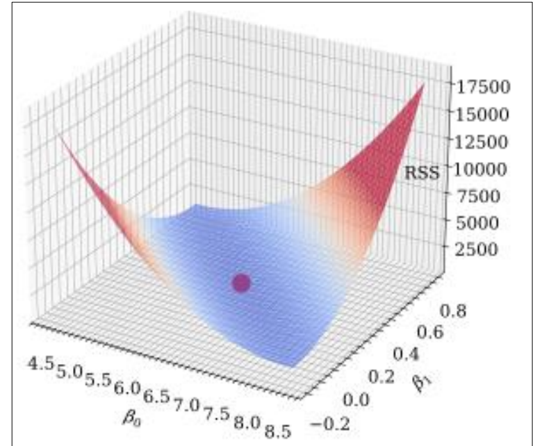
Figure 3.3: Residual sum squared loss surface
