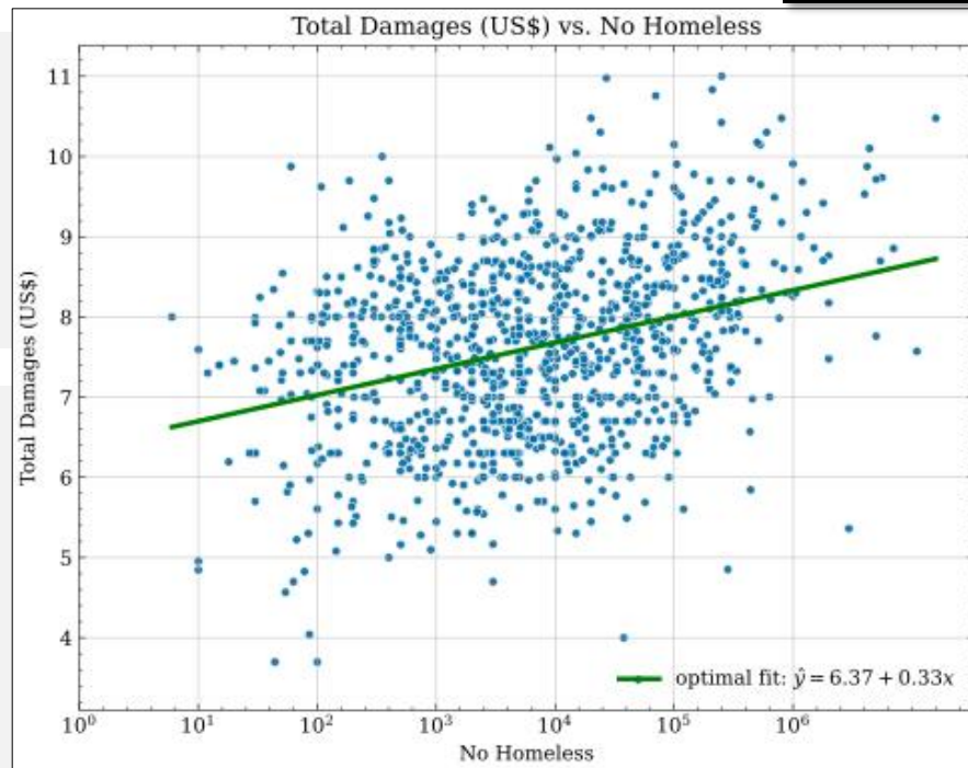
Figure 3.2: ols fit
