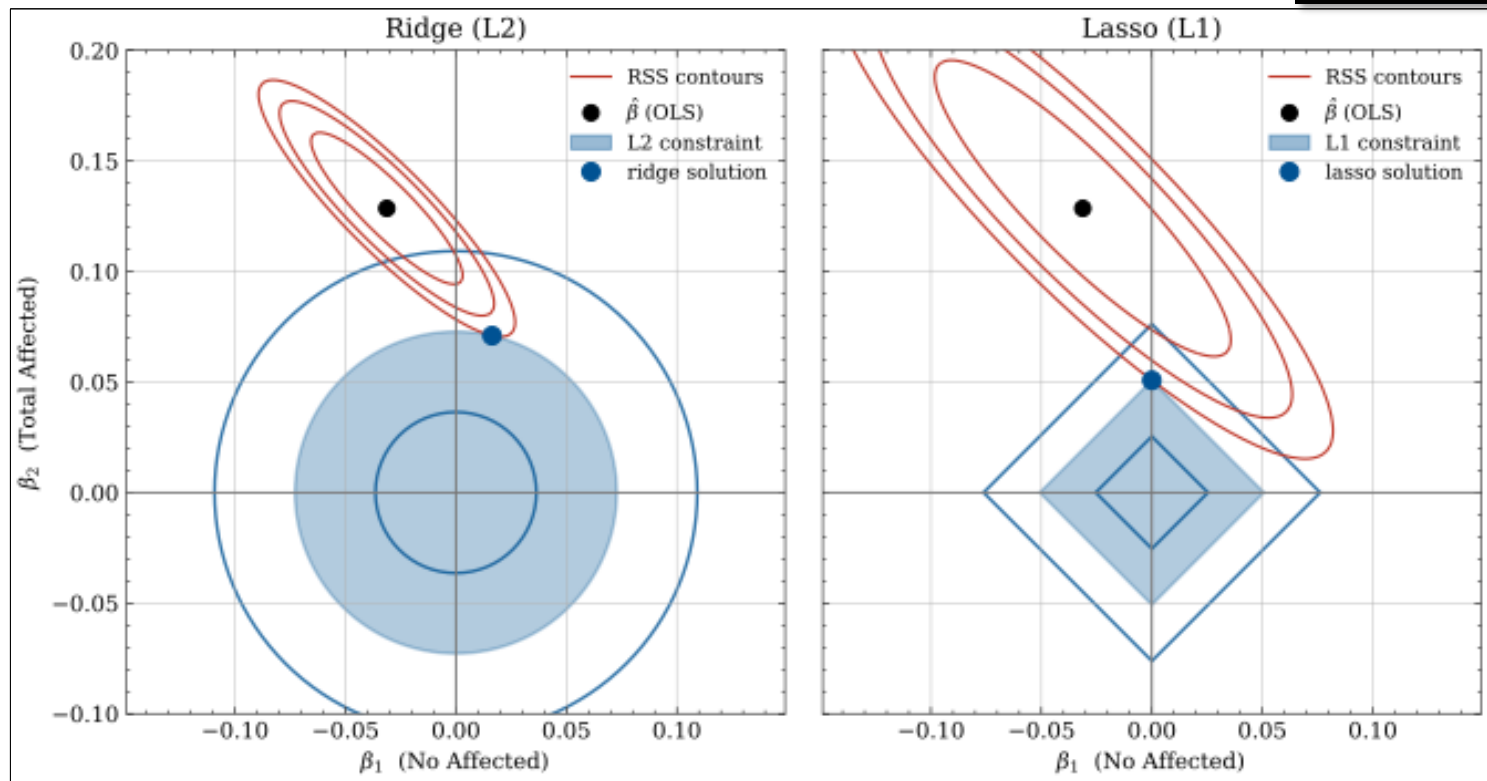
Figure 3.10: constraint geometry
