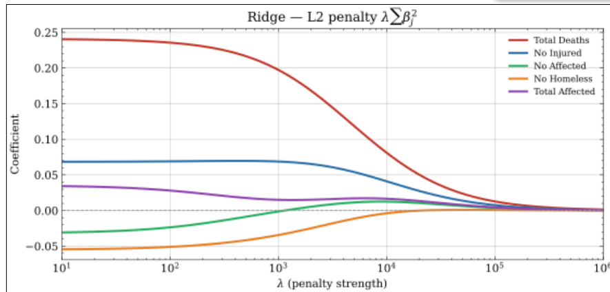
Figure 3.8: ridge
