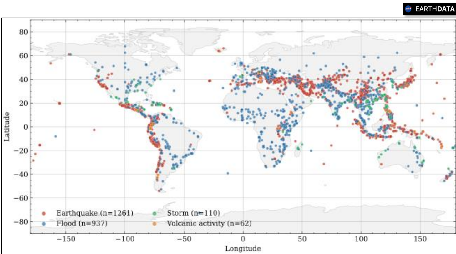
Figure 5.1: regions motivation
