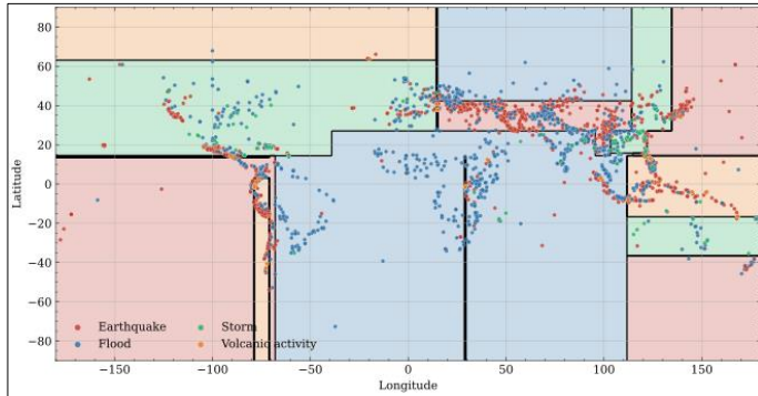
Figure 5.2: treeregions
