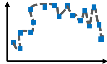
High variance
