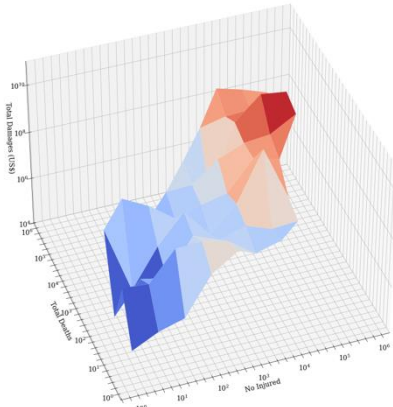
High bias
