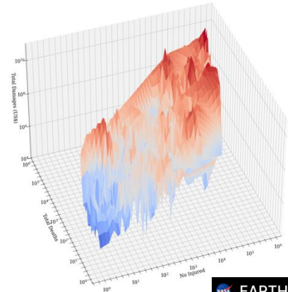
High variance
