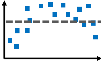
High bias
