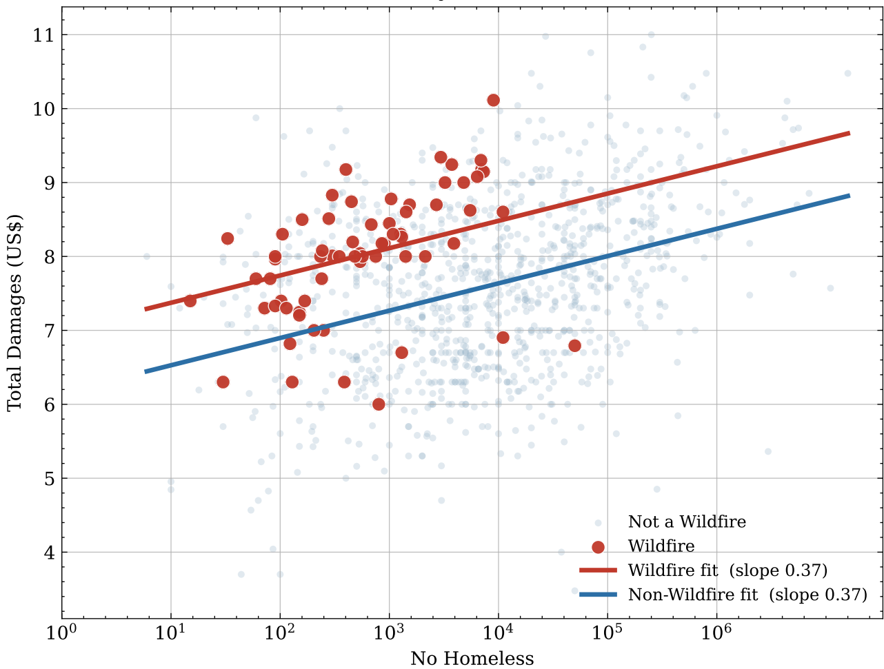
Wildfire dummy without interaction
