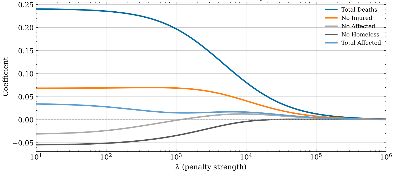
Ridge — L2 penalty \lambda \sum \beta_j^2
