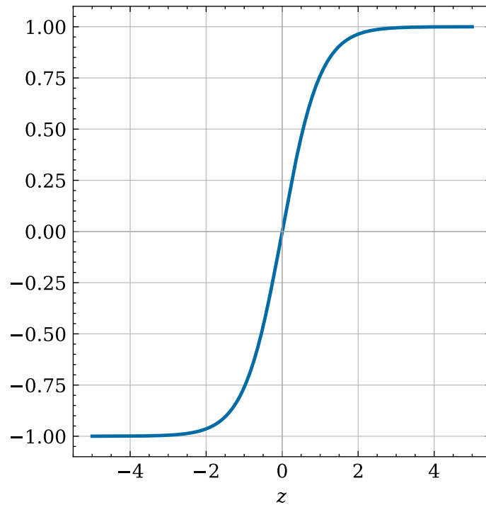
Hyperbolic tangent
