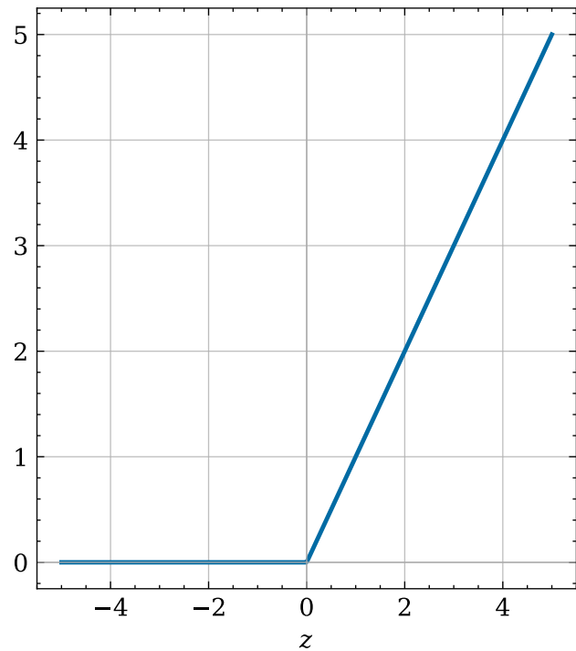
ReLU
