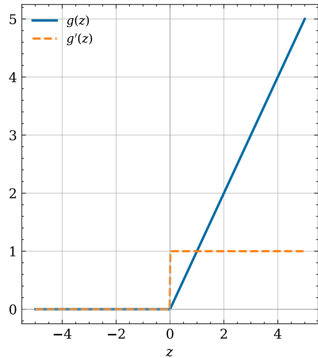
ReLU
