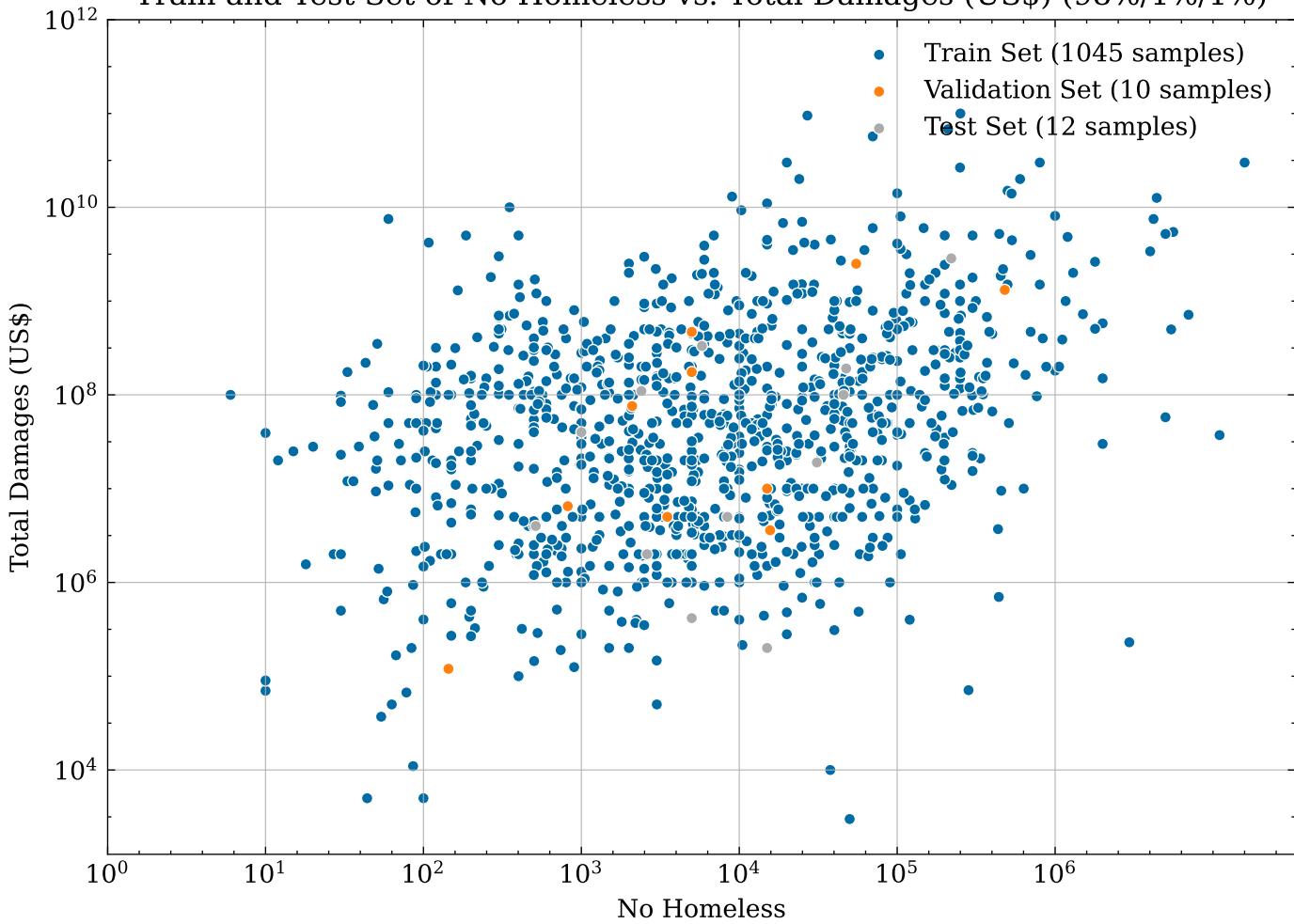
Train and Test Set of No Homeless vs. Total Damages (US$) (98%/1%/1%)
