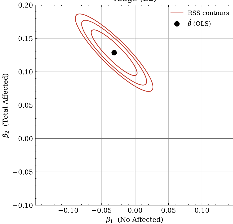
Ridge (L2)
