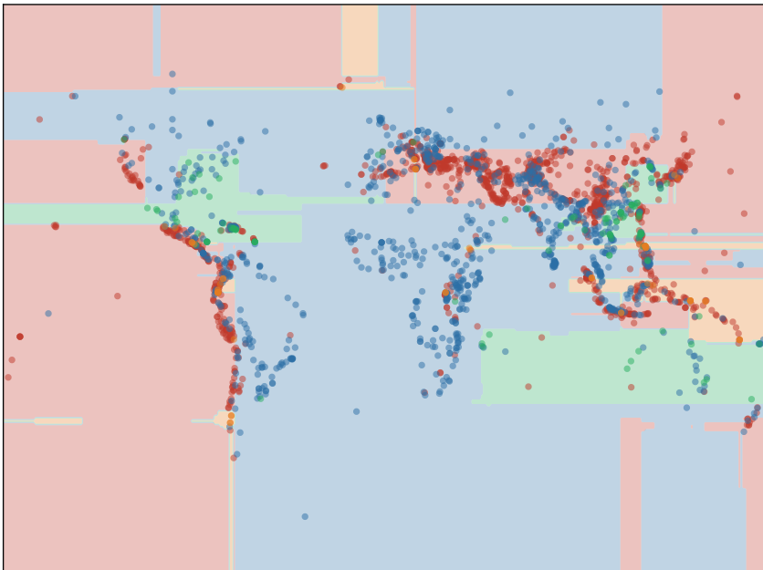
bagged ensemble — 200 trees
