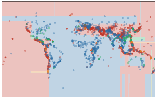
after 200 trees
