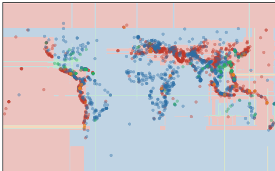
after 50 trees
