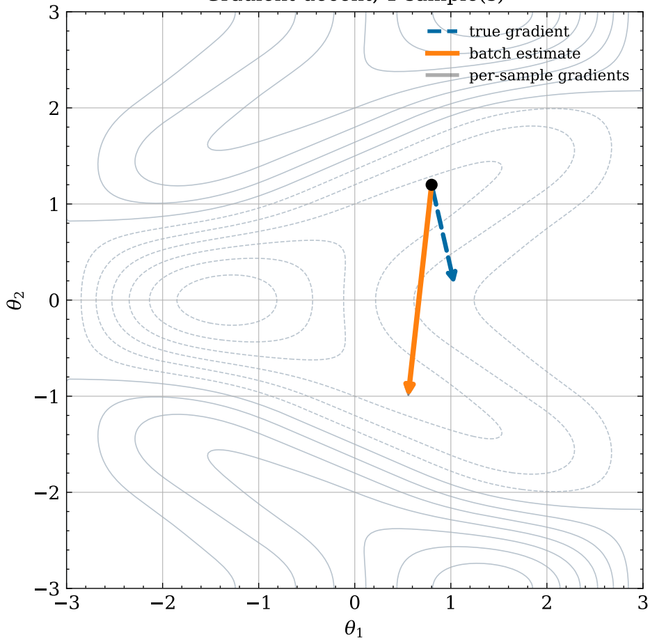
Gradient decent, 1 sample(s)
