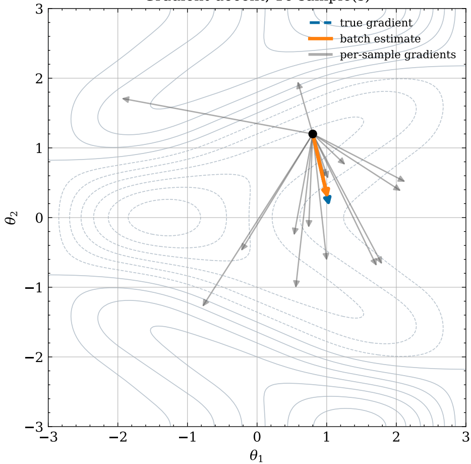
Gradient decent, 16 sample(s)
