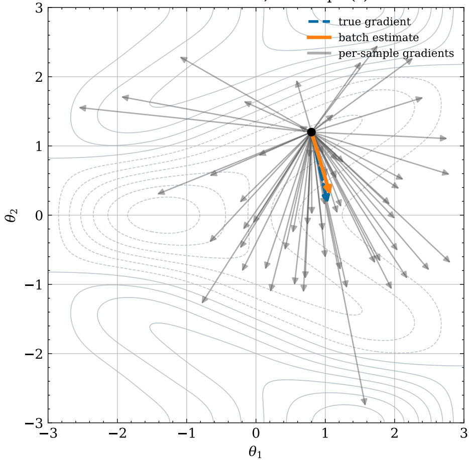
Gradient decent, 64 sample(s)
