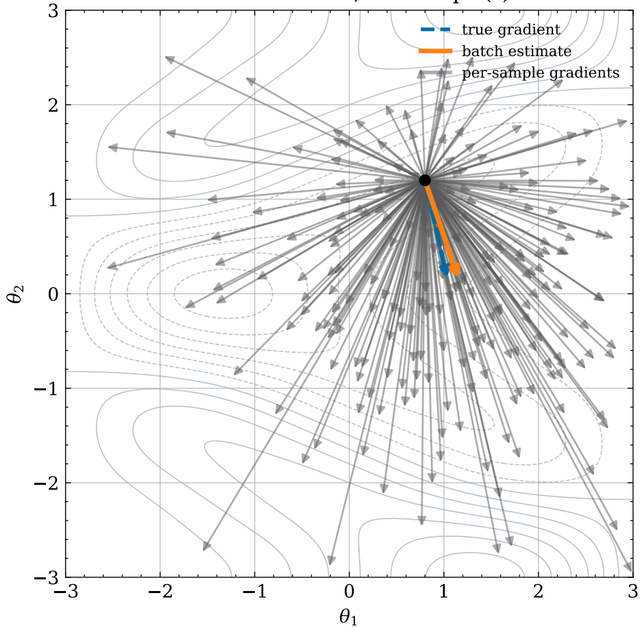
Gradient decent, 256 sample(s)
