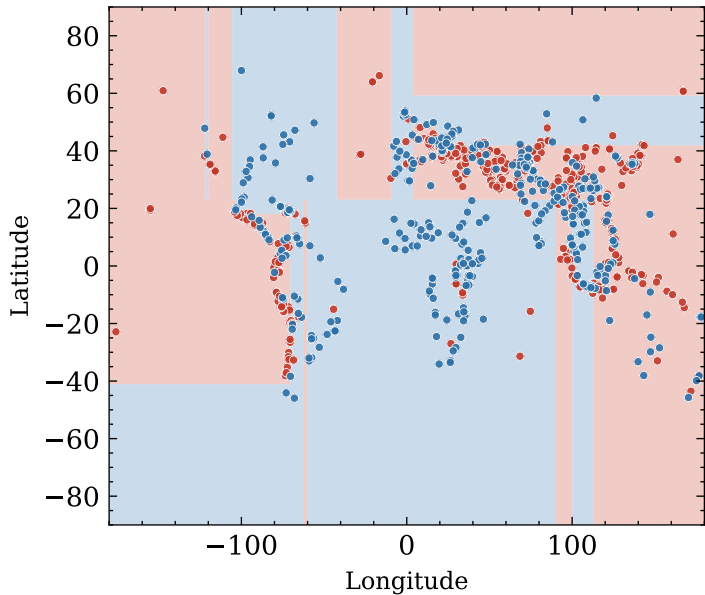
Decision tree (depth 5)
