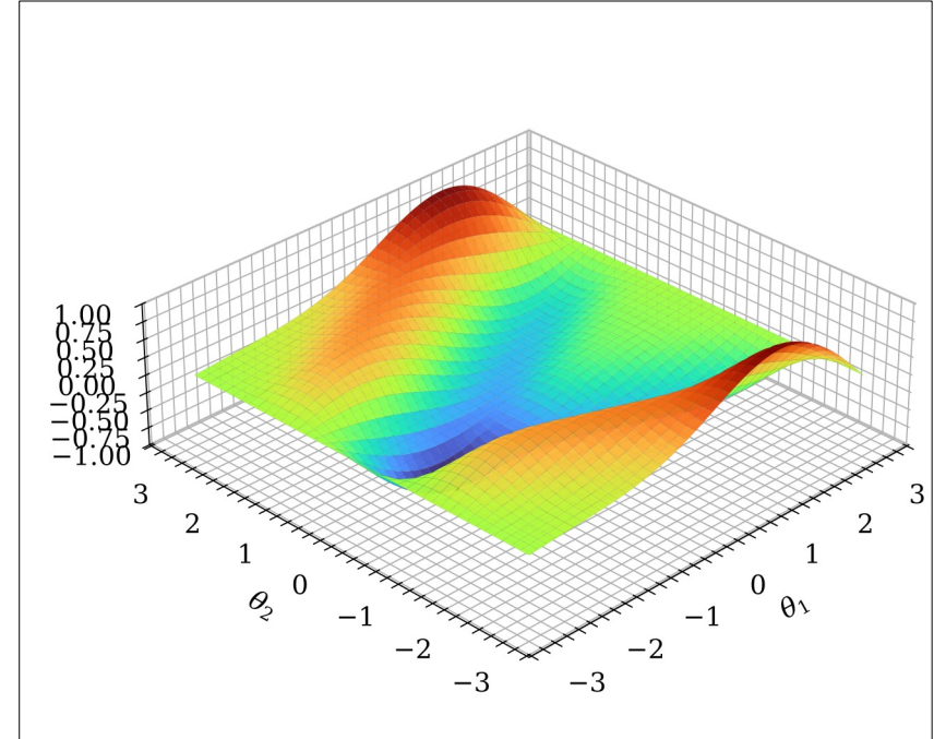
Figure 6.7: loss surface
