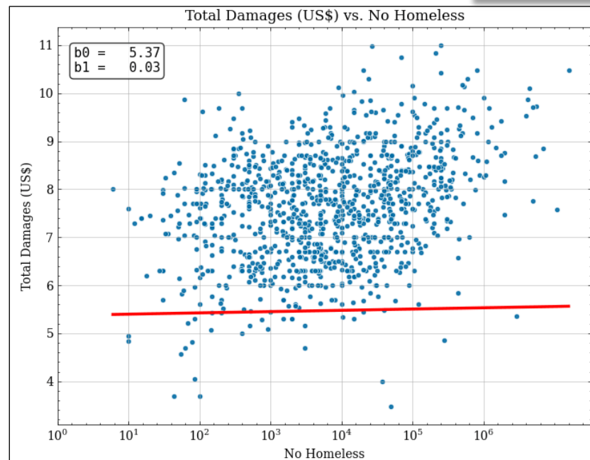
Figure 3.2: ols fit
