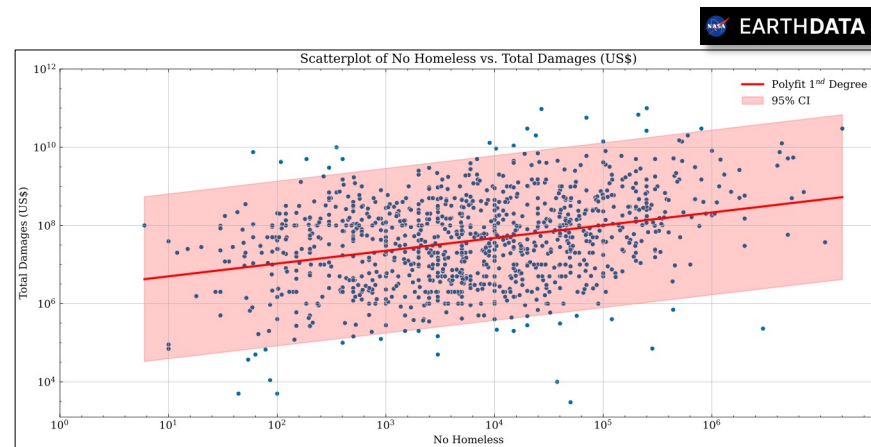
Figure 3.5: confidence band
