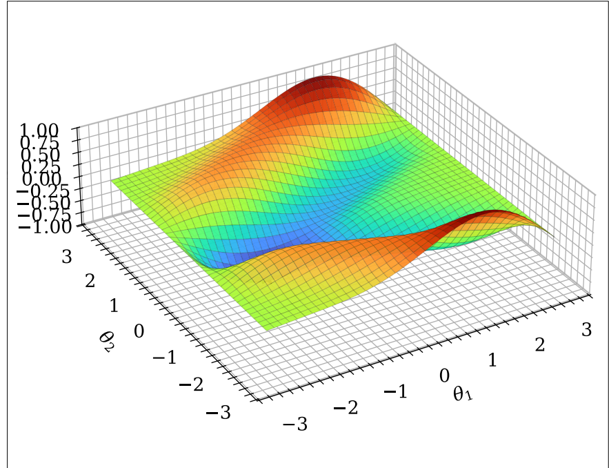
Figure 6.7: loss surface
