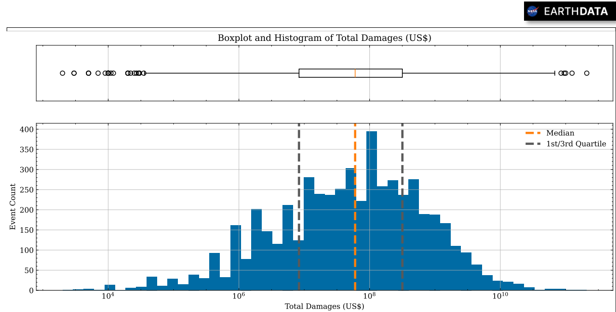
Figure 1.5: boxplot dispersion
